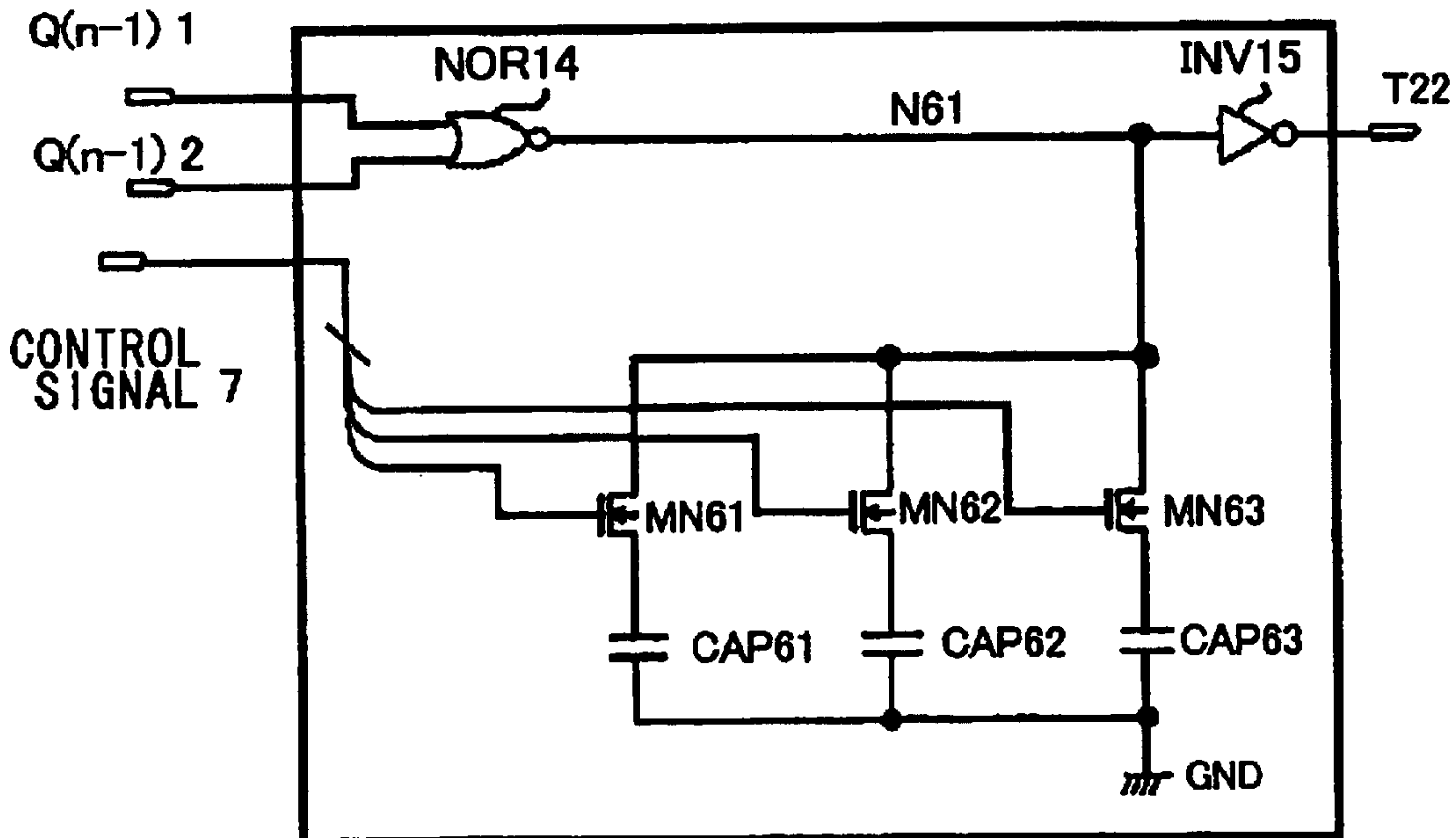
TIMING DIFFERENCE DIVIDING CIRCUITS 209
