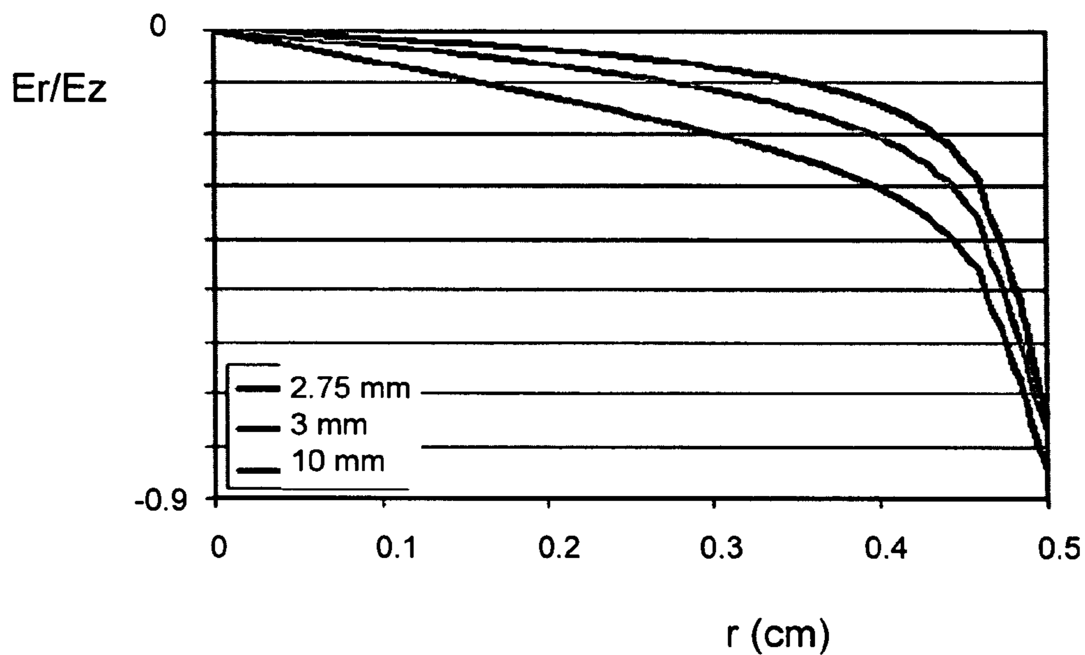
NORMALIZED FOCUSING FIELD AT CATHODE SURFACE
