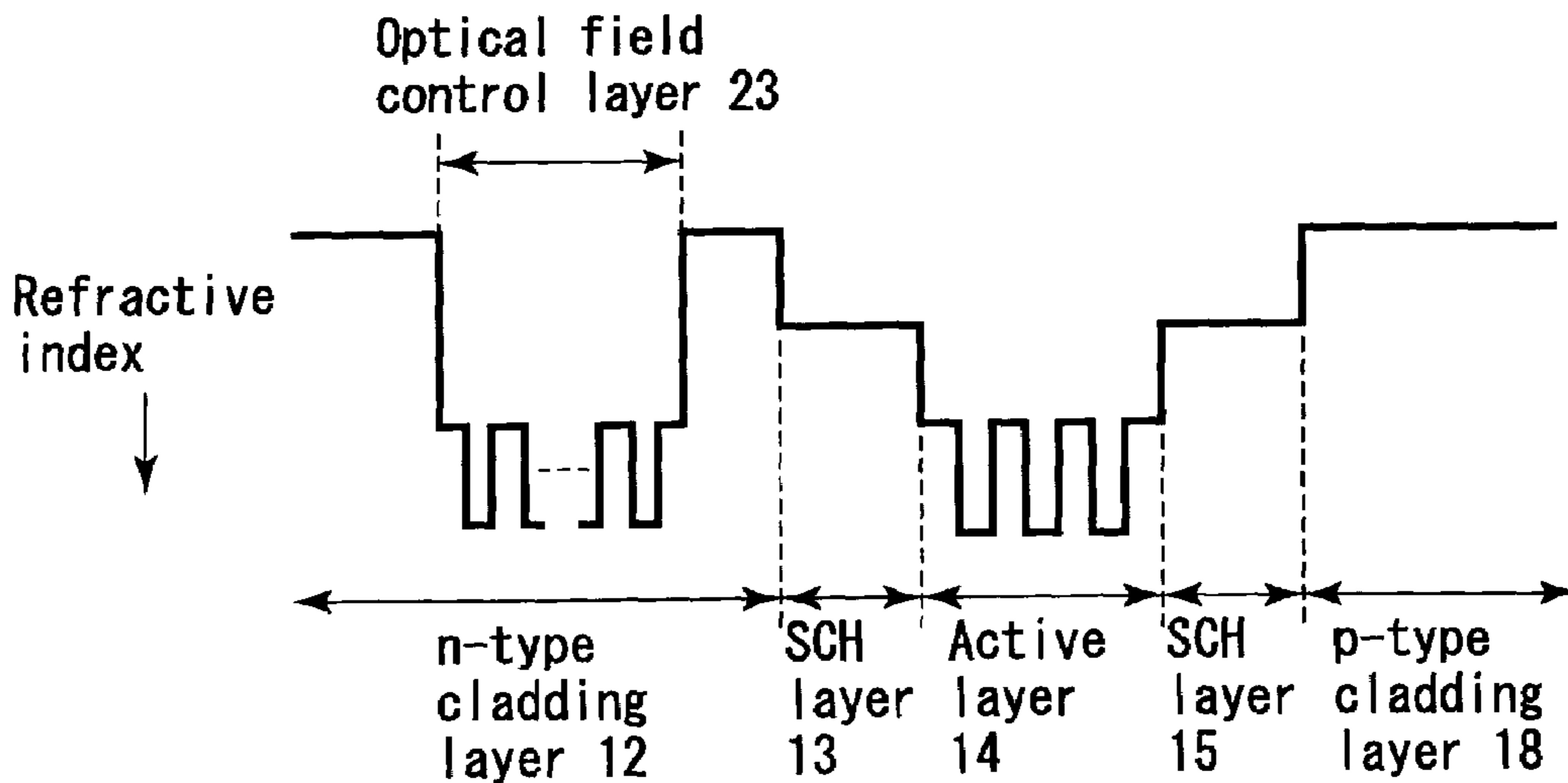
FIG. 15 (PRIOR ART)
