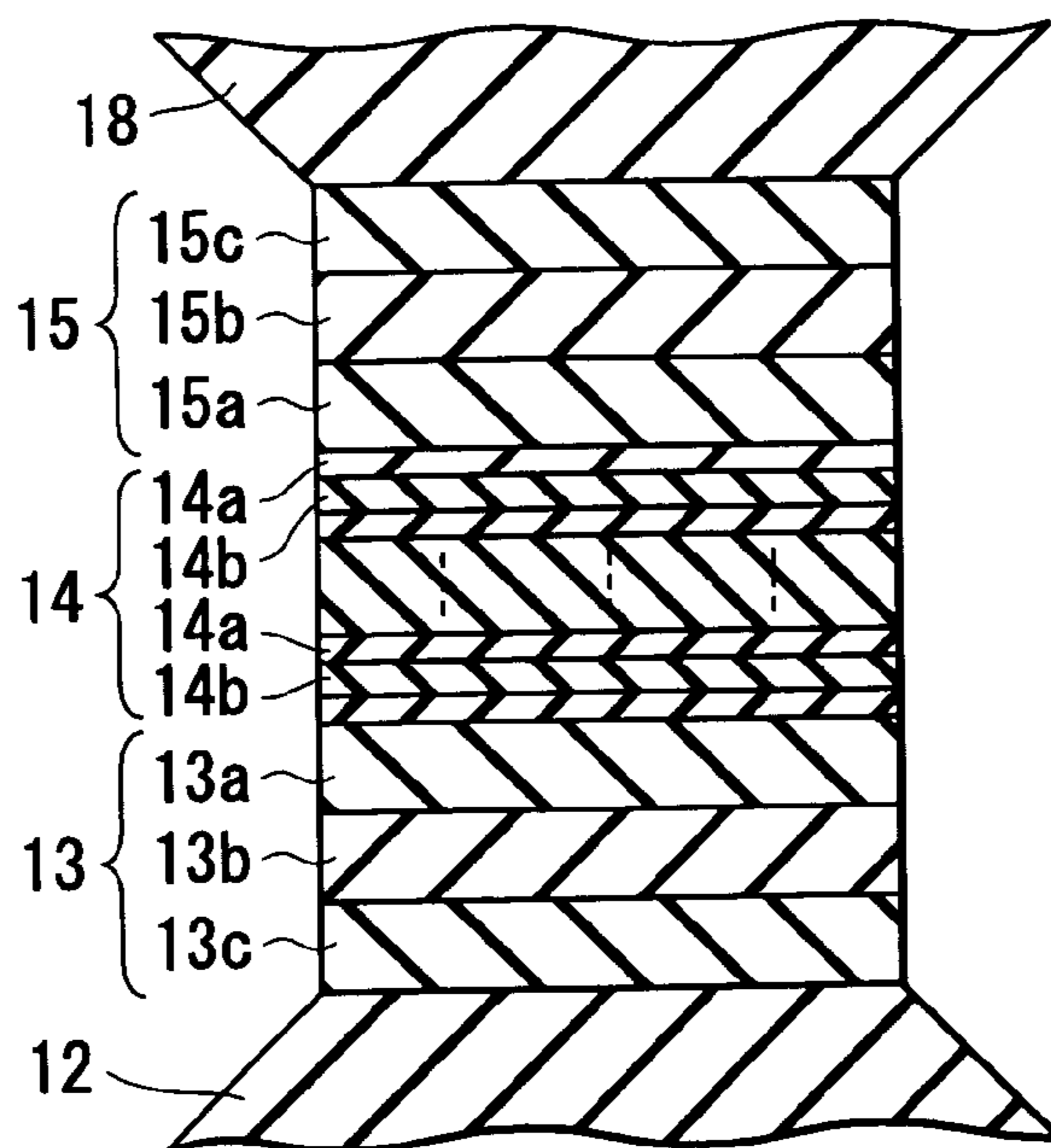
FIG. 13 (PRIOR ART)
