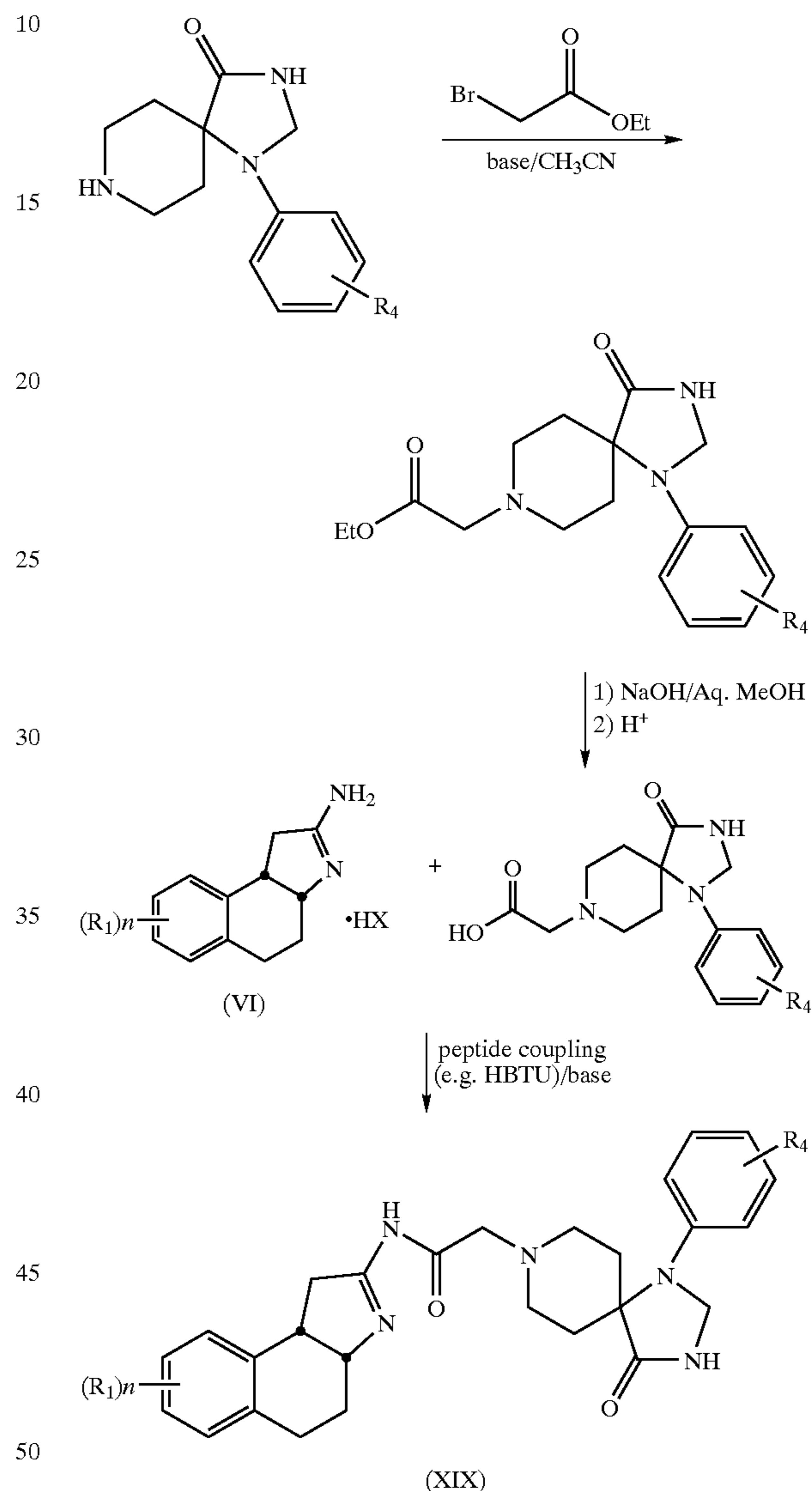
Scheme 9
