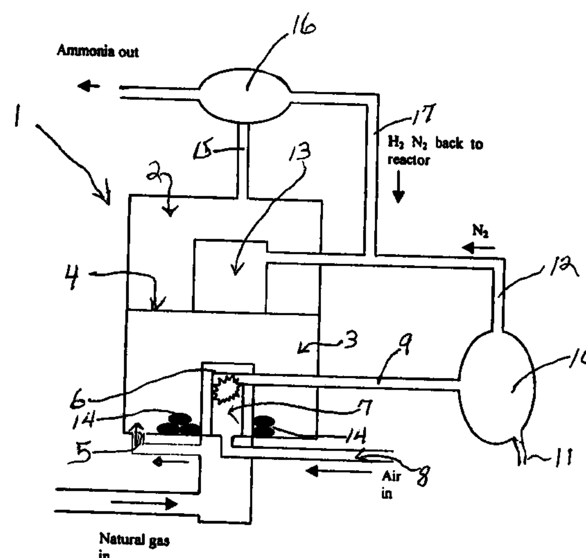
Combined Process Chemical Reactor
