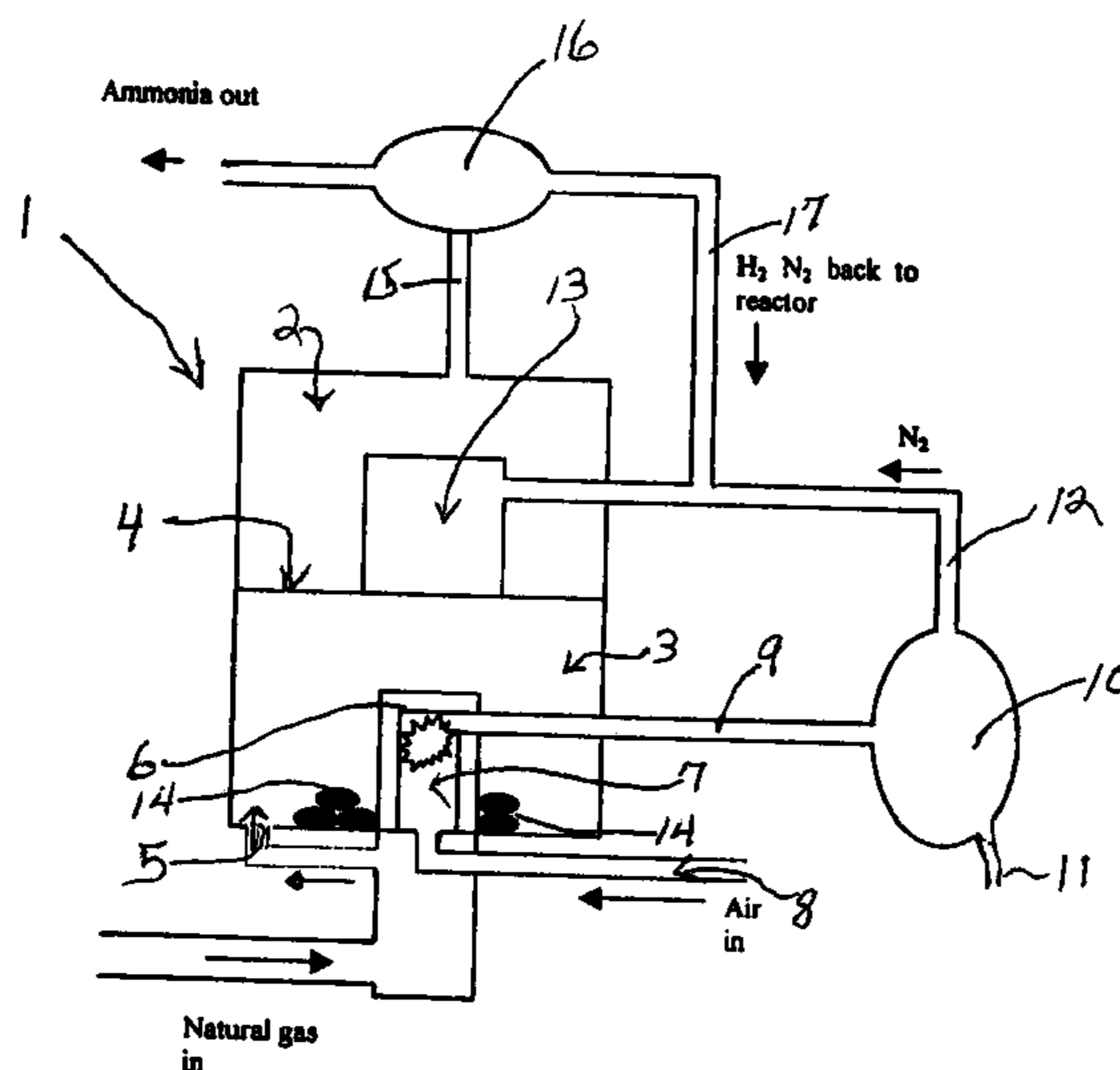
Combined Process Chemical Reactor
