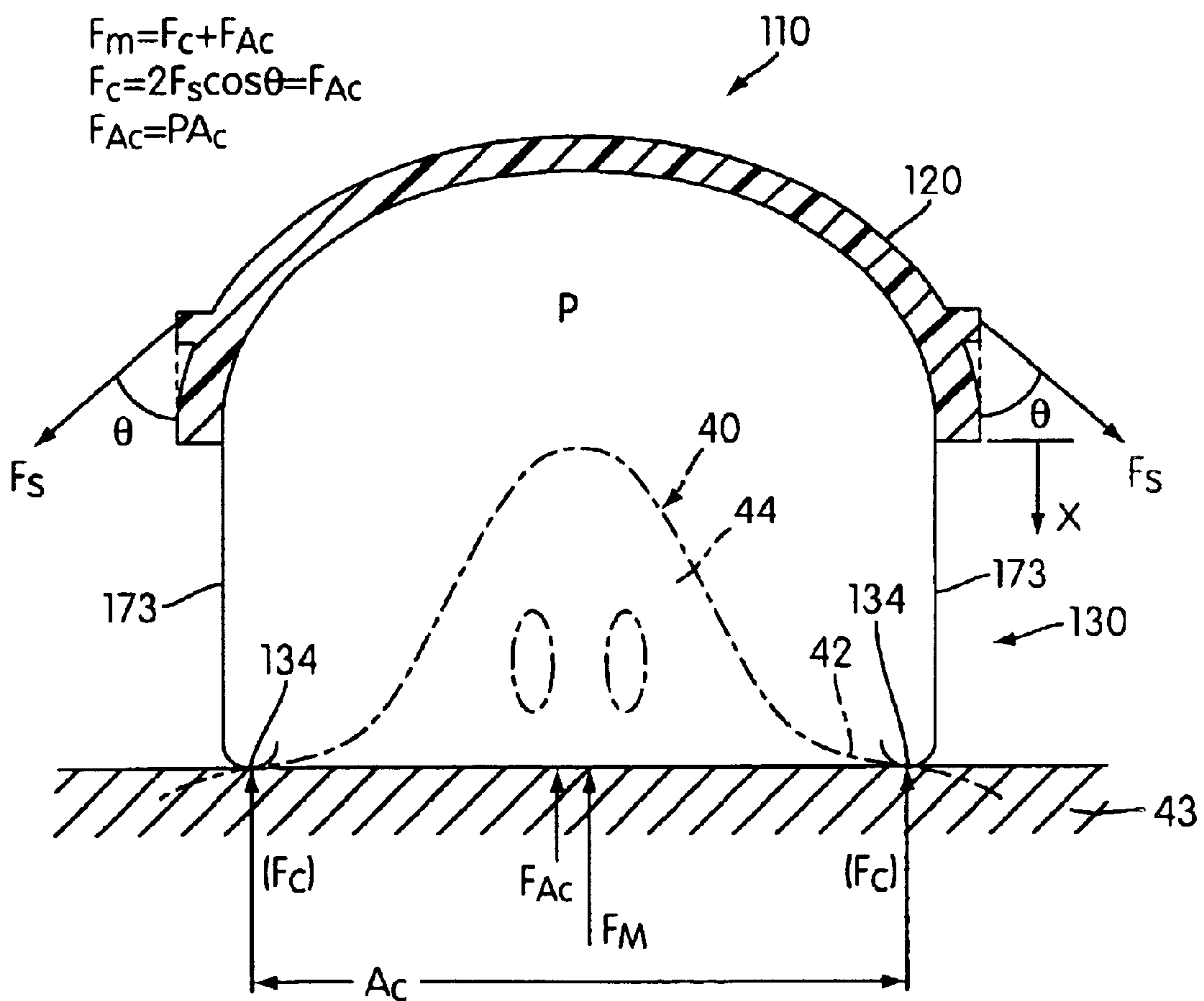
FIG. 1 PRIOR ART
