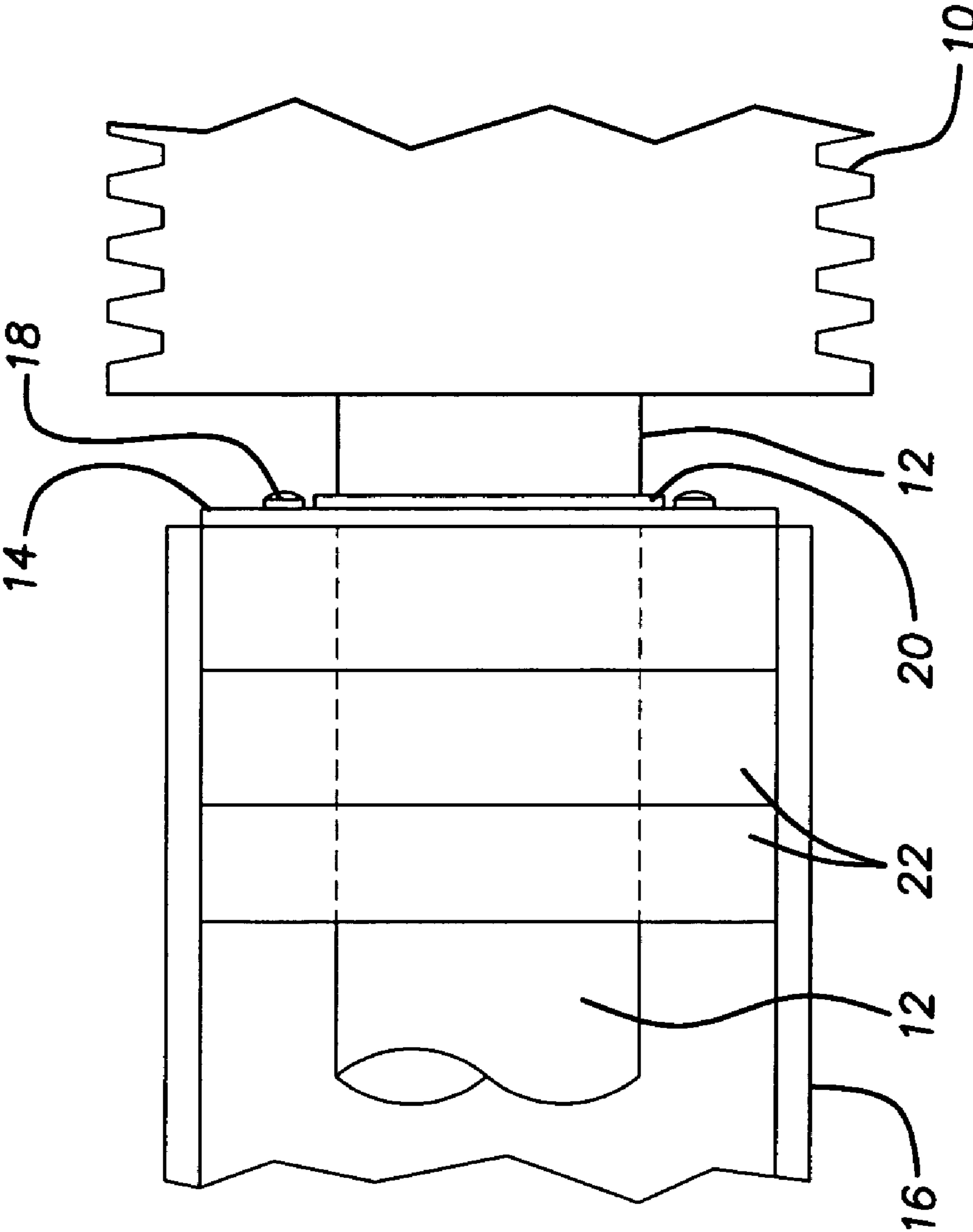
FIG. 1 PRIOR ART
