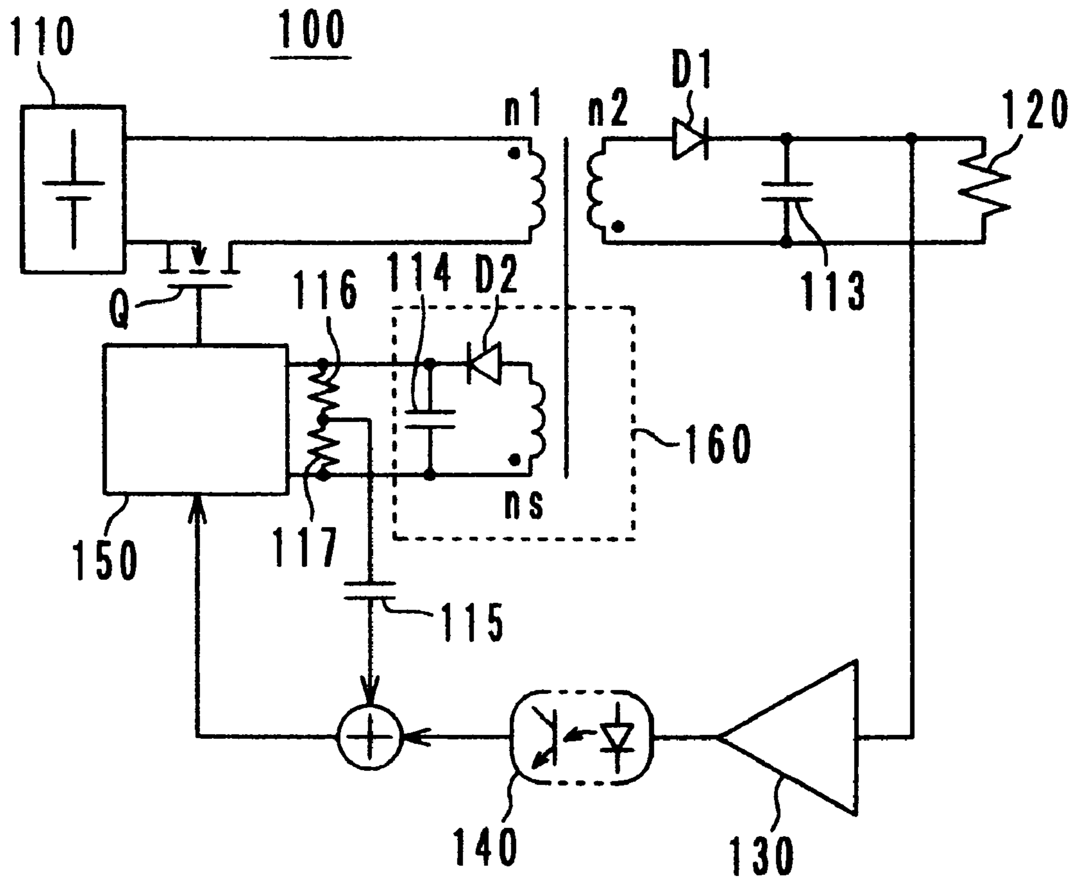
FIG. 5 PRIOR ART
