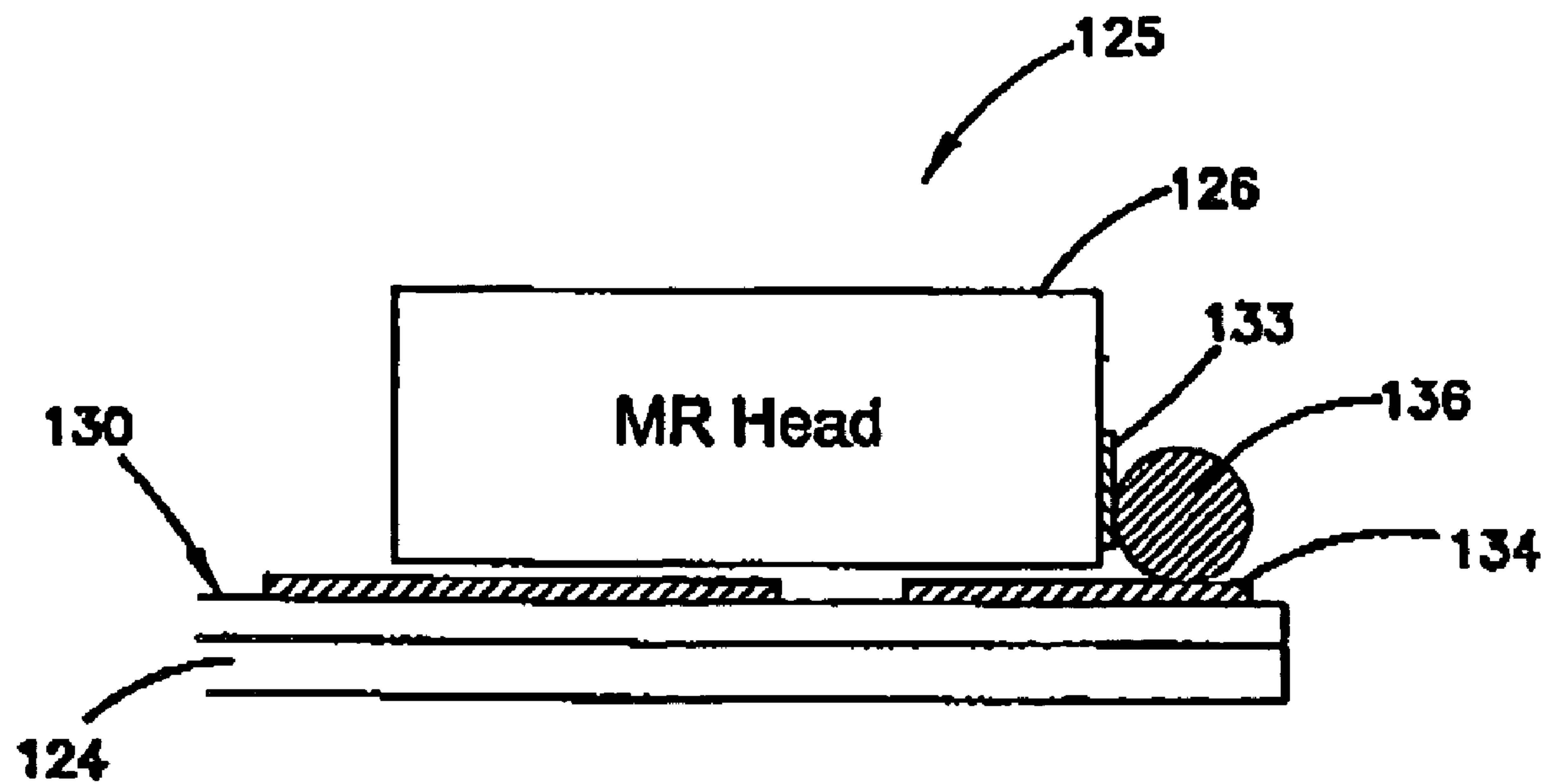
FIG. 2 (Prior Art)
