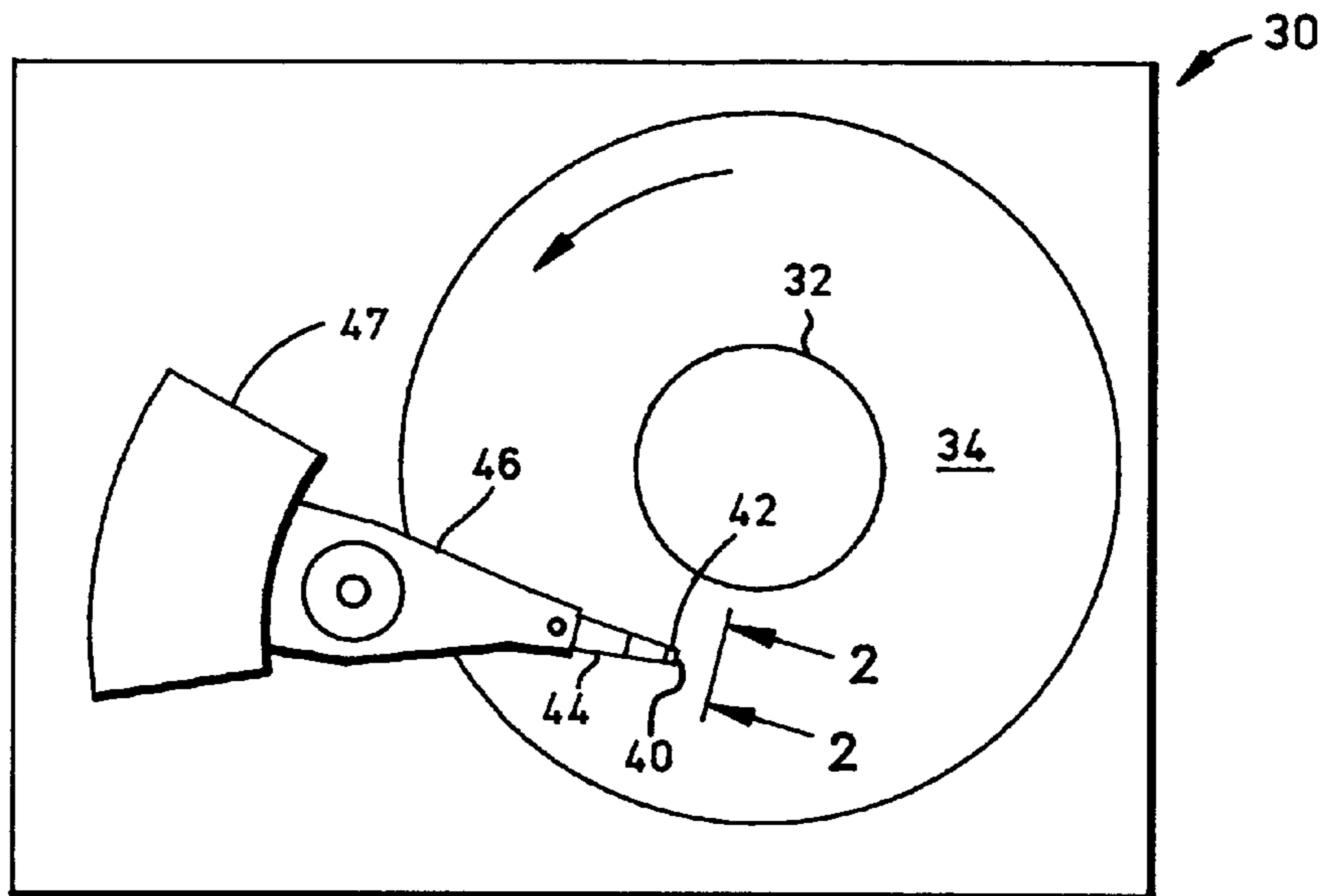
FIG. 1 (PRIOR ART)
