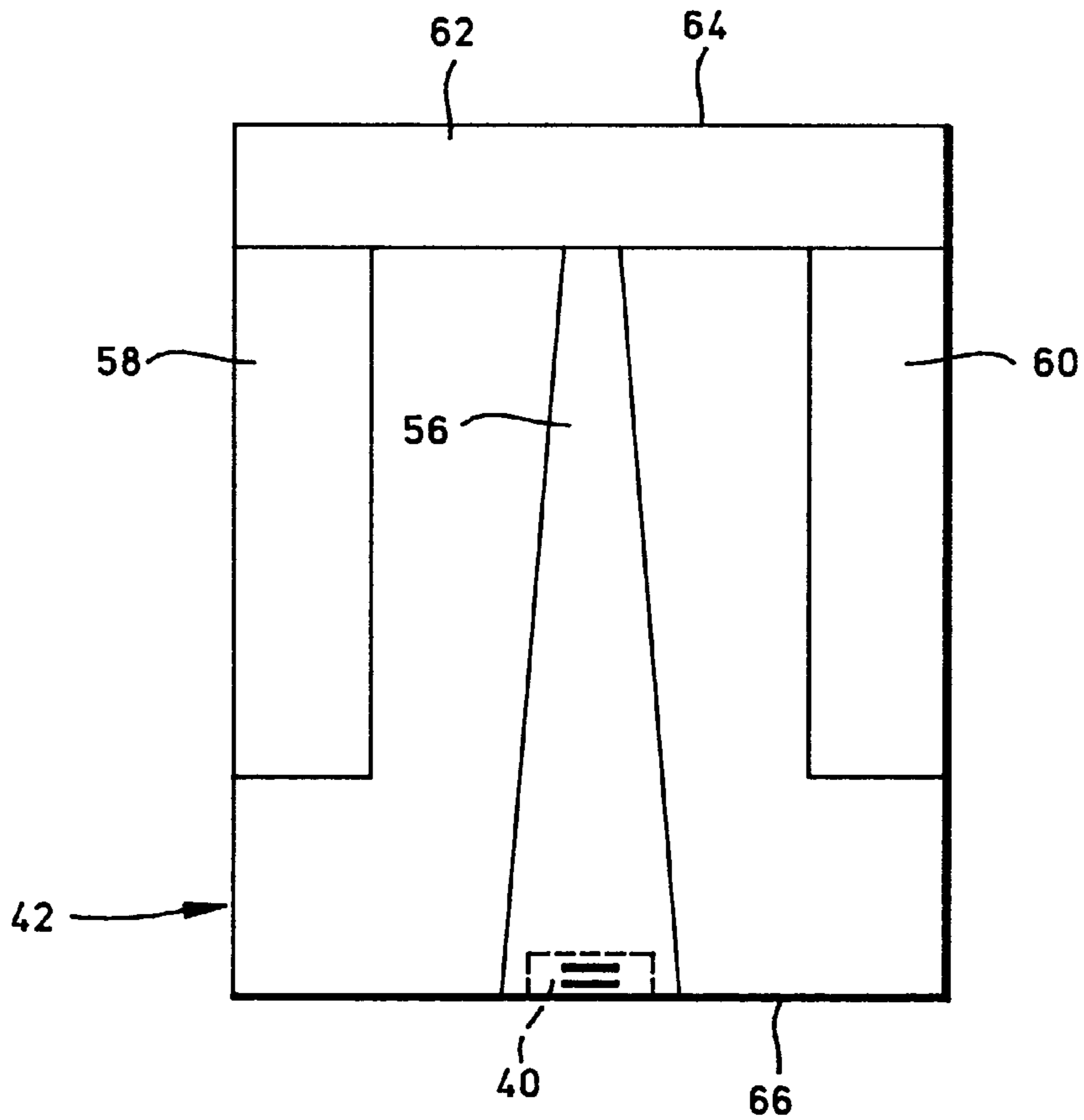
FIG. 5 (PRIOR ART)
