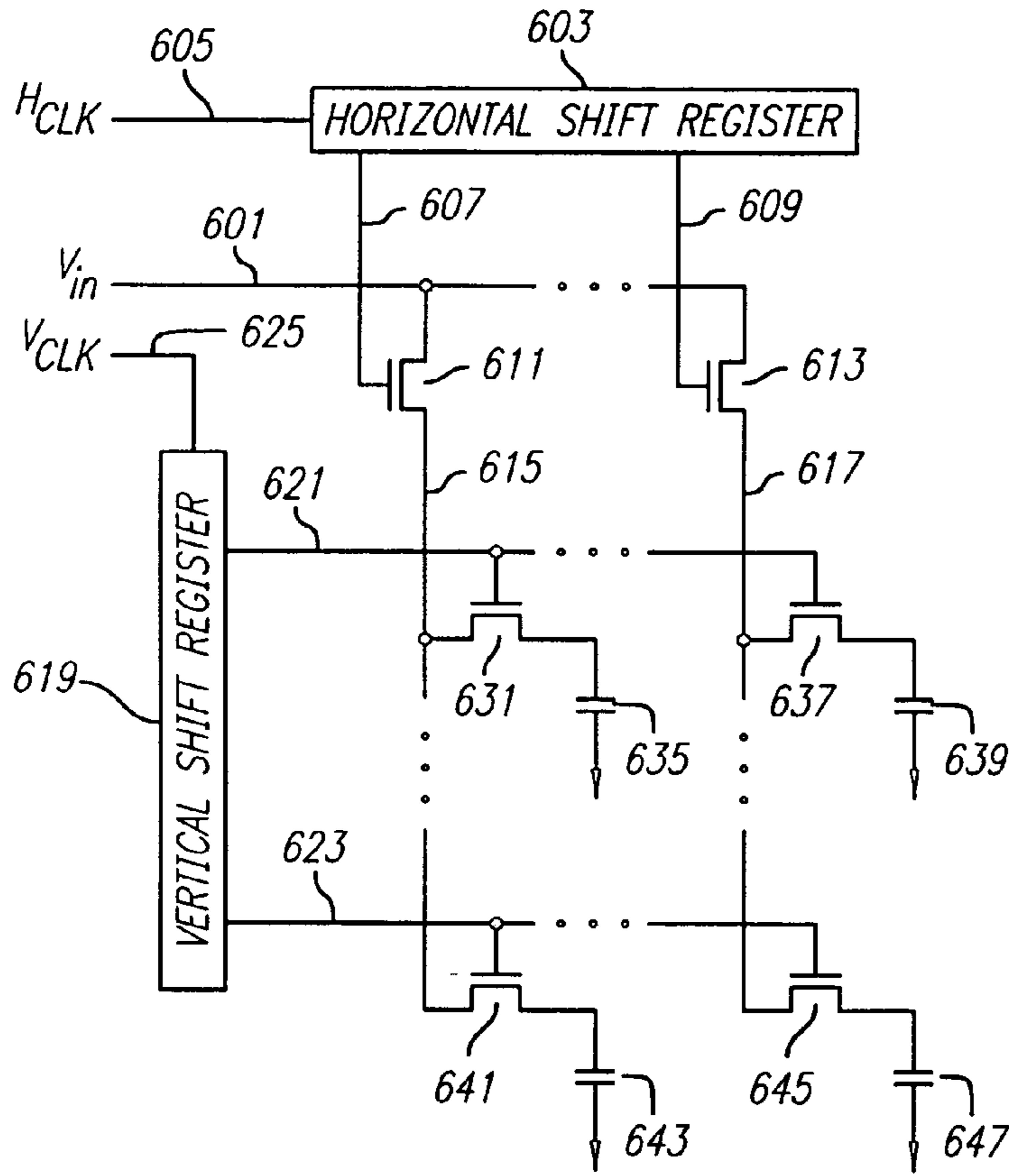
FIG. 12 PRIOR ART
