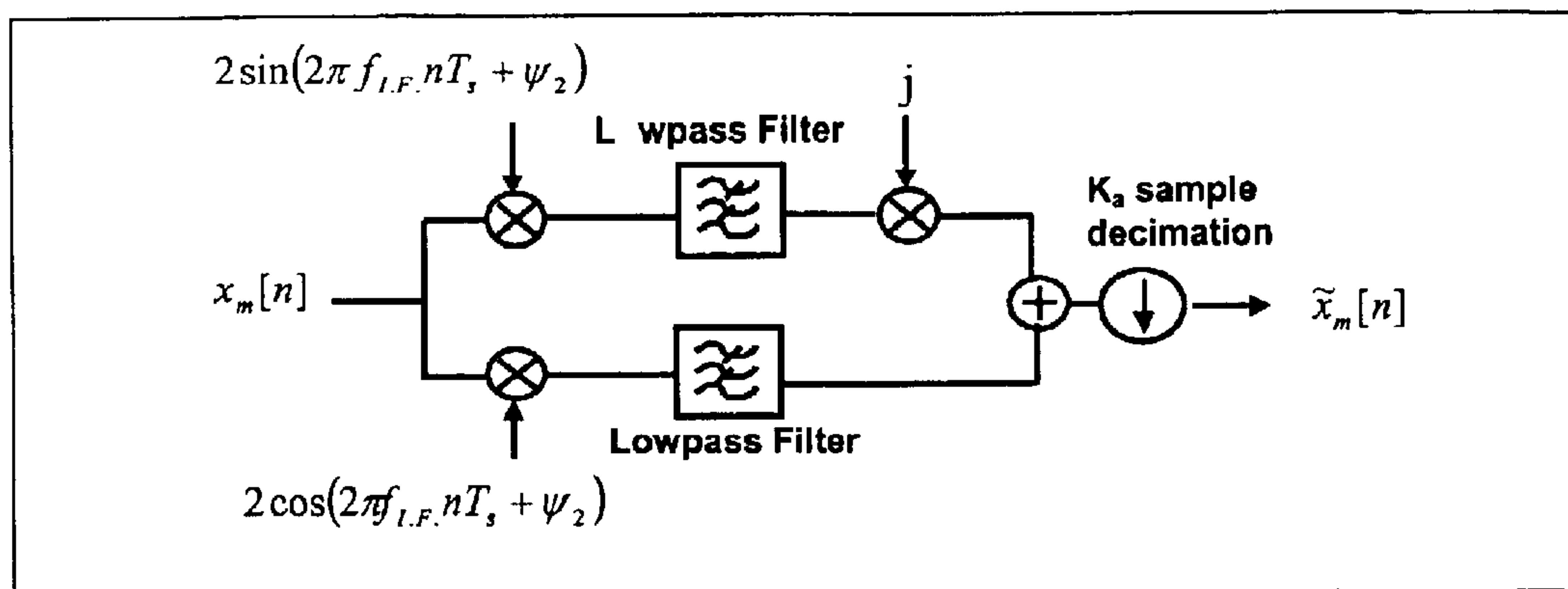
Figure 2 Complex Envelope OOK Demodulation
