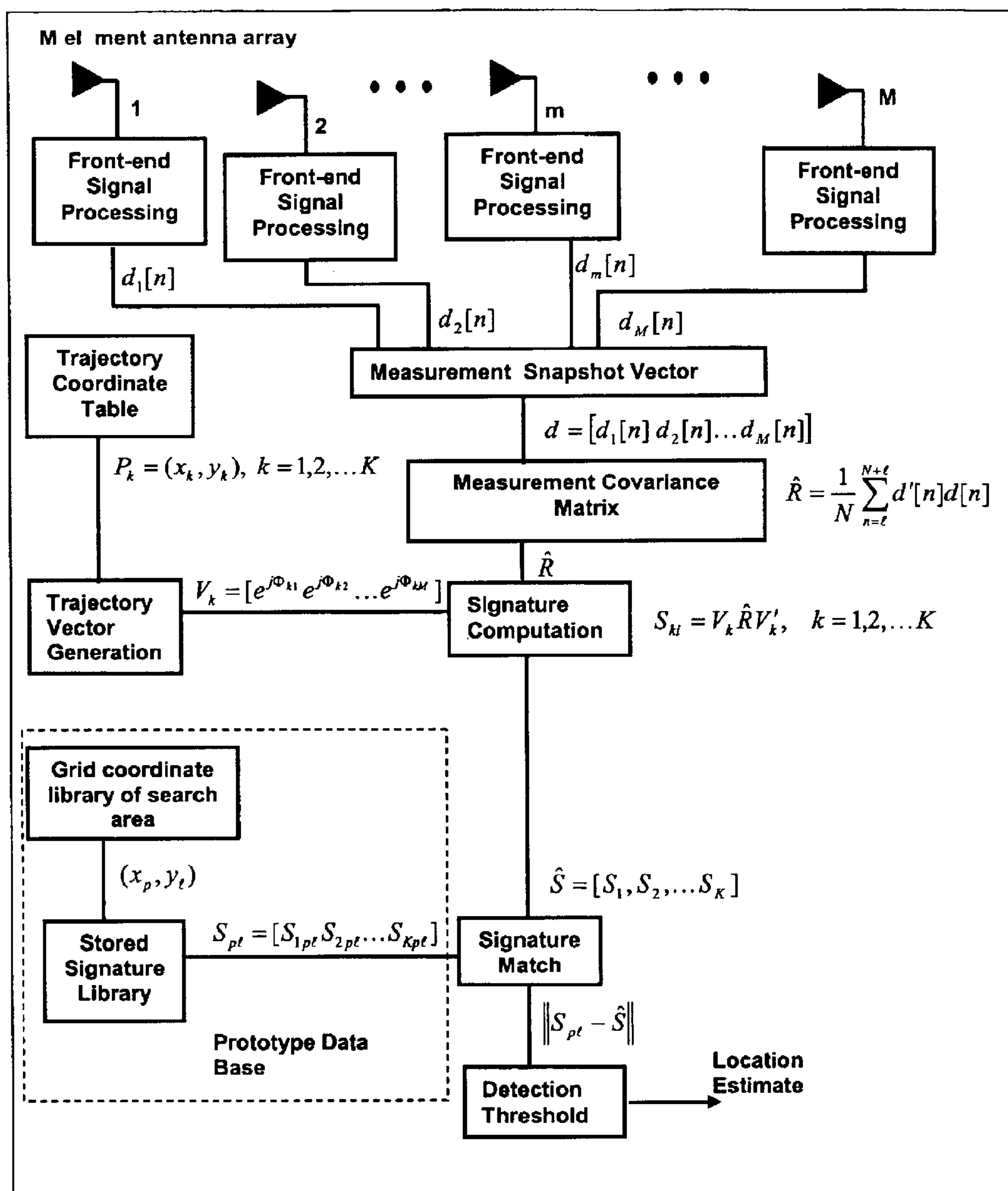
Figure 9 Radio Transmitter Location Estimation – Trajectory Signature Method (Non-CDMA processing)
