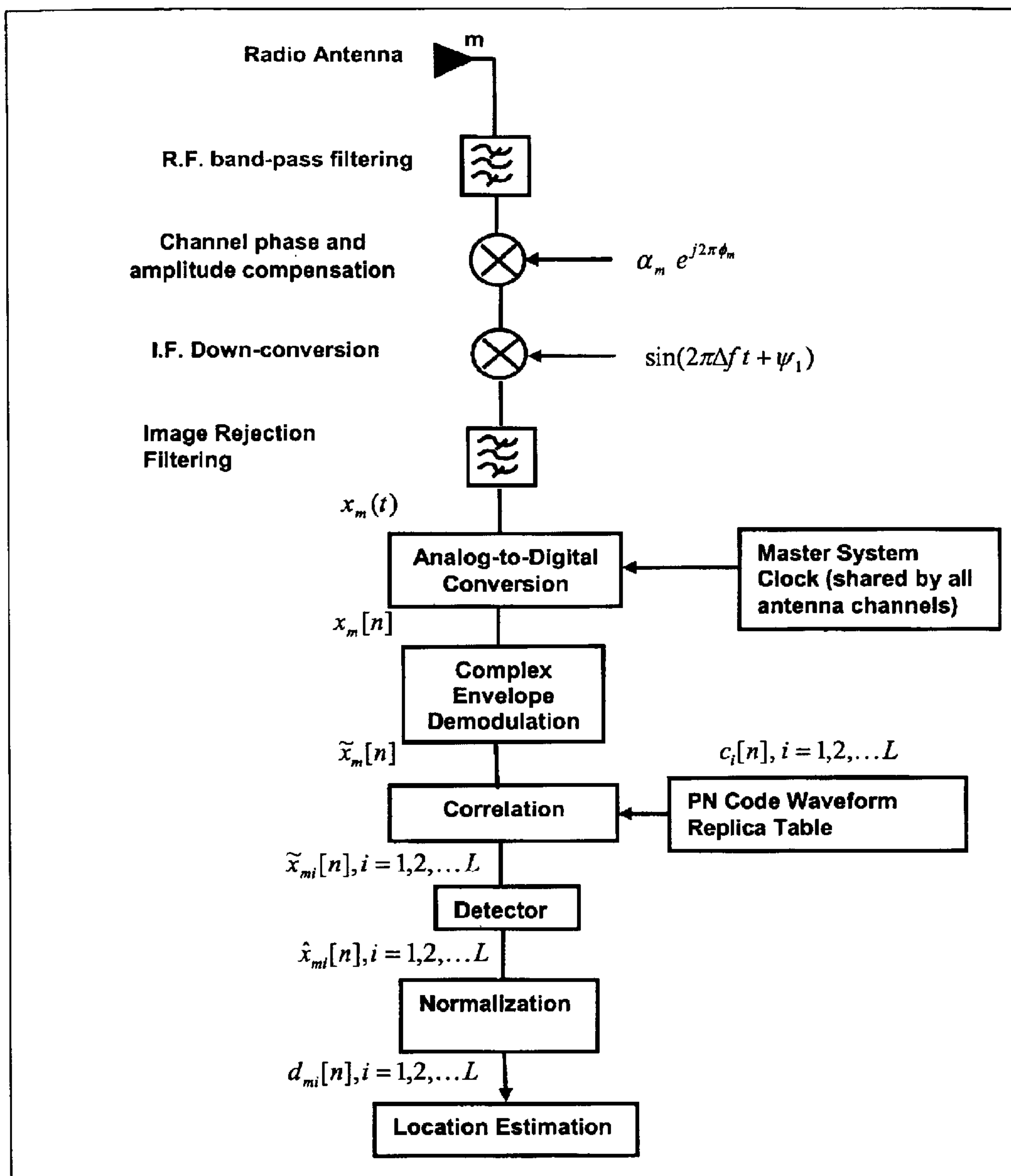
Figure 1 Front-end signal processing chain for m^{\text{th}} antenna chain CDMA applications
