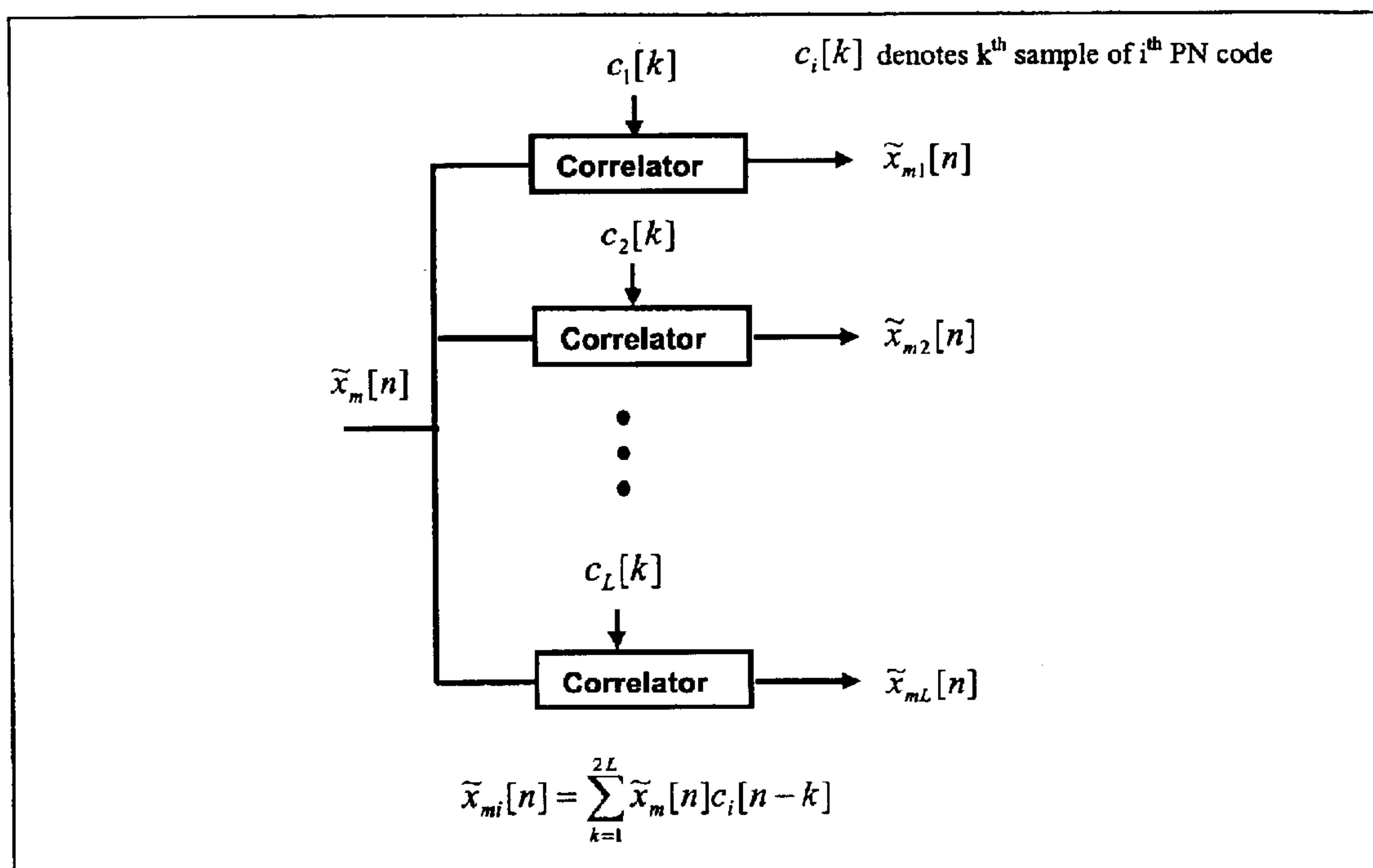
Figure 3 Correlator Operation
