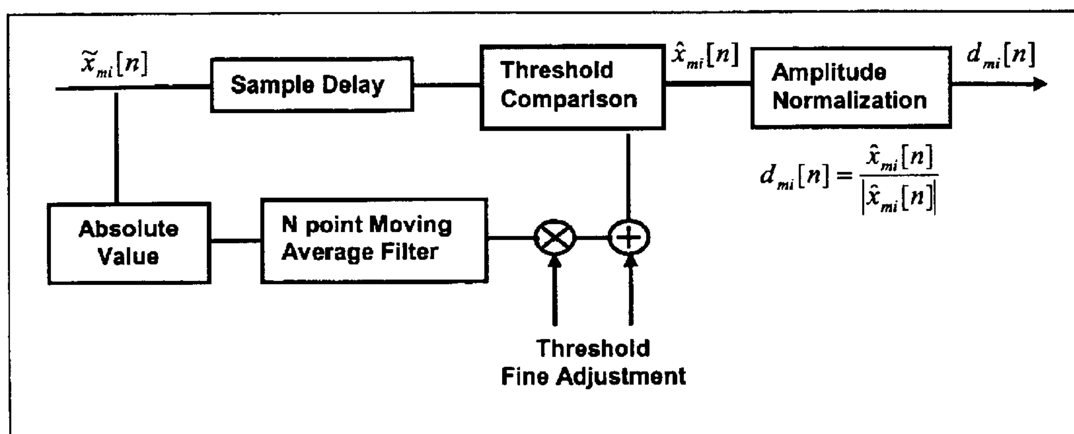
Figure 4 Threshold Generation and Normalization – i^{\text{th}} code channel
