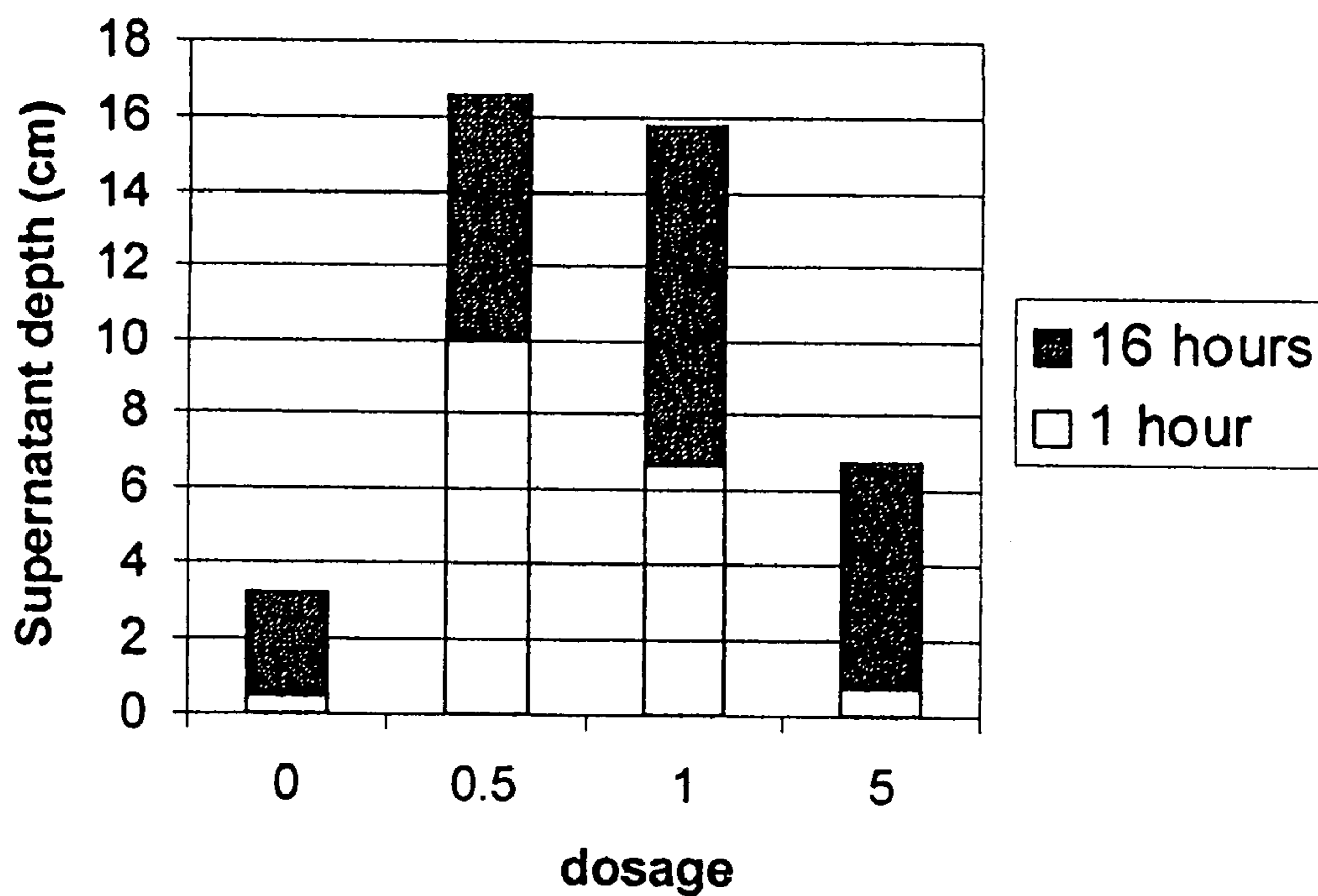
Figure 7 – Incremental depth of supernatant layer above settled sludge as a function of seed dosage.
