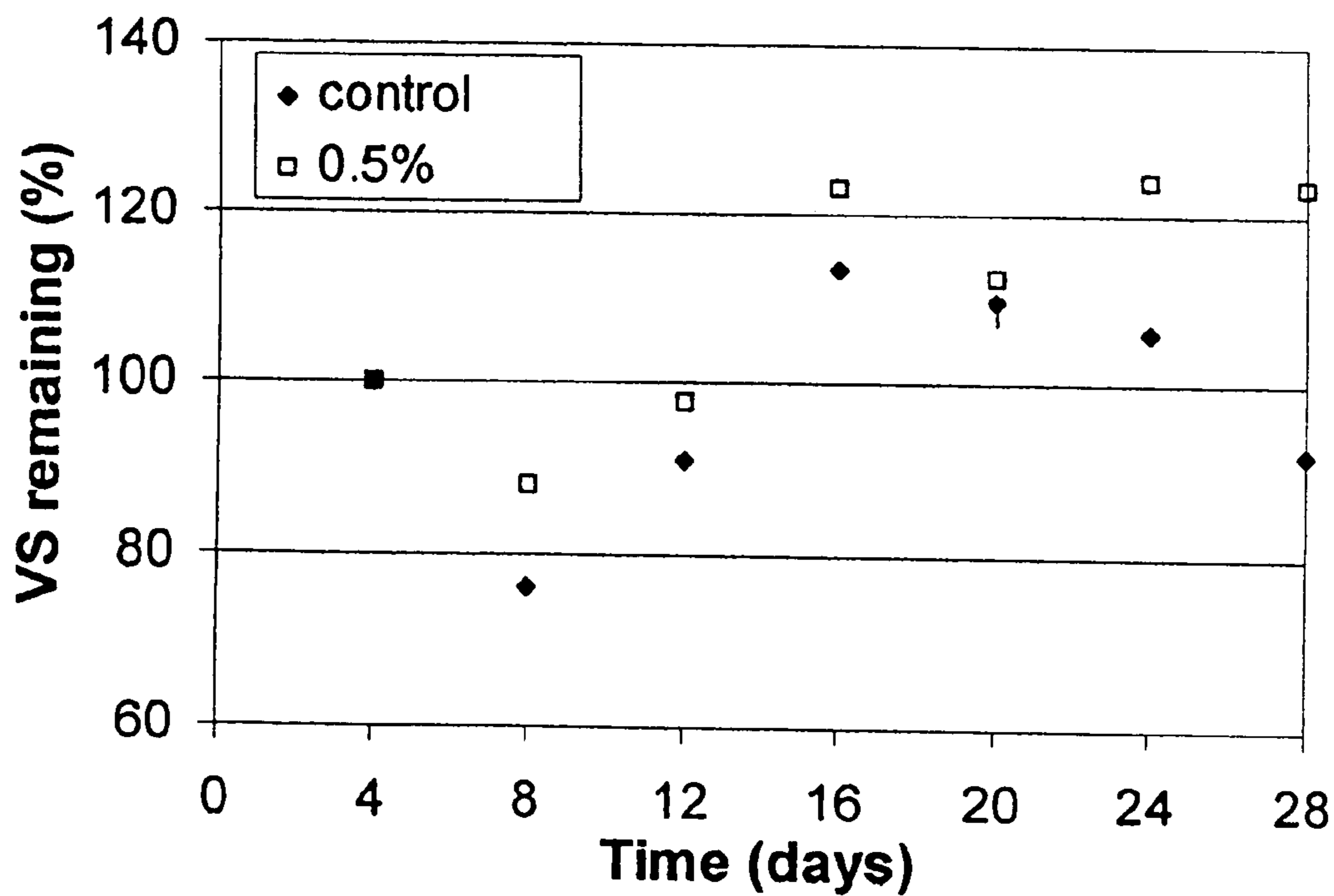
Figure 2. Volatile solids remaining versus time at 8°C.
