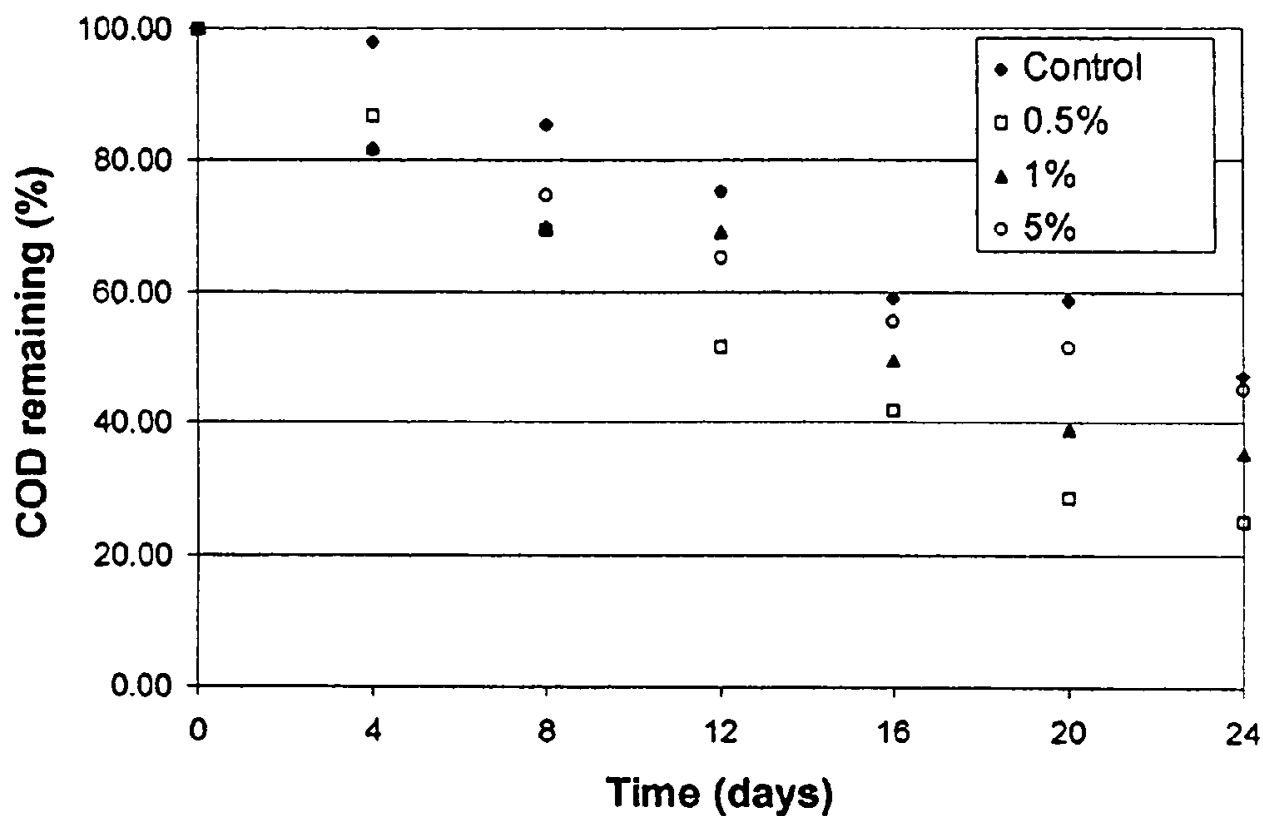
Figure 5 – COD remaining versus time at 23°C .
