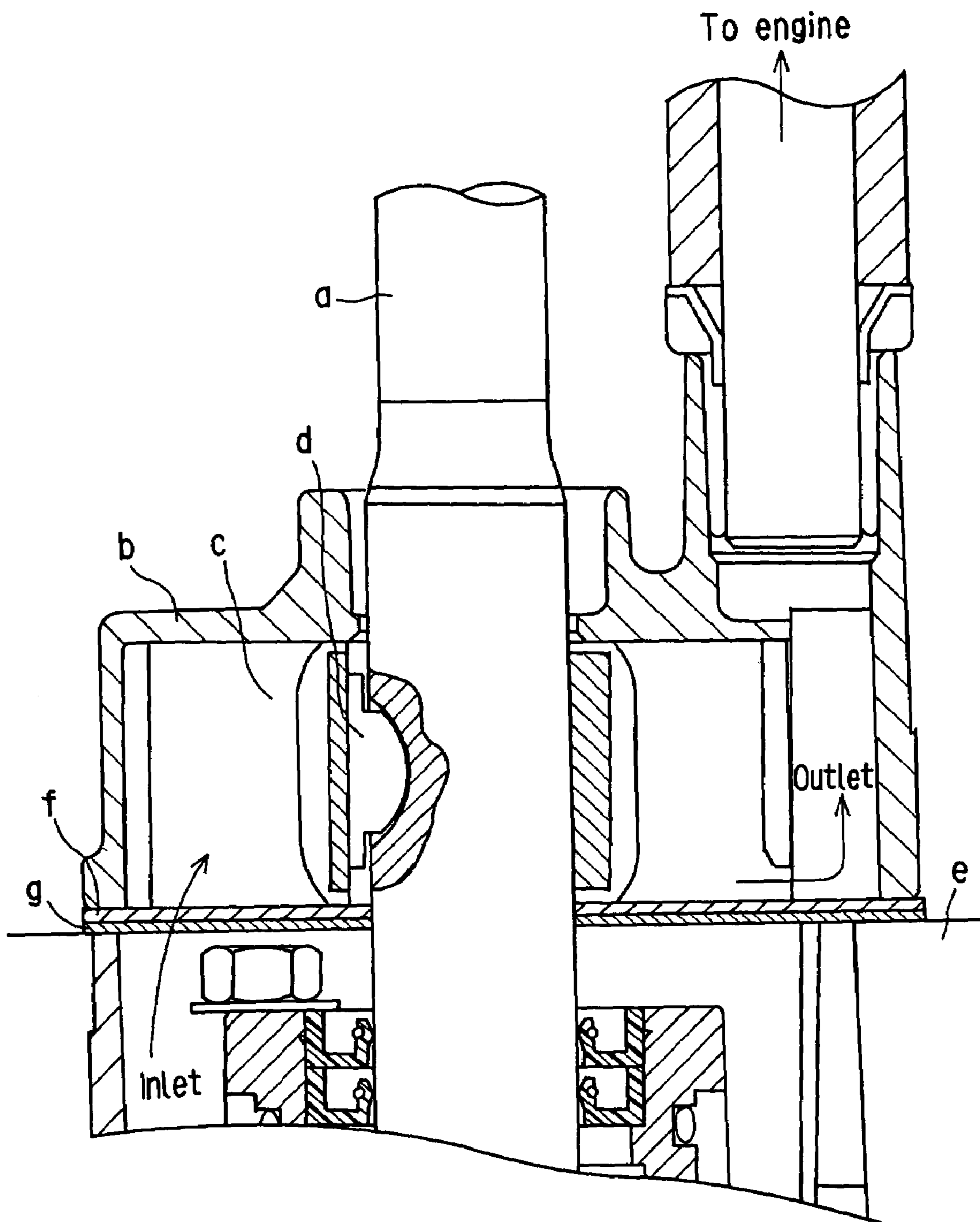
Conventional stainless cooling pump configuration
