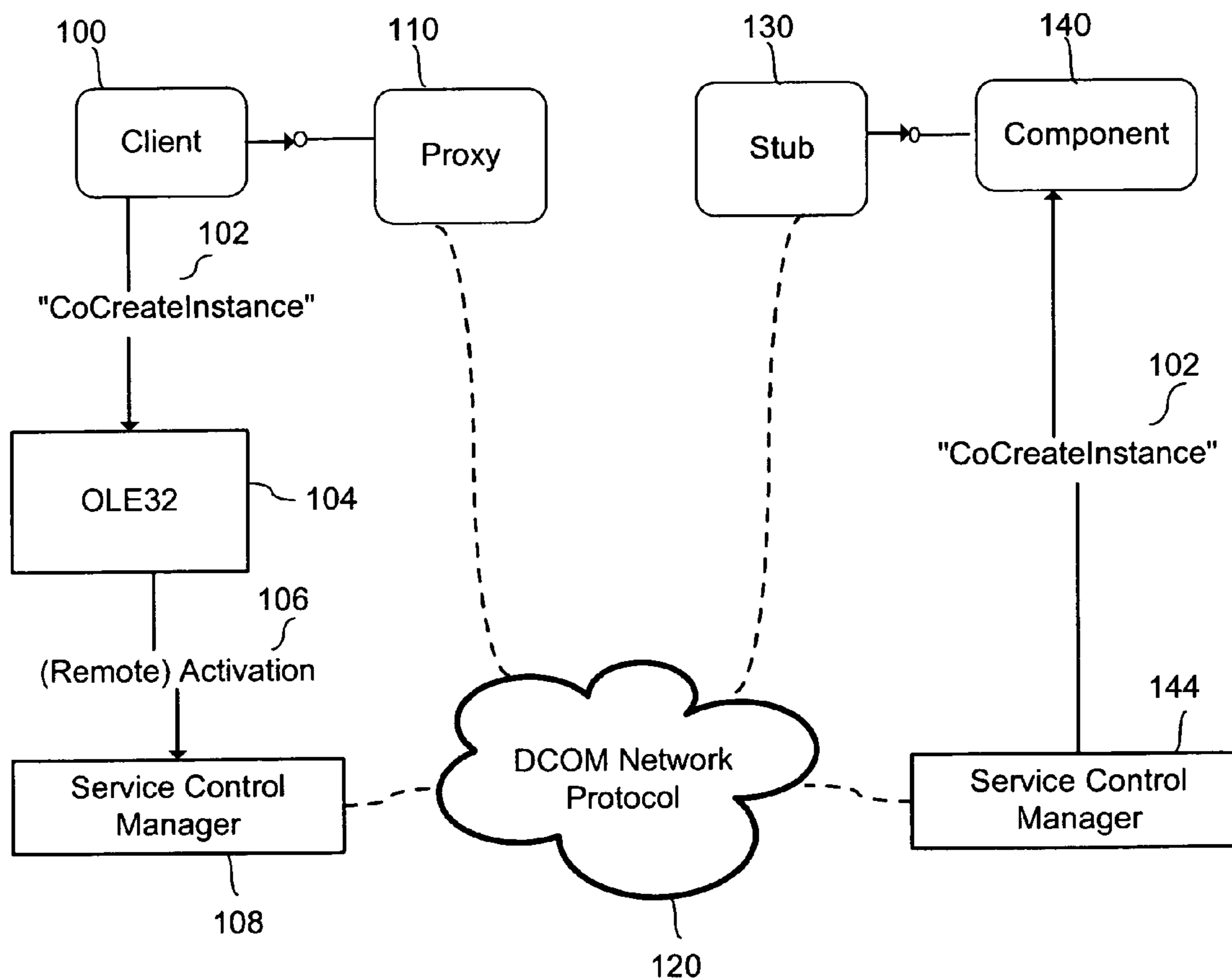
Distributed Computing Environment with Client and COM Component for Application Partitioned and Distributed by ADPS with Network-Independent Profiling of Applications
