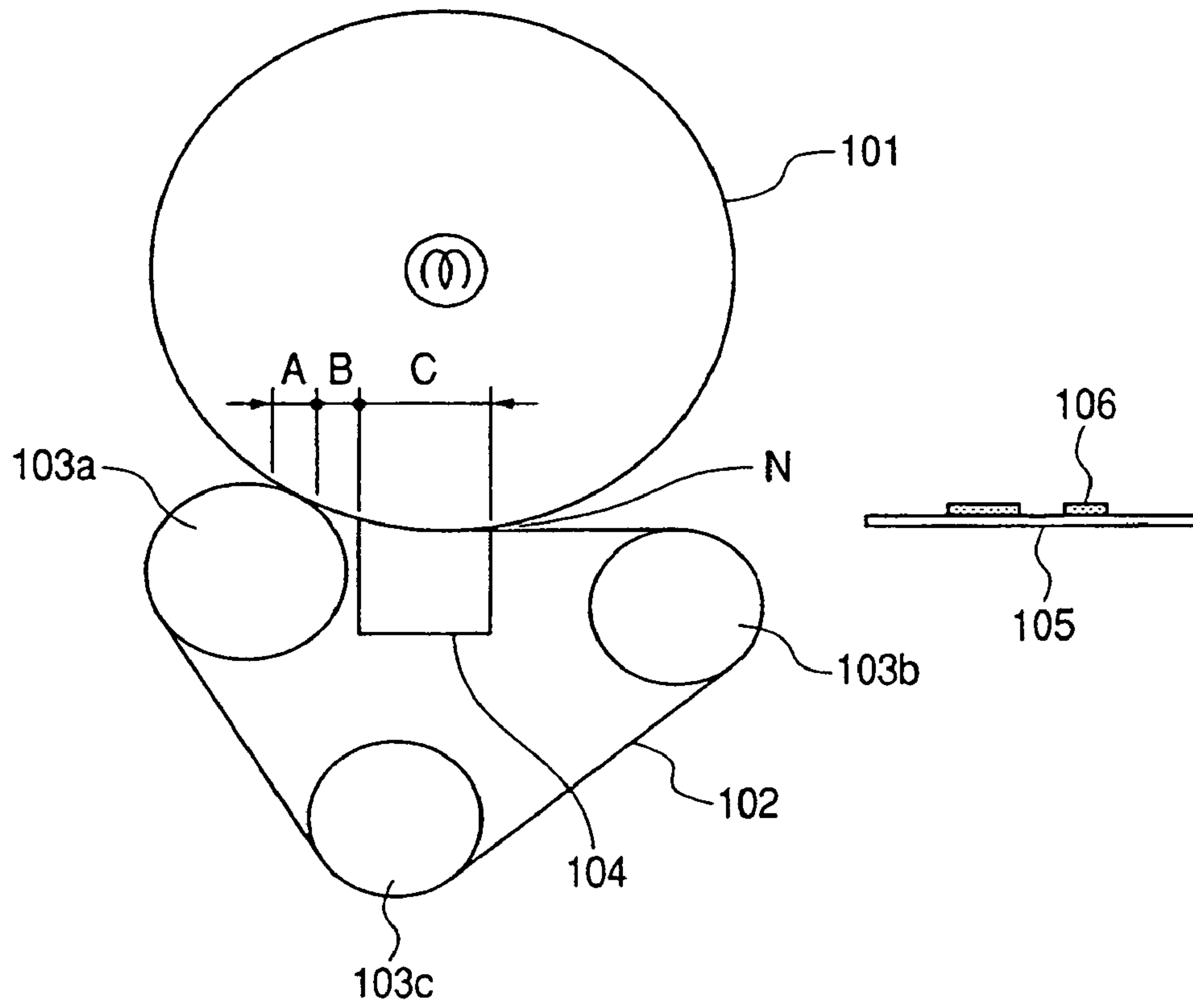
FIG. 8 PRIOR ART
