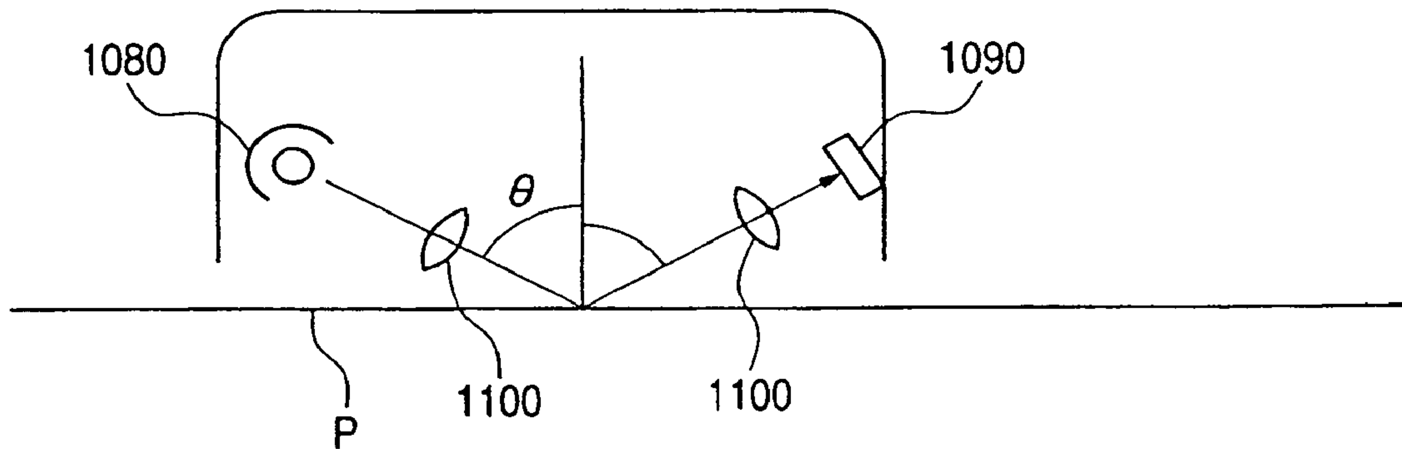
FIG. 9 PRIOR ART
