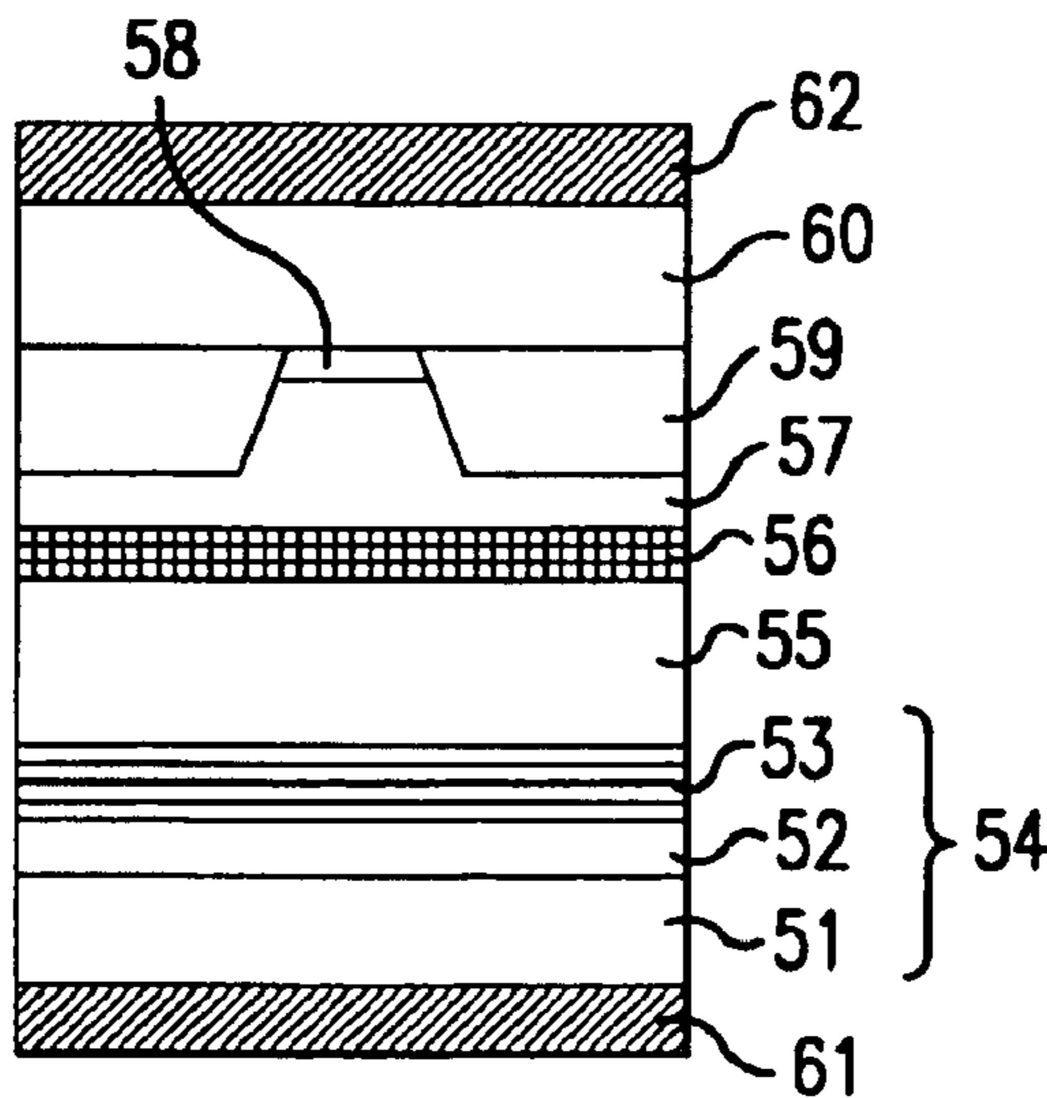
FIG.7 PRIOR ART
