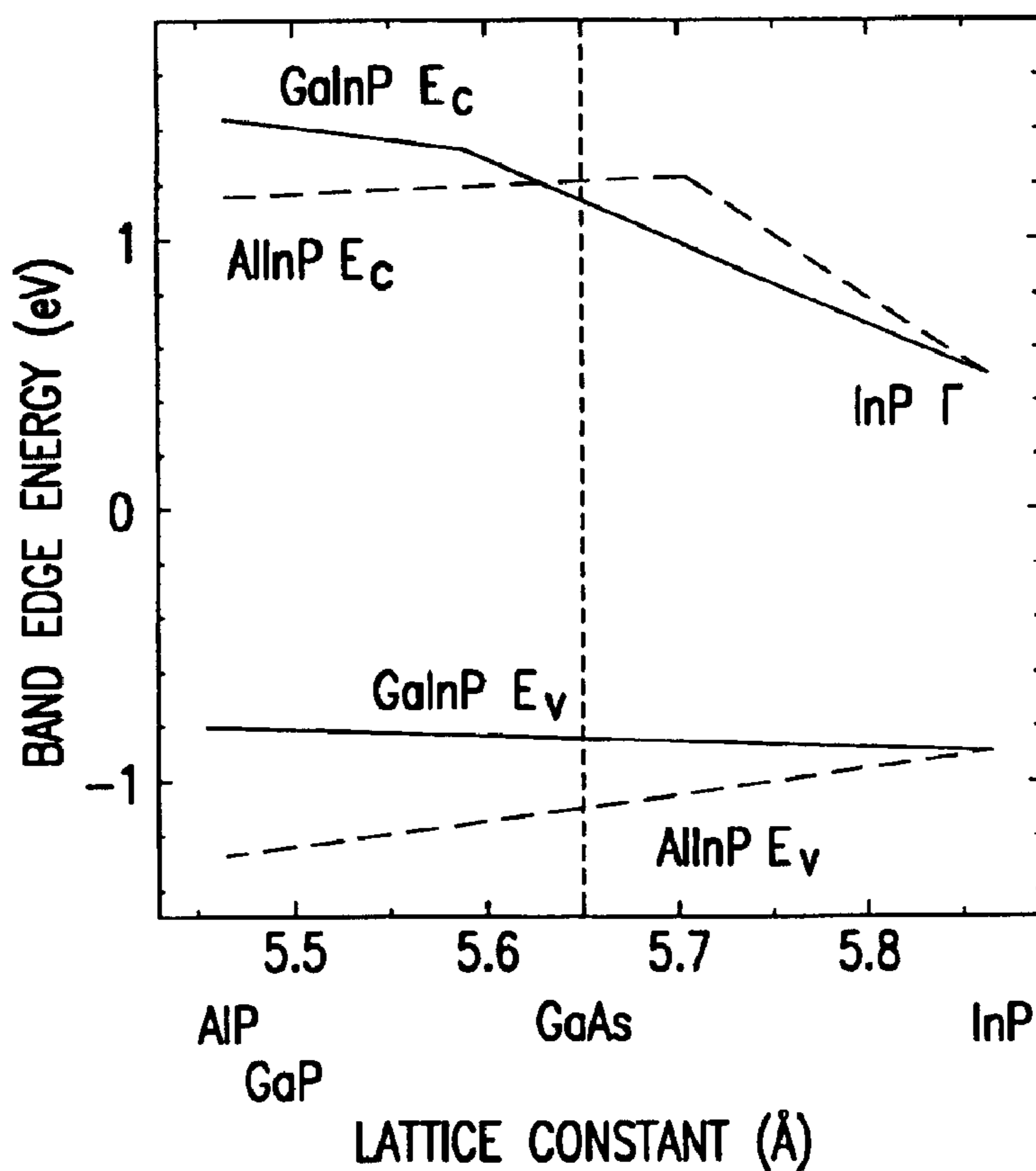
FIG. 5 PRIOR ART
