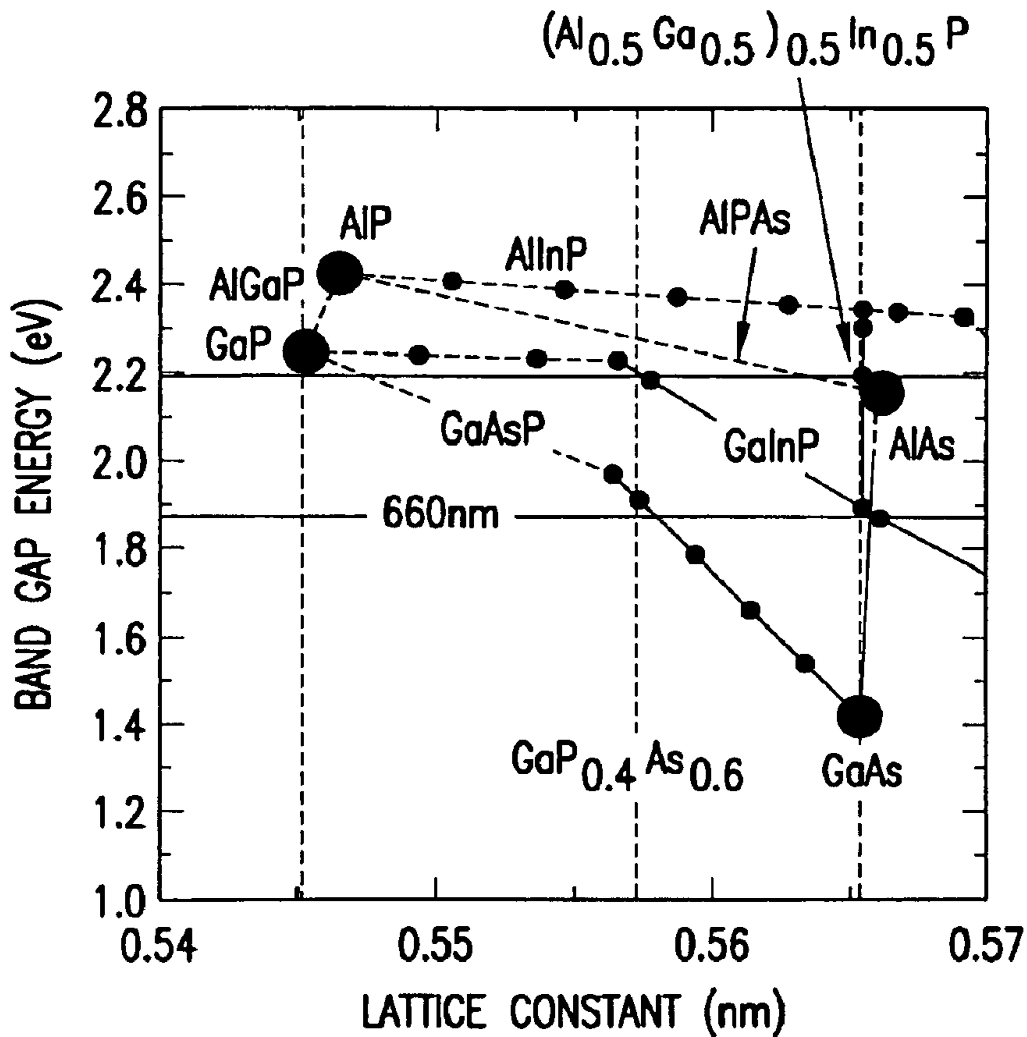
FIG.6 PRIOR ART
