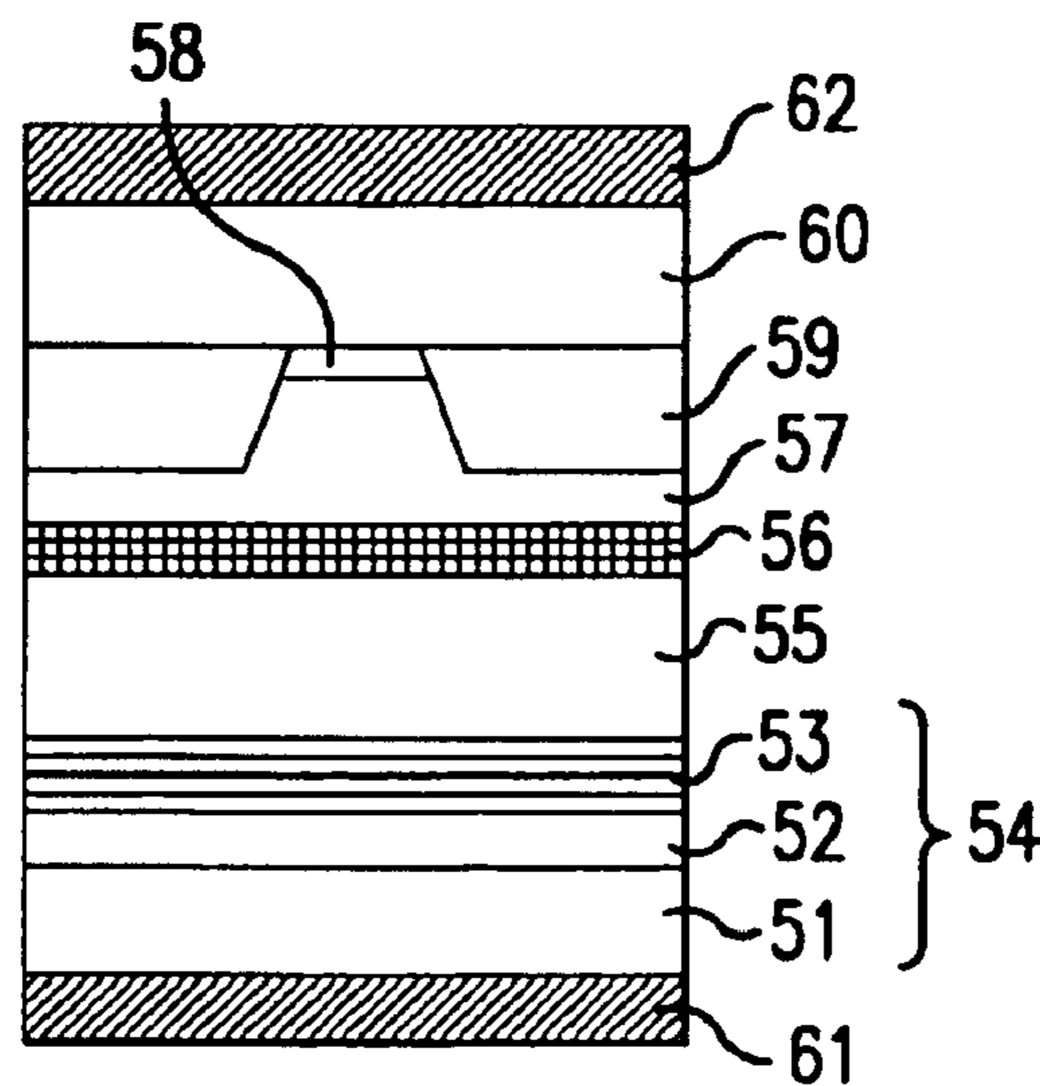
FIG.7 PRIOR ART
