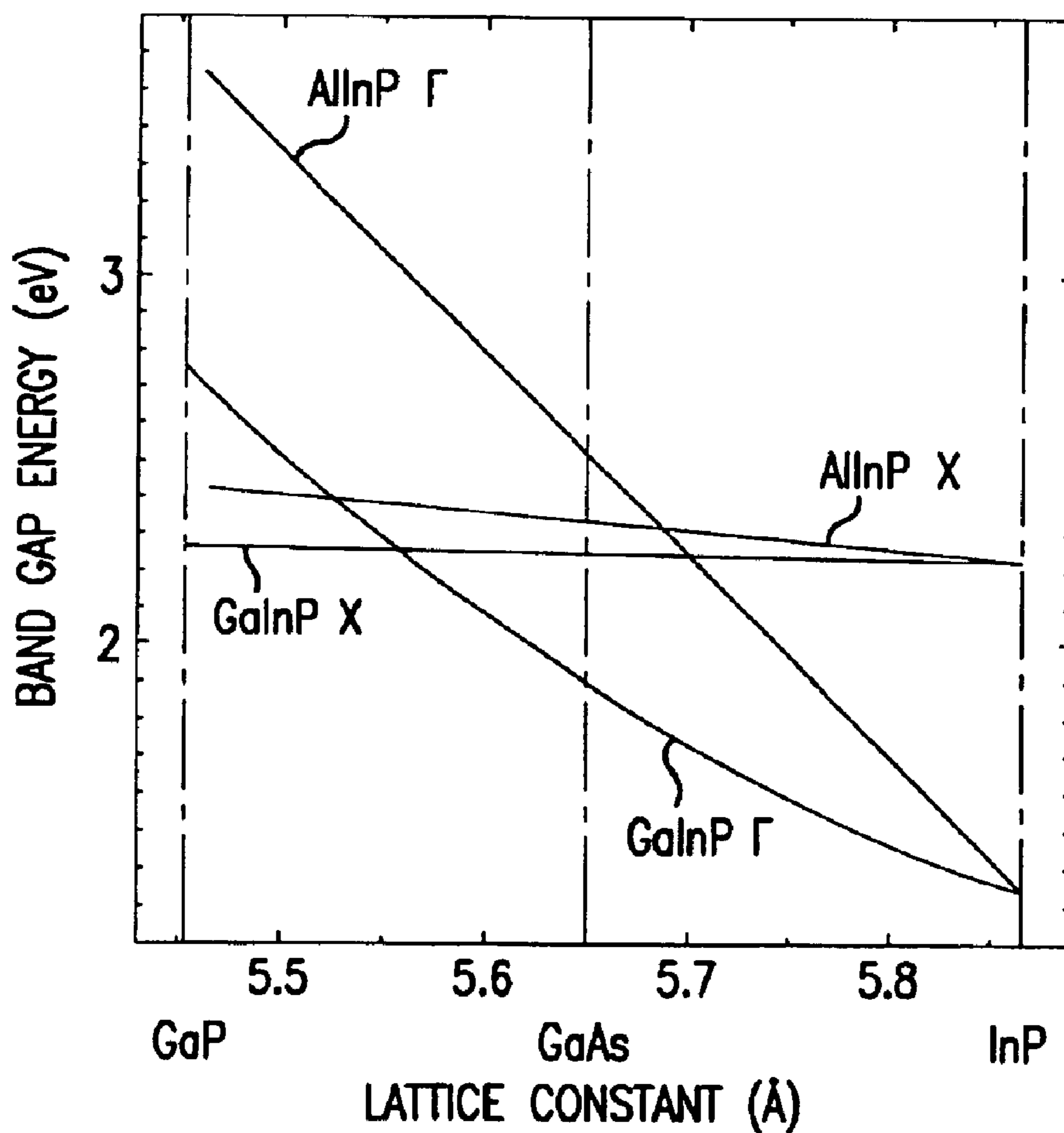
FIG.8 PRIOR ART
