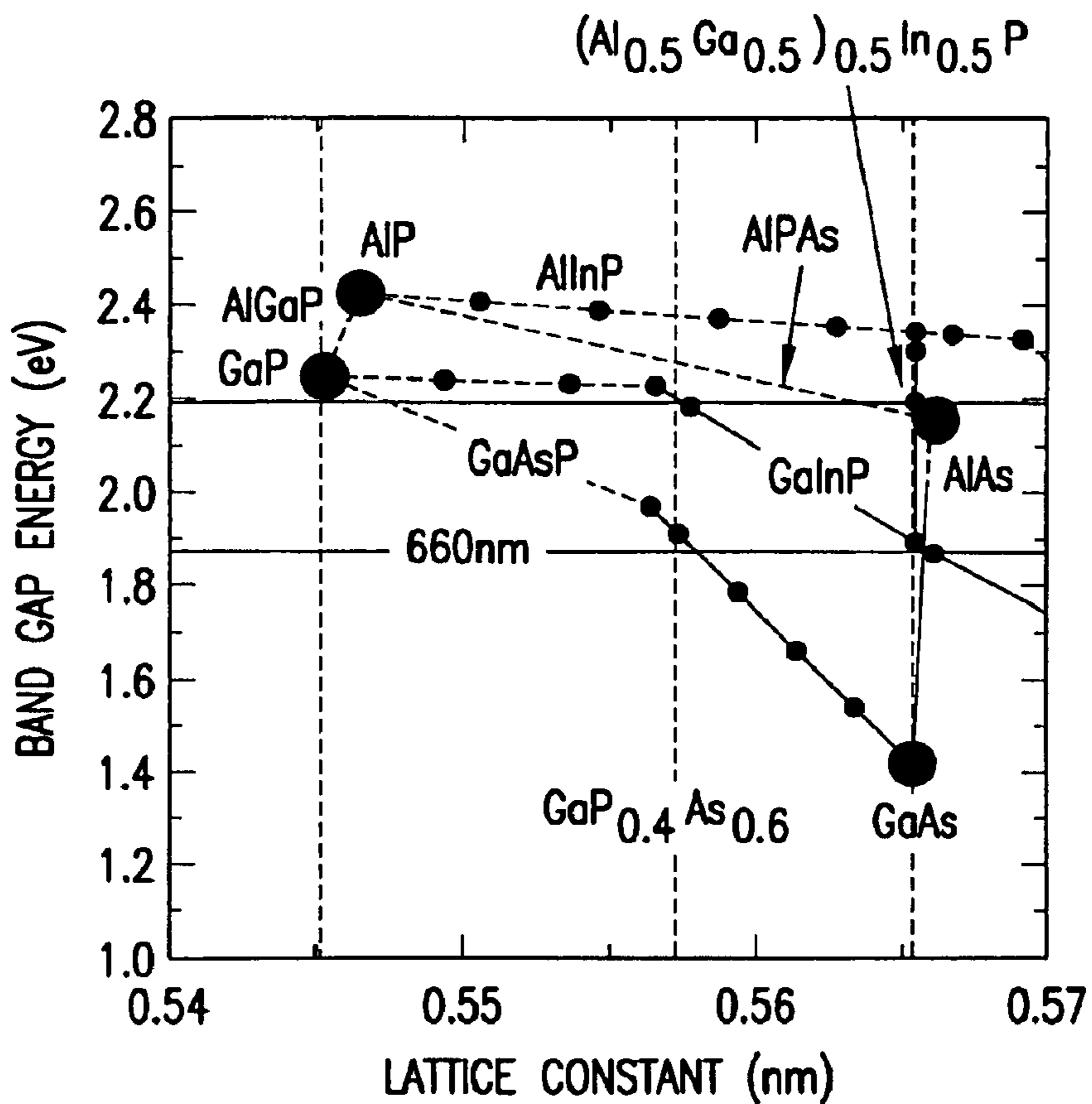
FIG.6 PRIOR ART
