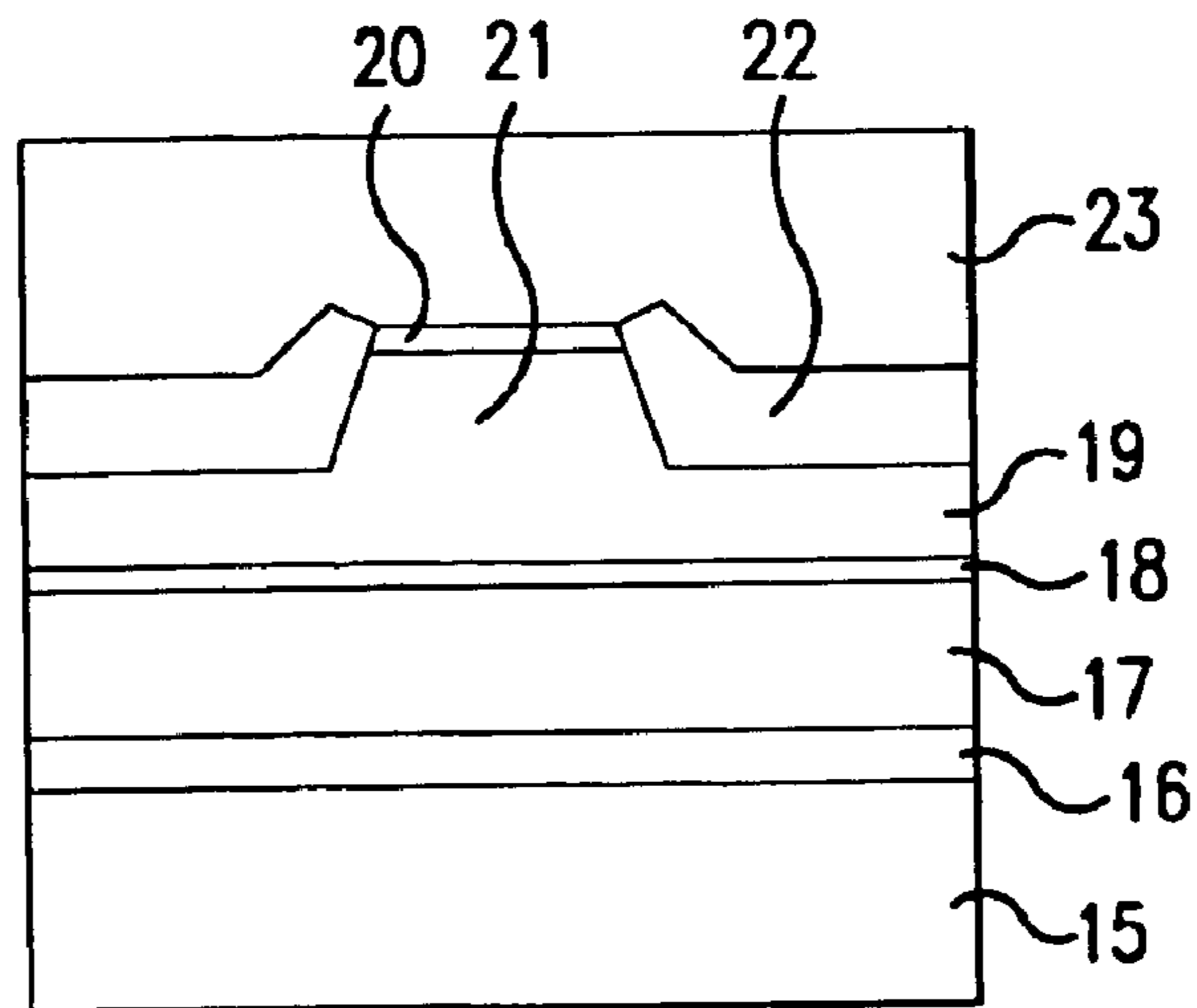
FIG. 2 PRIOR ART
