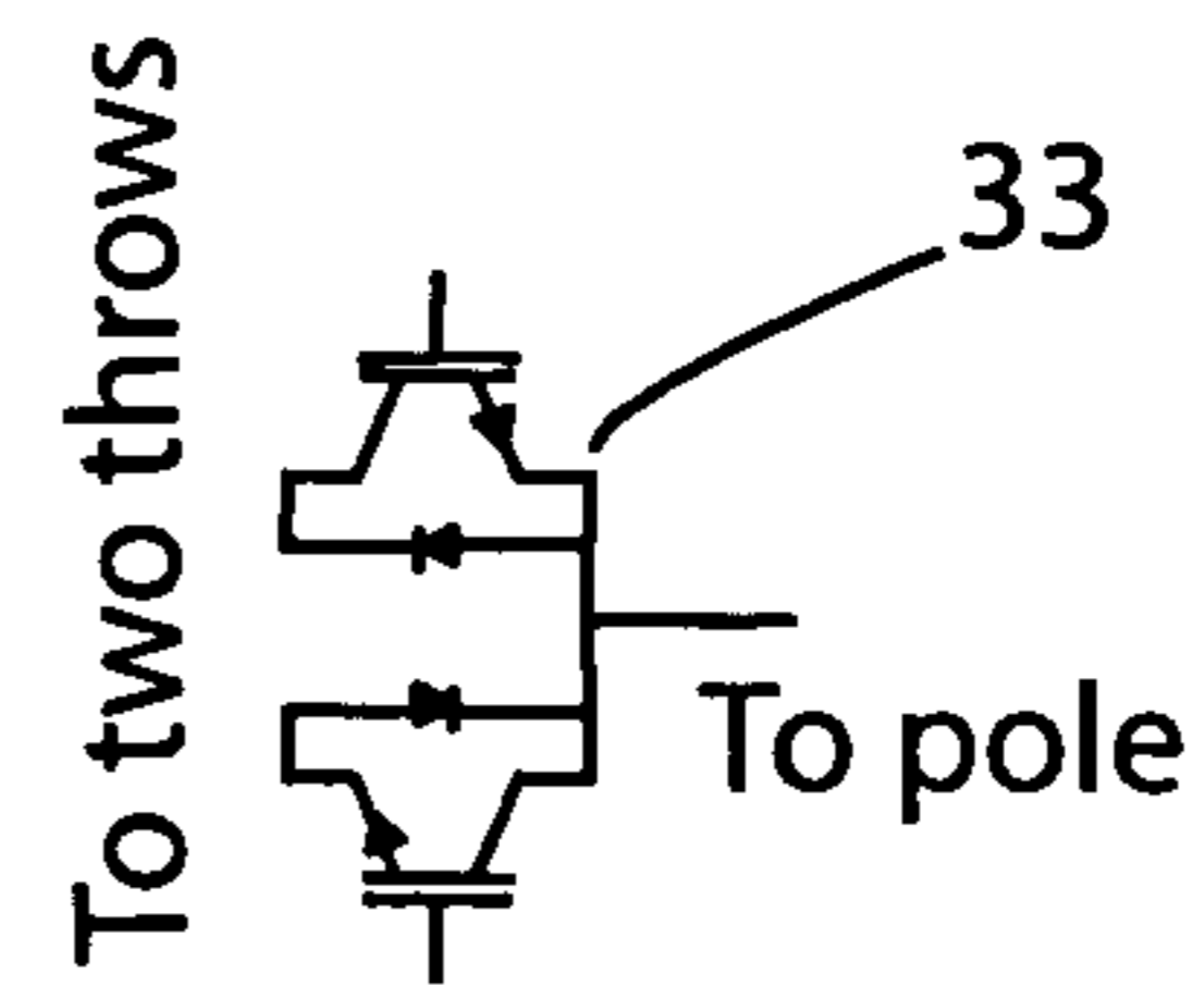
FIG. 4 (prior art)
