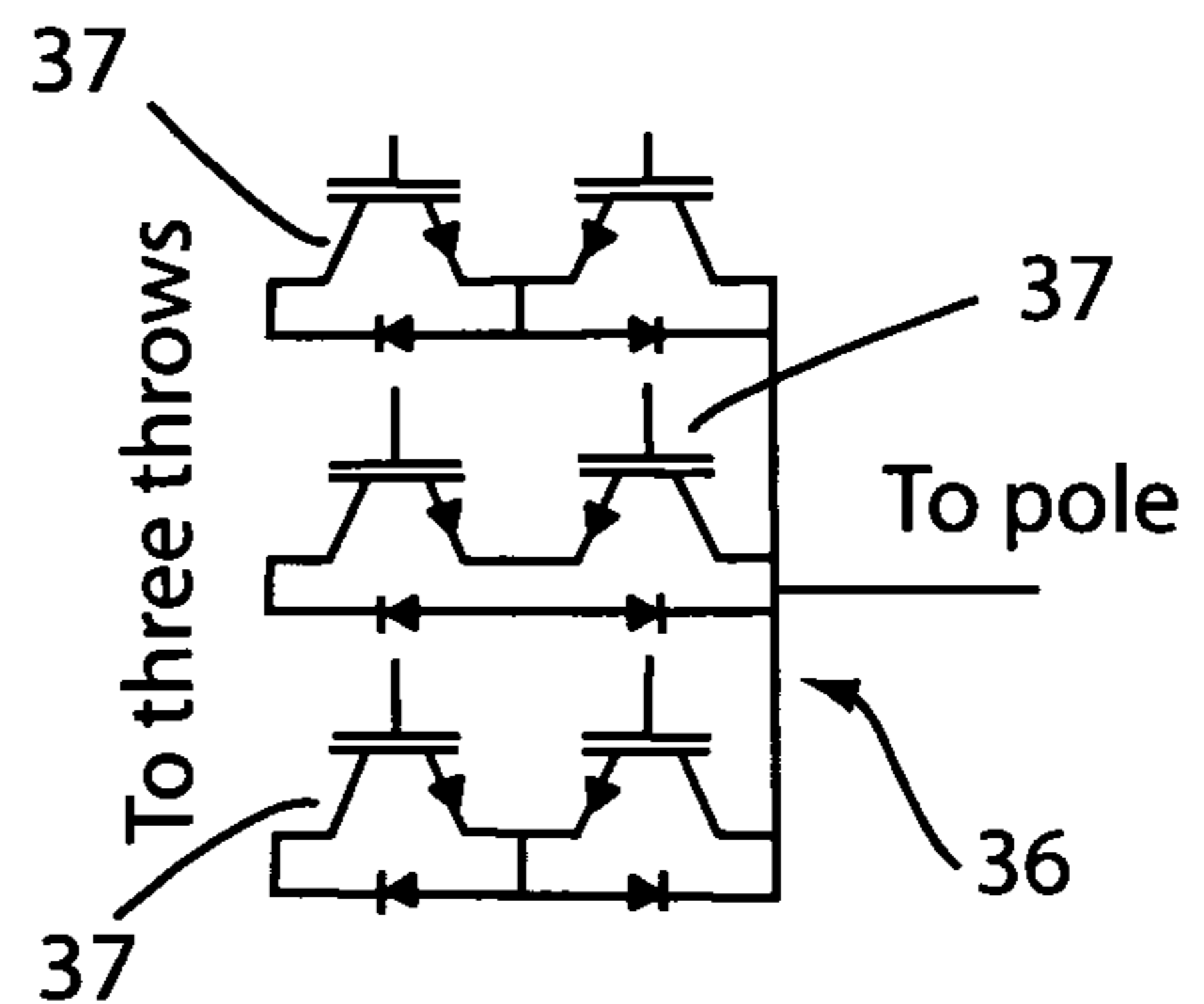
FIG. 6 (prior art)
