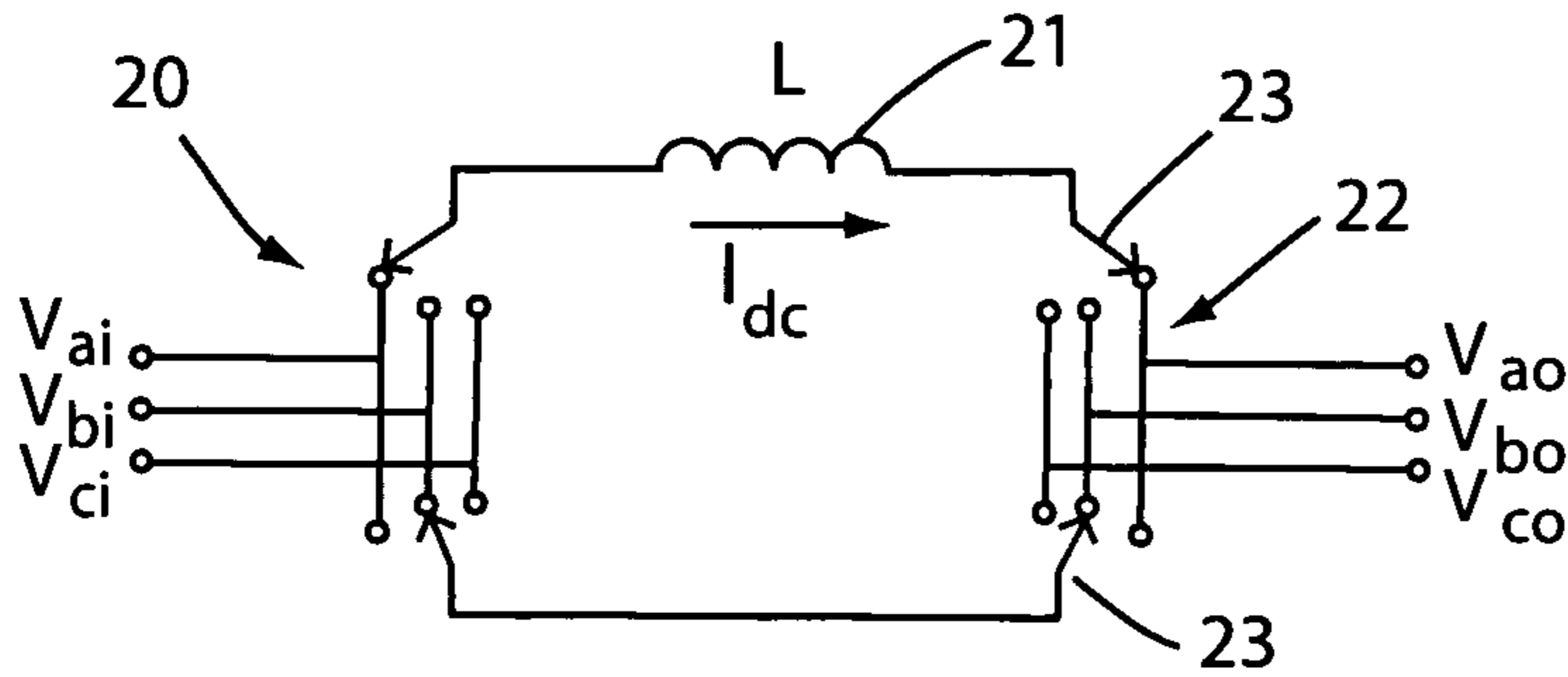
FIG. 1 (prior art)
