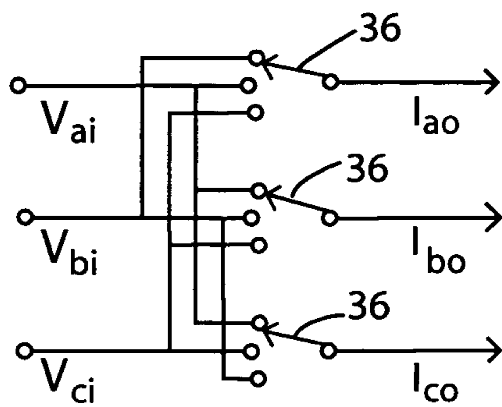
FIG. 5 (prior art)
