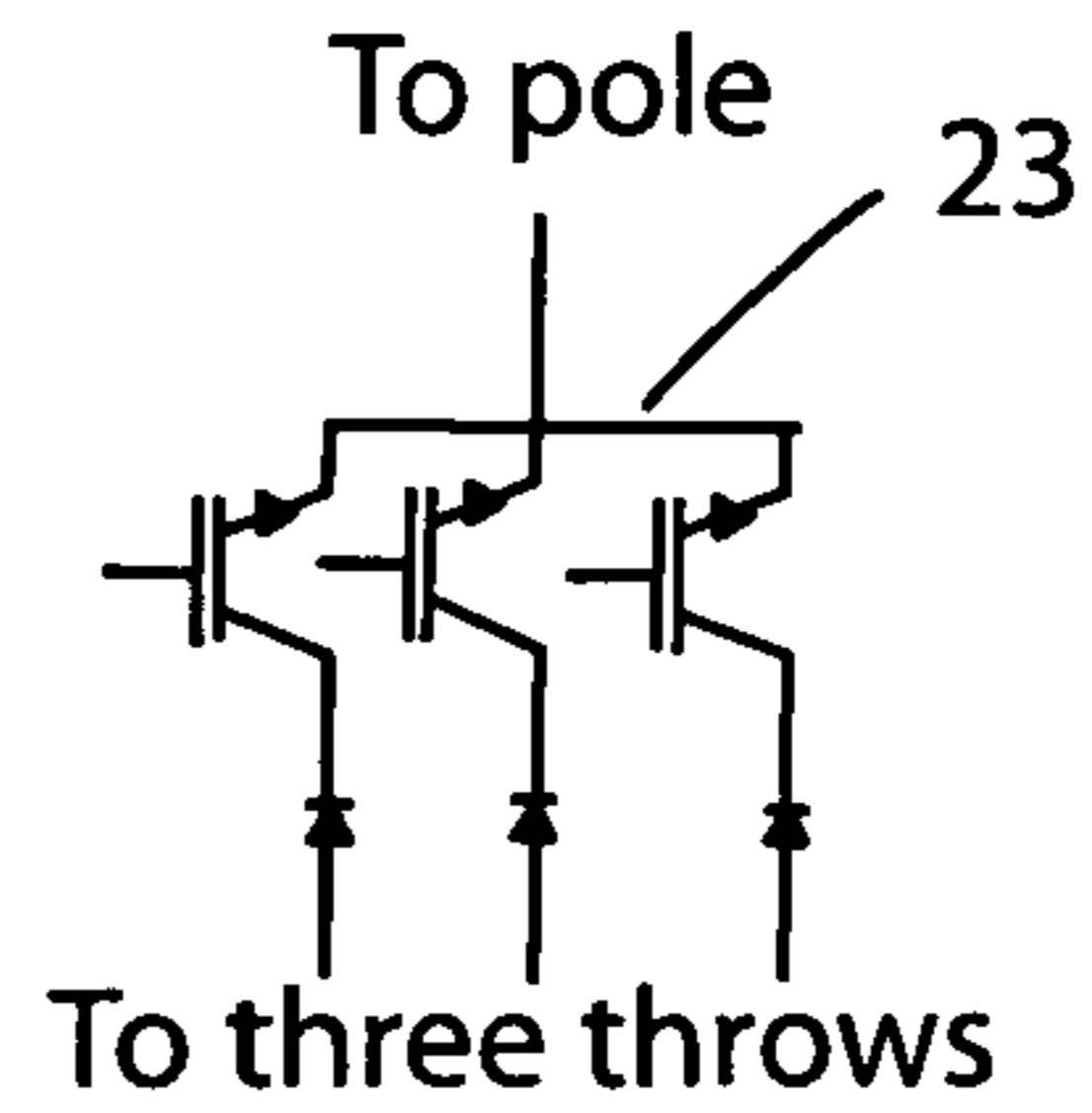
FIG. 2 (prior art)
