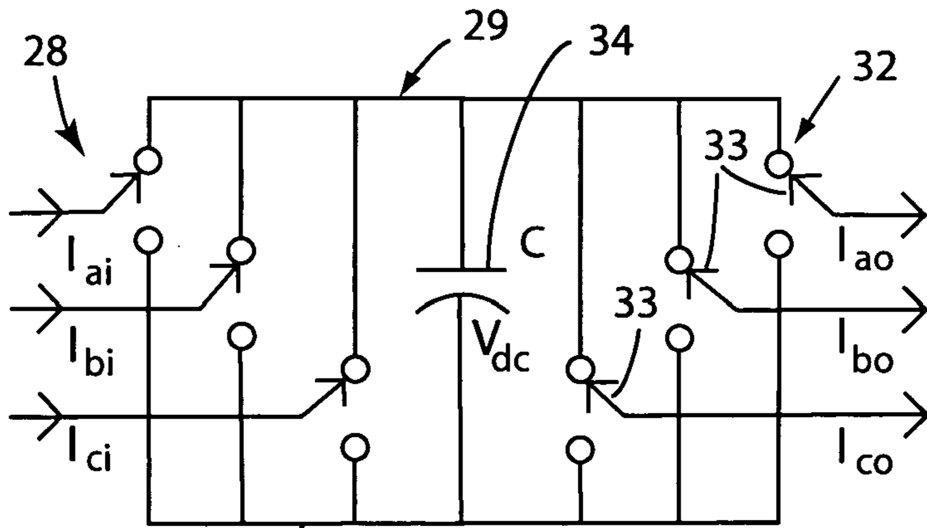
FIG. 1 (prior art)
