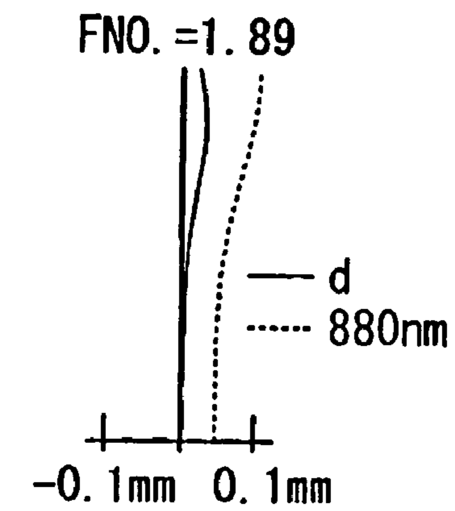
Spherical Aberration Fig. 5A
