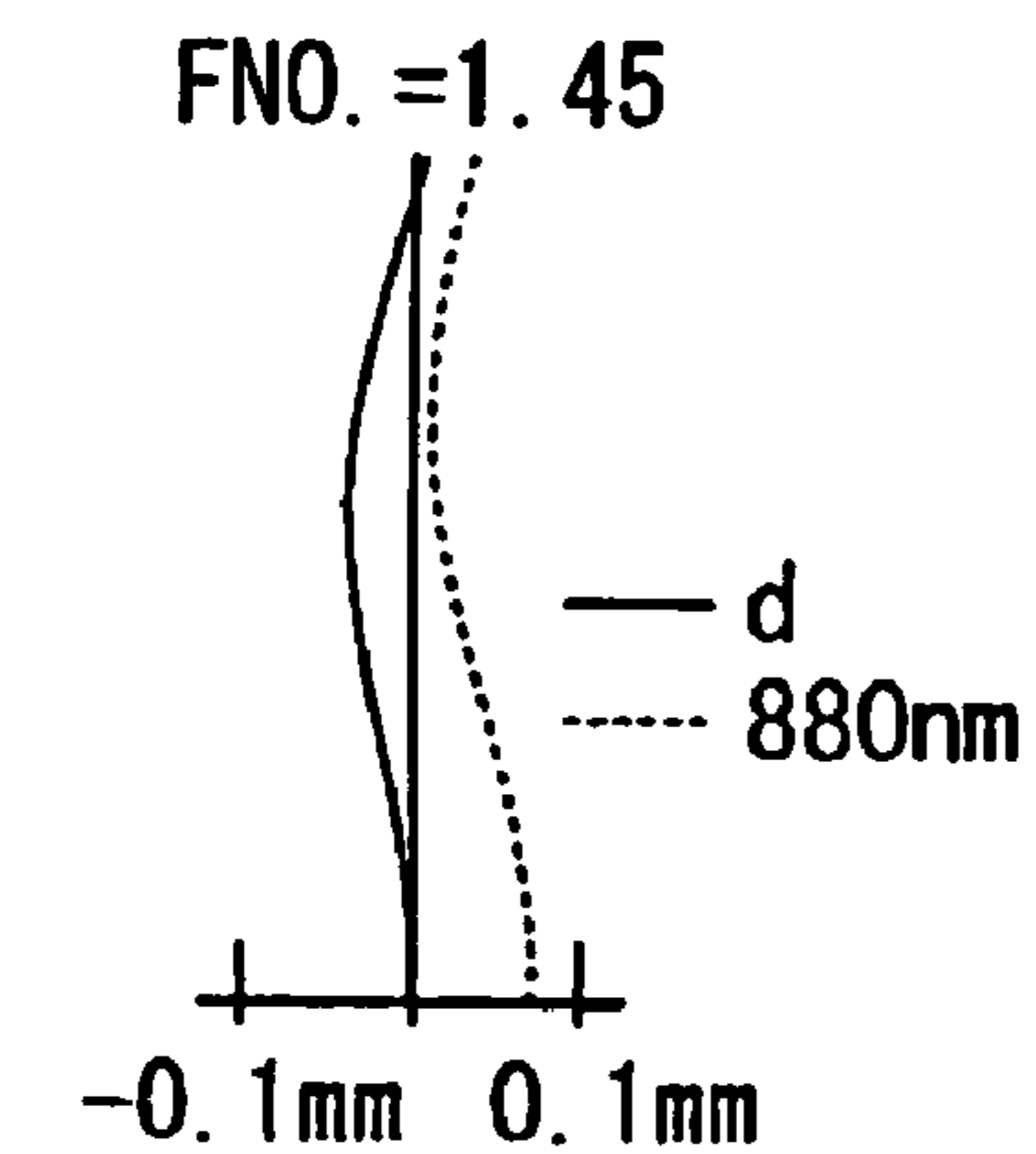
Spherical Aberration Fig. 6A
