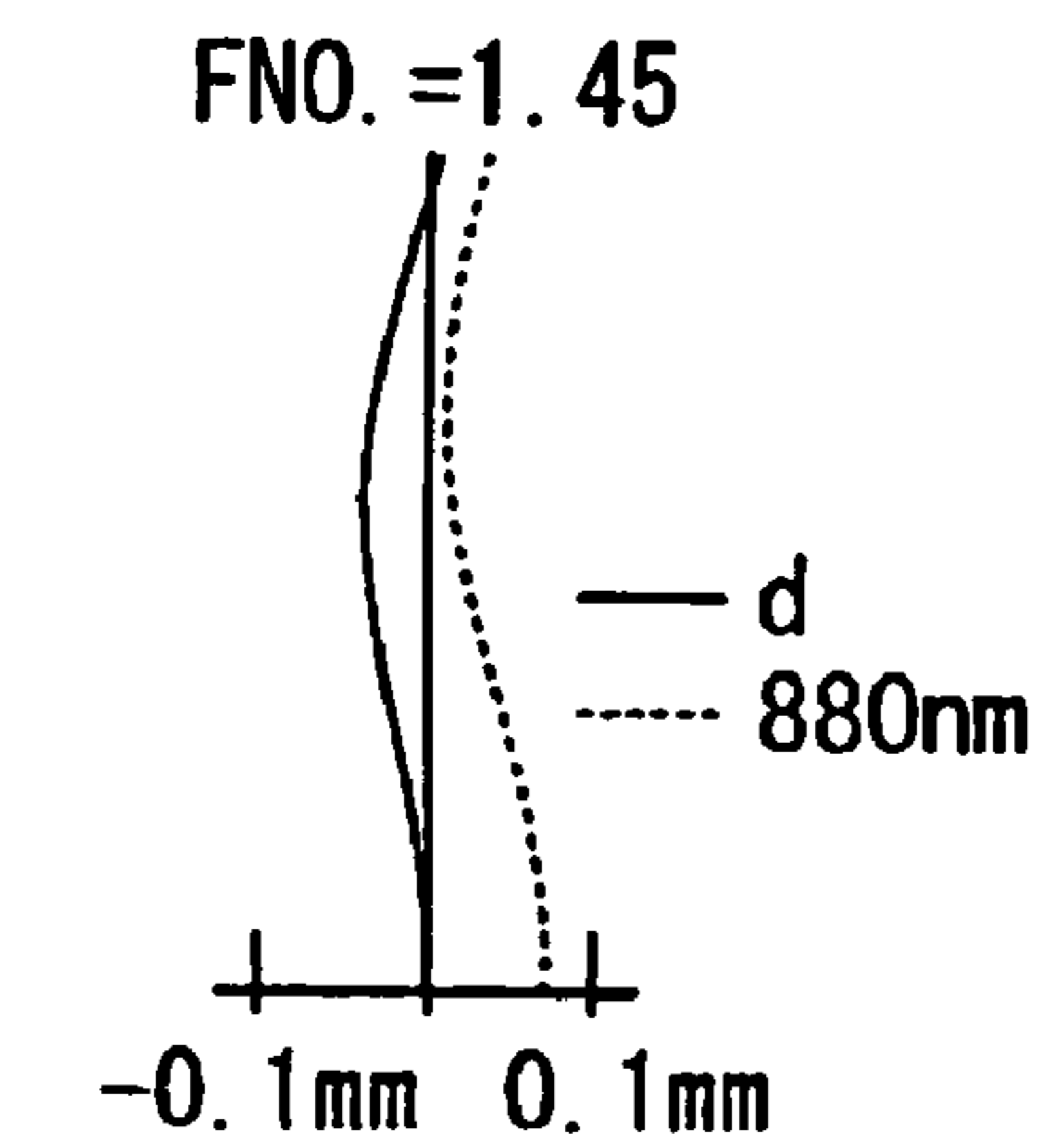
Spherical Aberration Fig. 6A
