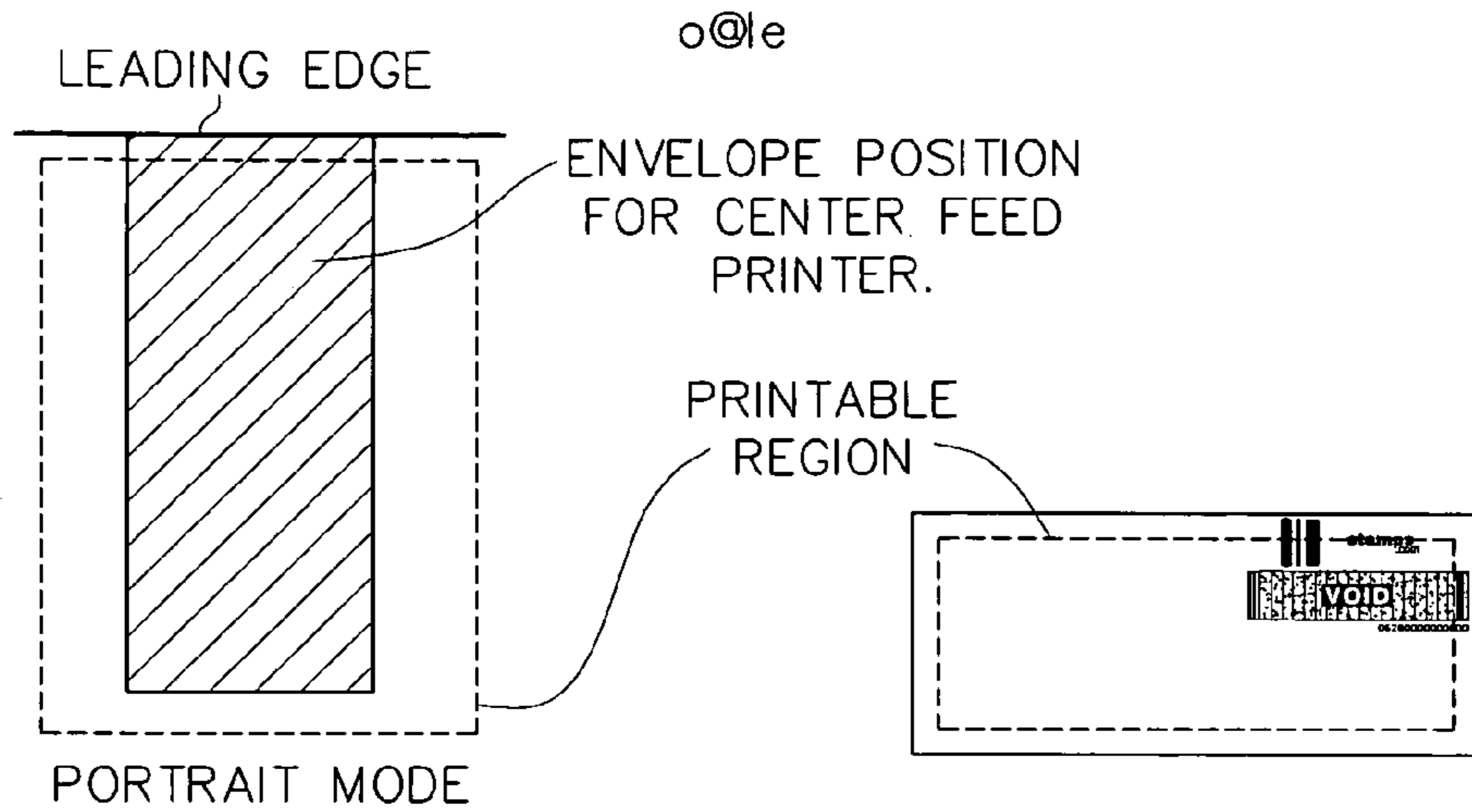
FIG. 22A VIRTUALIZATION PROCESS FOR CENTER-FEED PRINTERS
