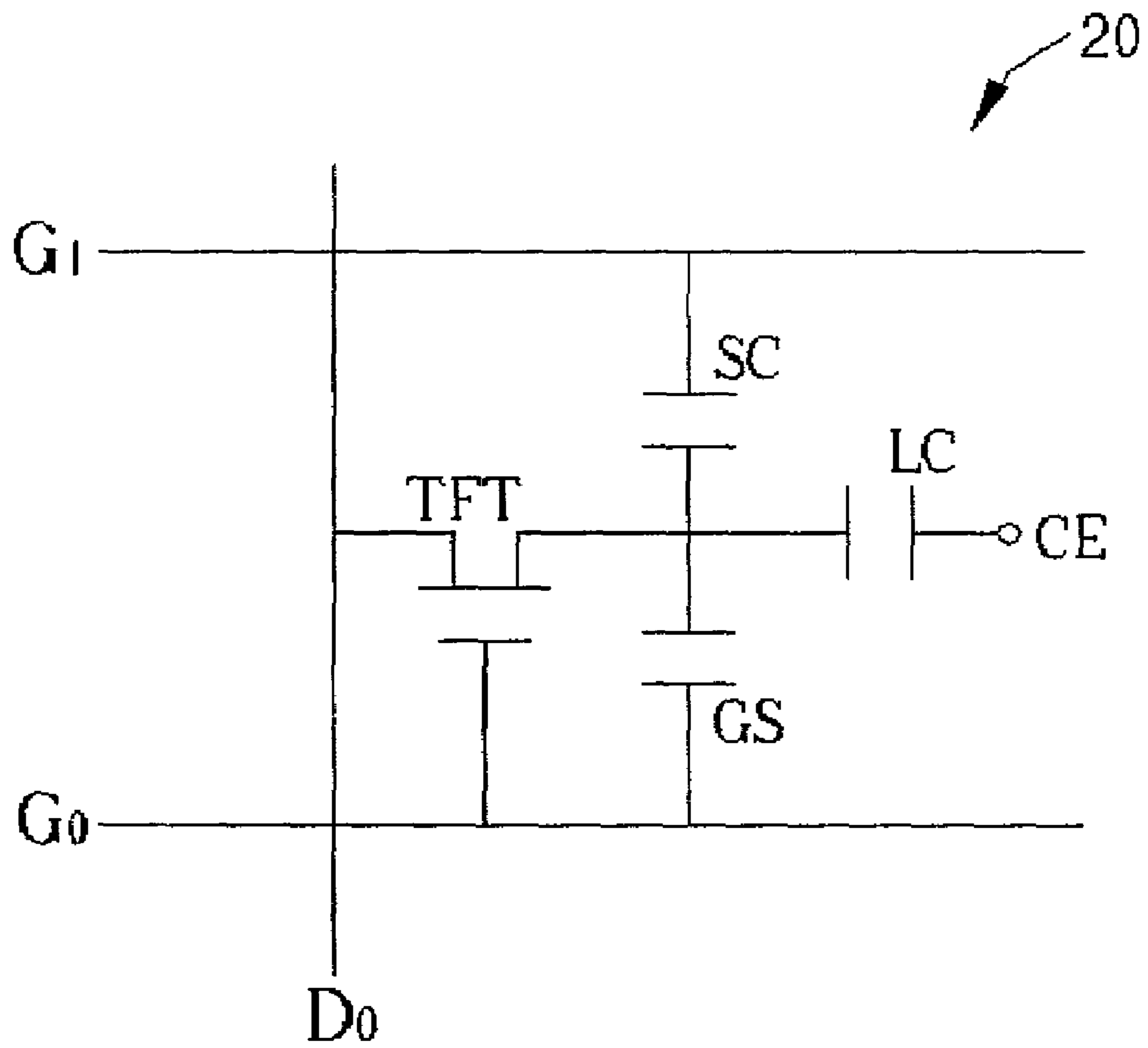
Fig. 2 Prior art
