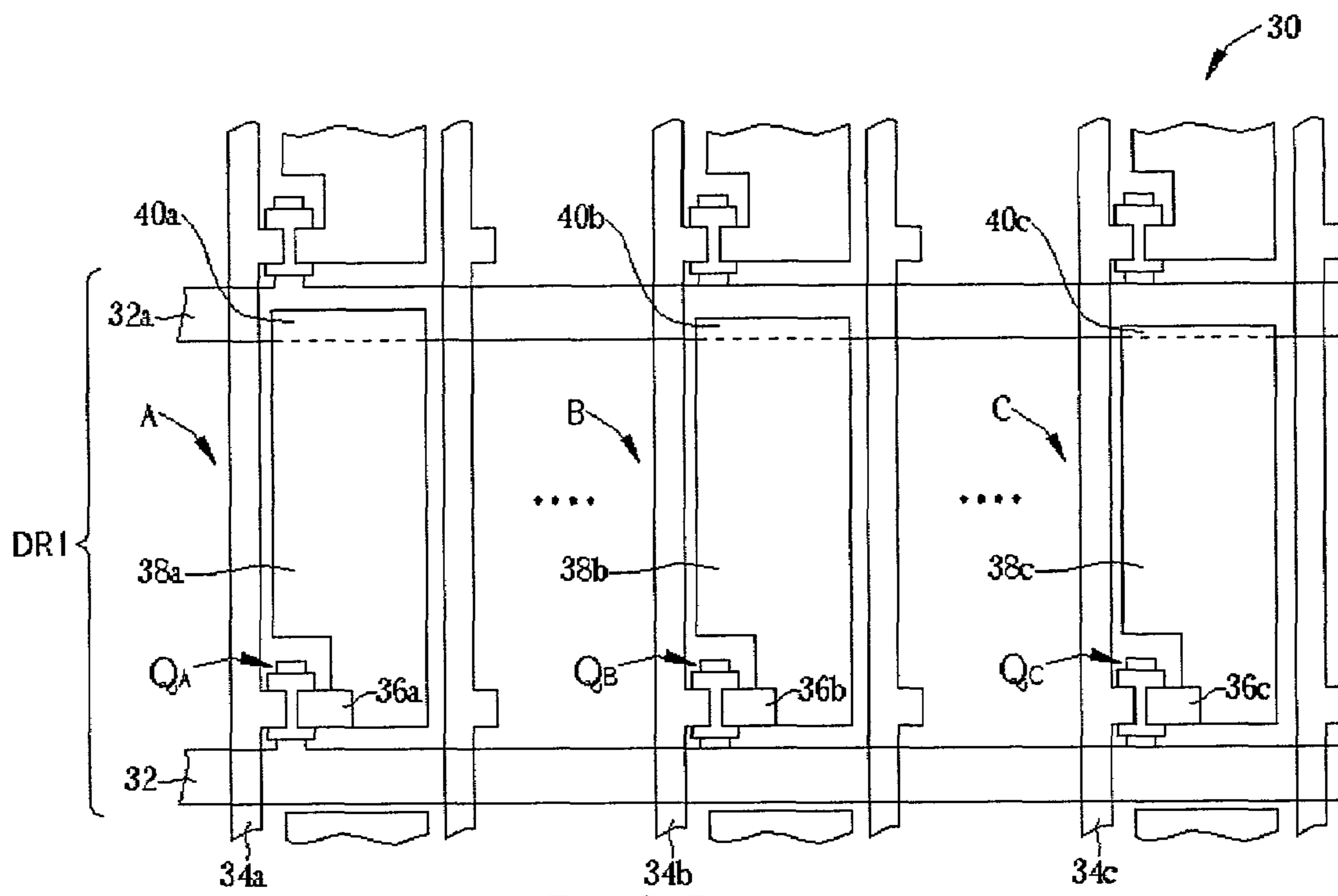
Fig. 3 Prior art
