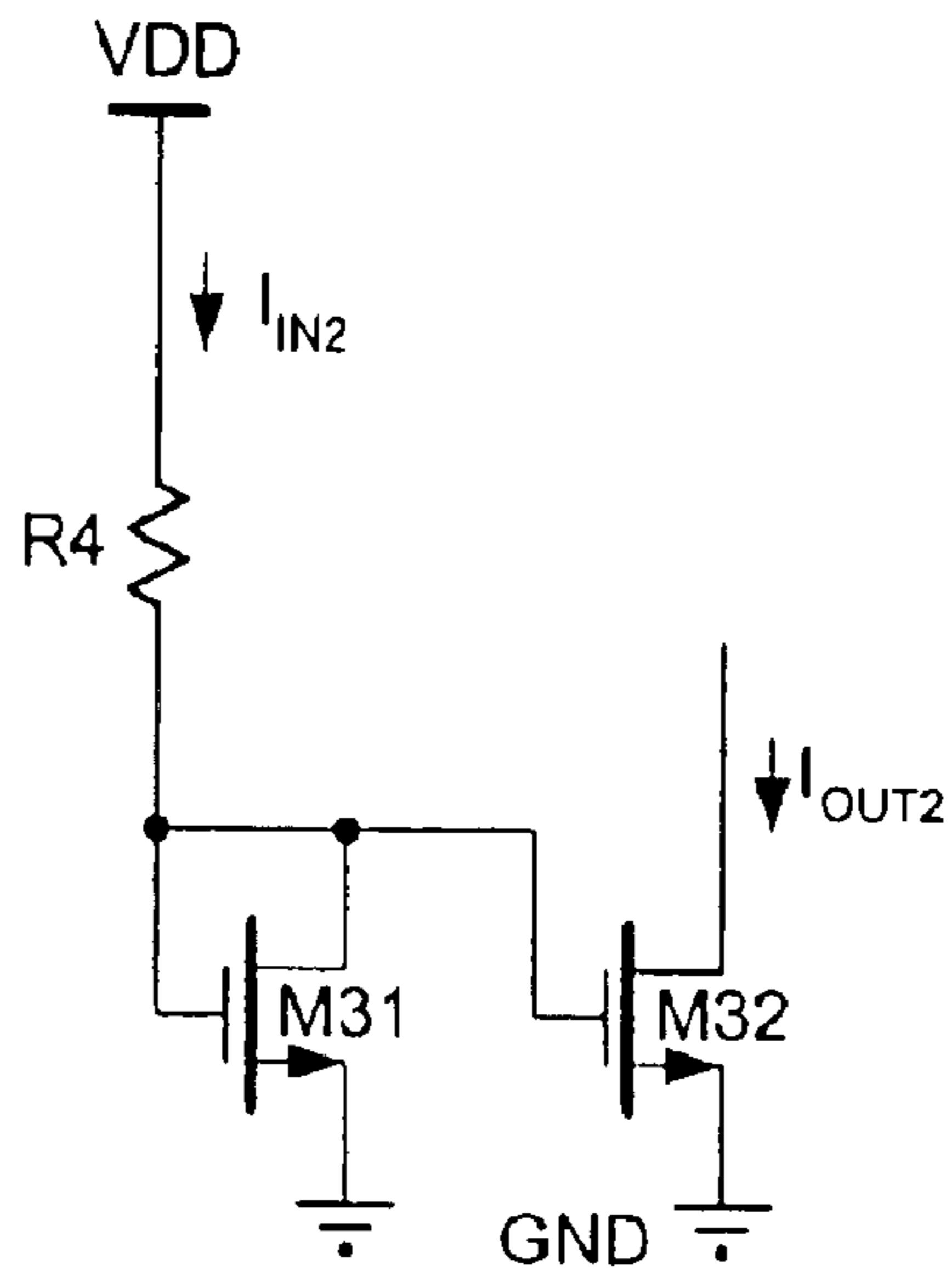
Simple Current Mirror FIG. 7A (Prior Art)
