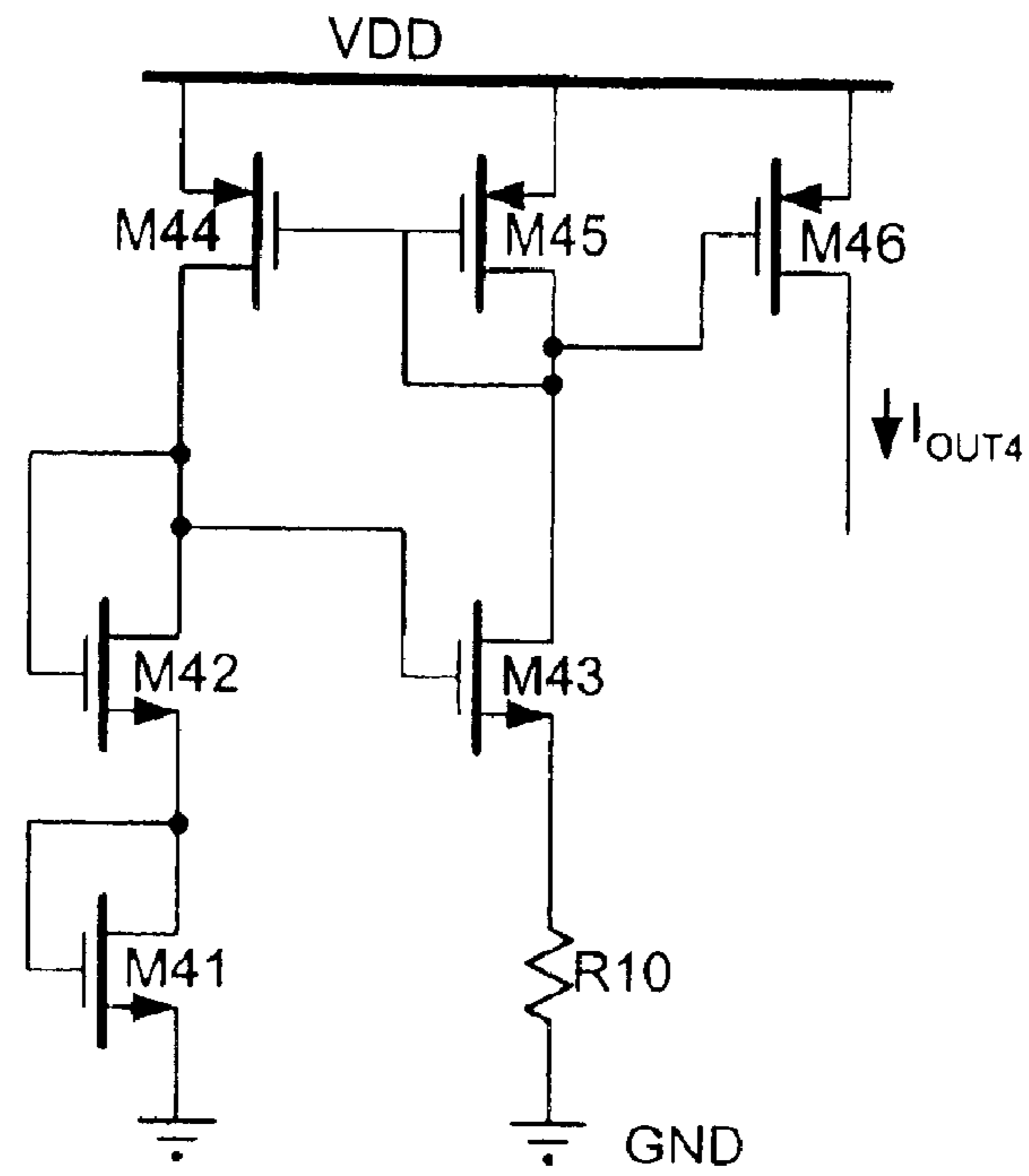
Self-Biased Current Mirror With Resistor FIG. 7C (Prior Art)
