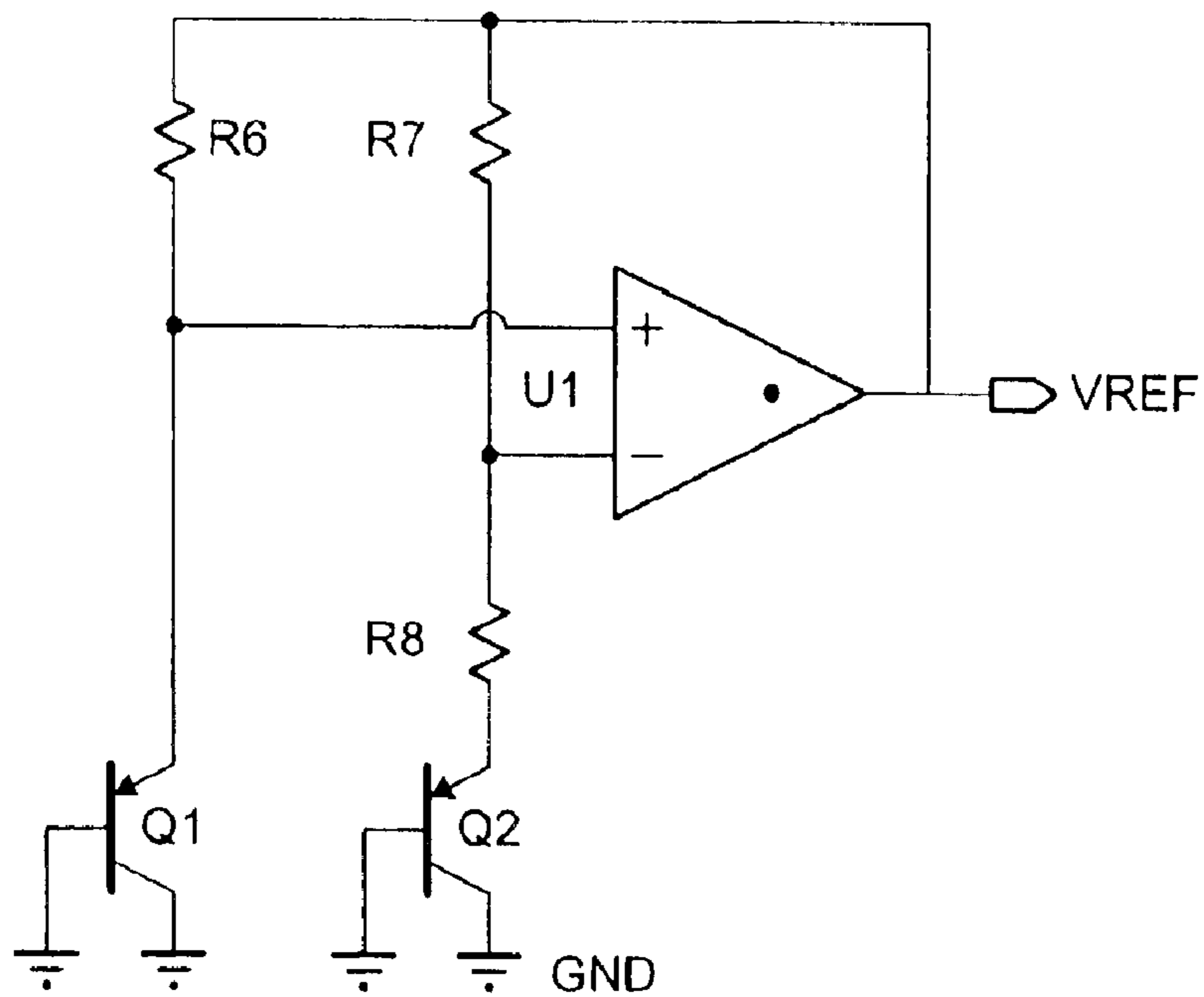
Bandgap Voltage Reference FIG. 7D (Prior Art)
