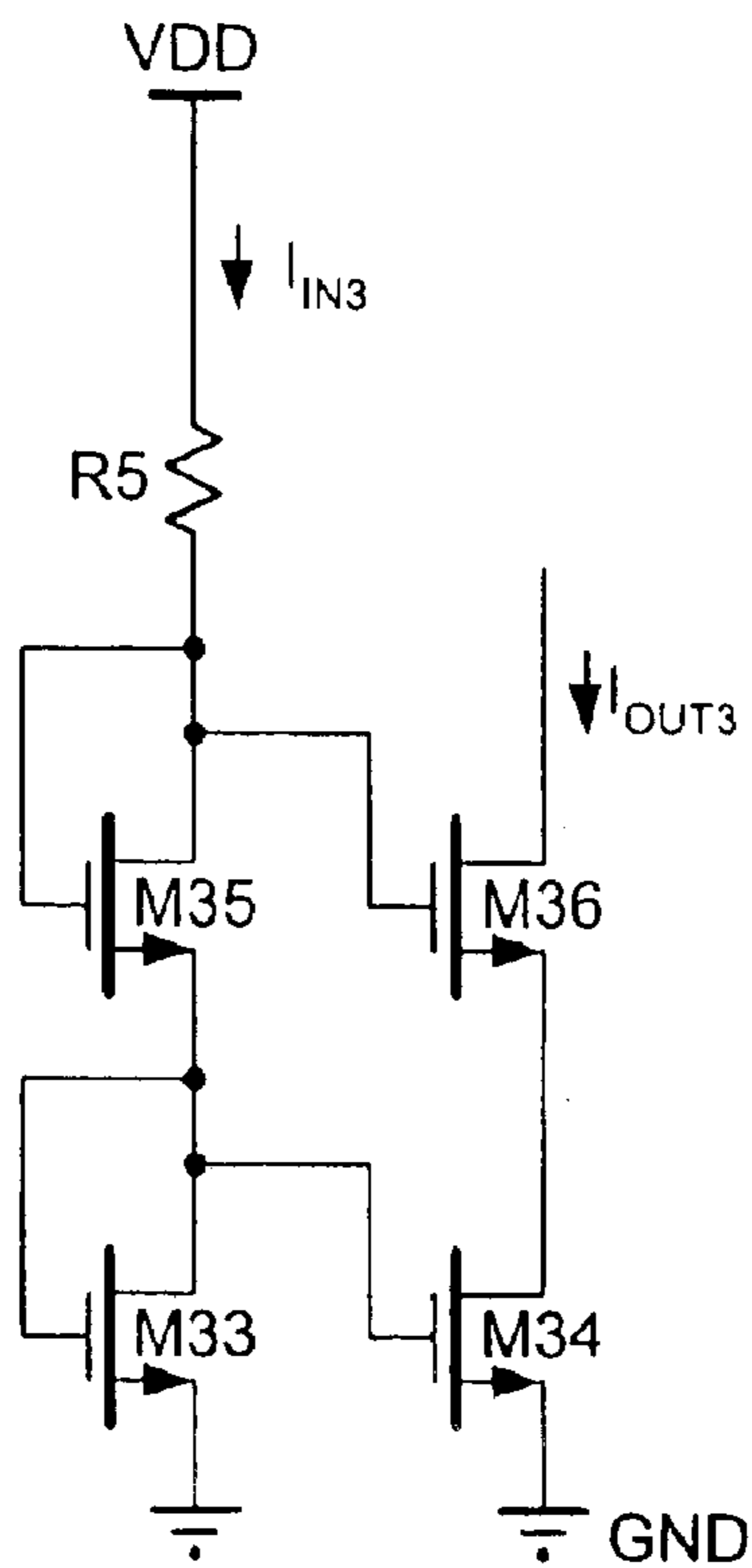
Cascode Current Mirror FIG. 7B (Prior Art)
