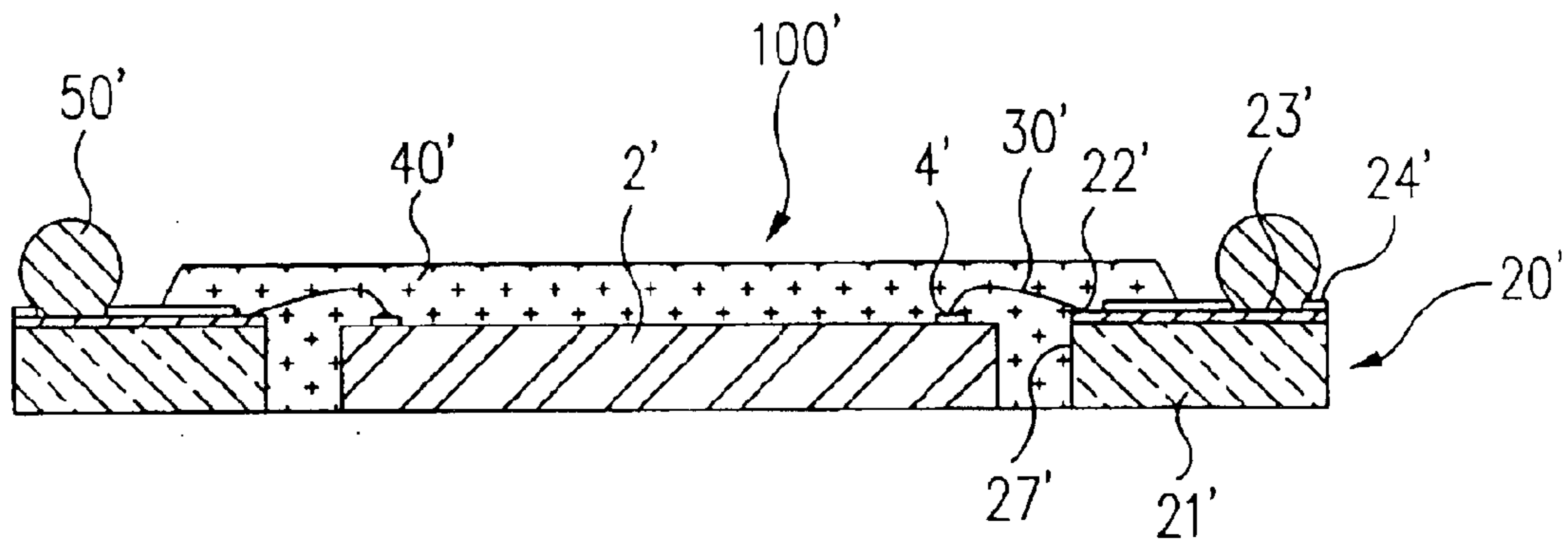
FIG. 7 (PRIOR ART)
