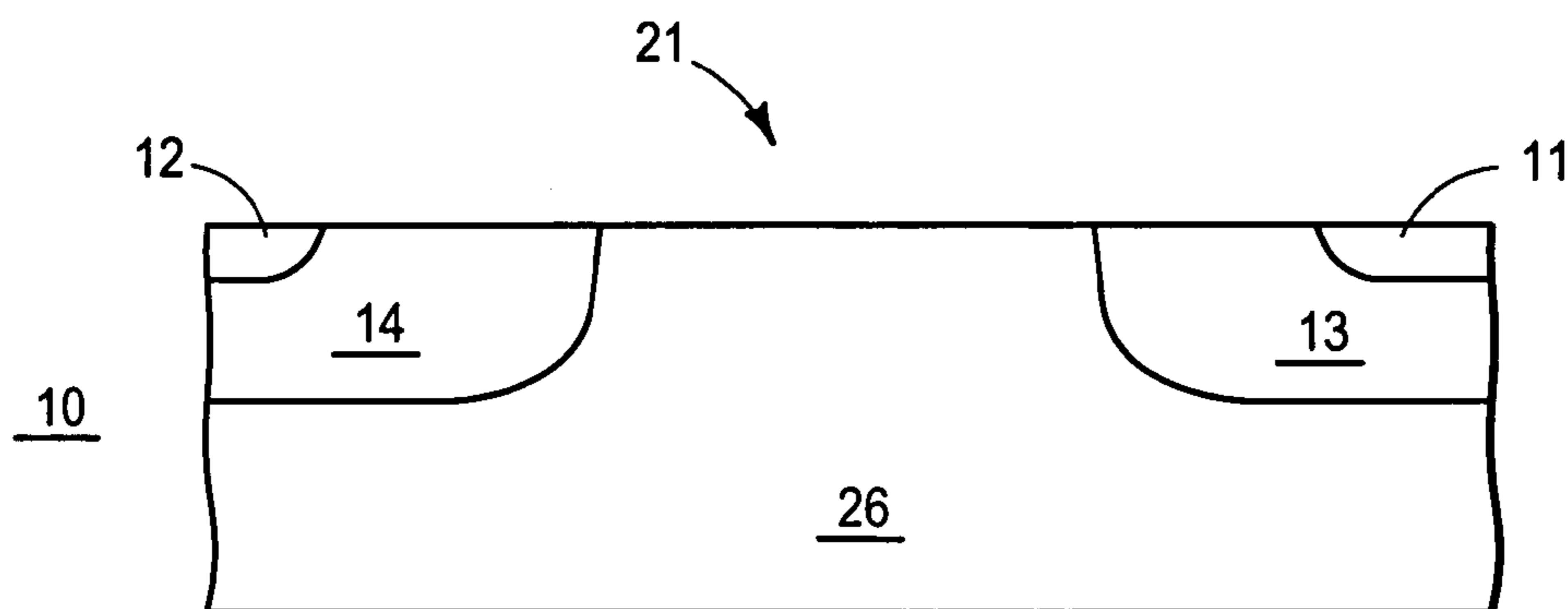
FIG. 2 Prior Art
