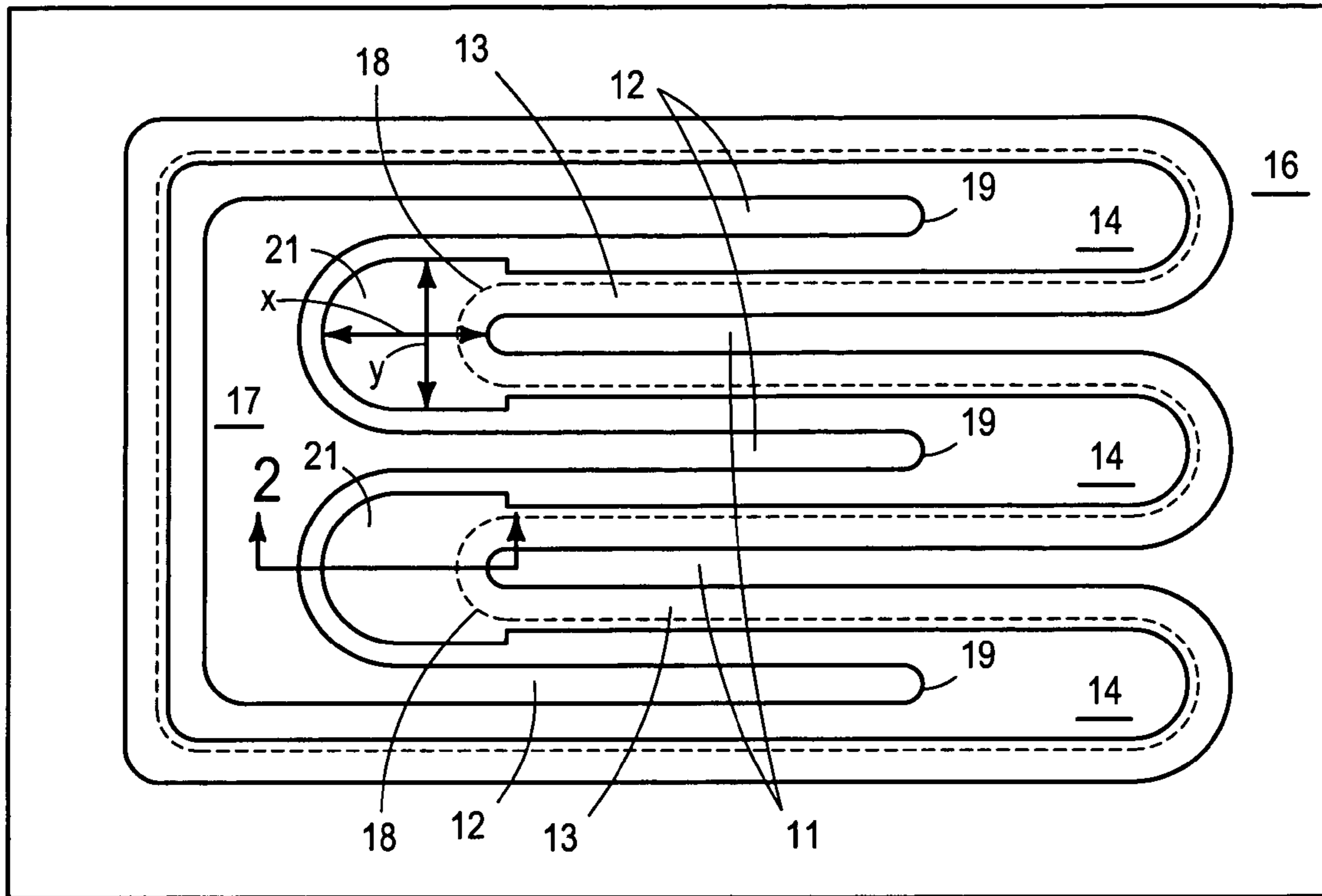
FIG. 1 Prior Art
