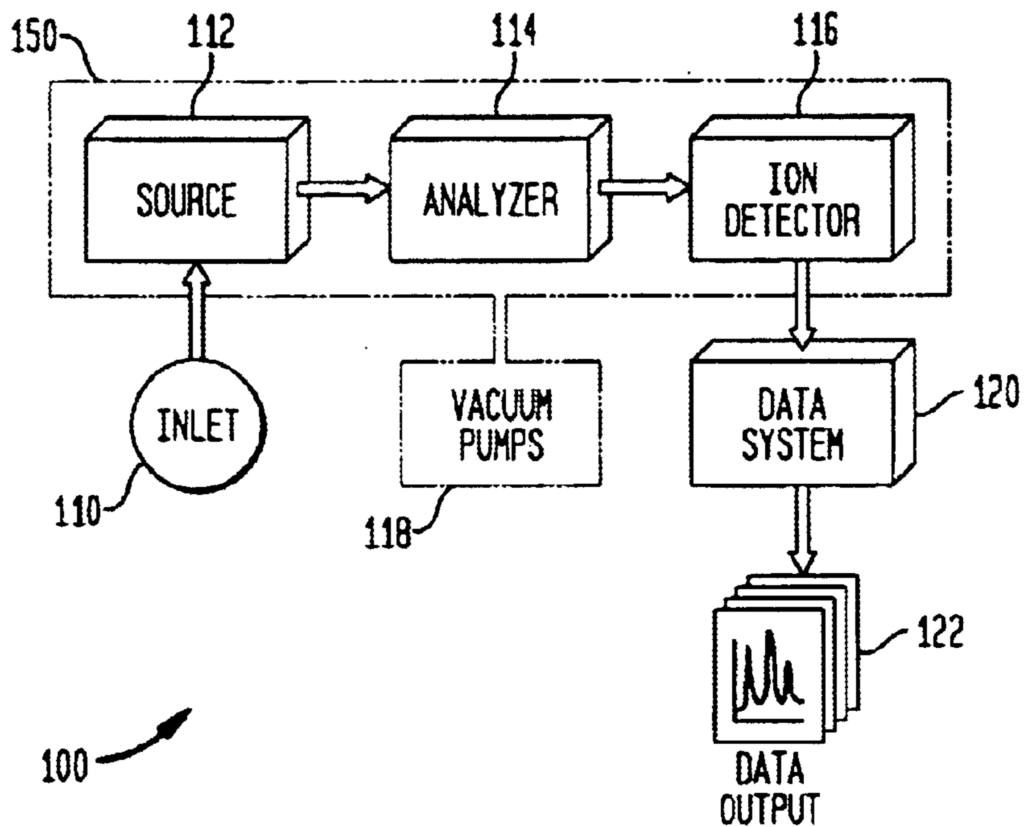
FIG. 2 (PRIOR ART)
