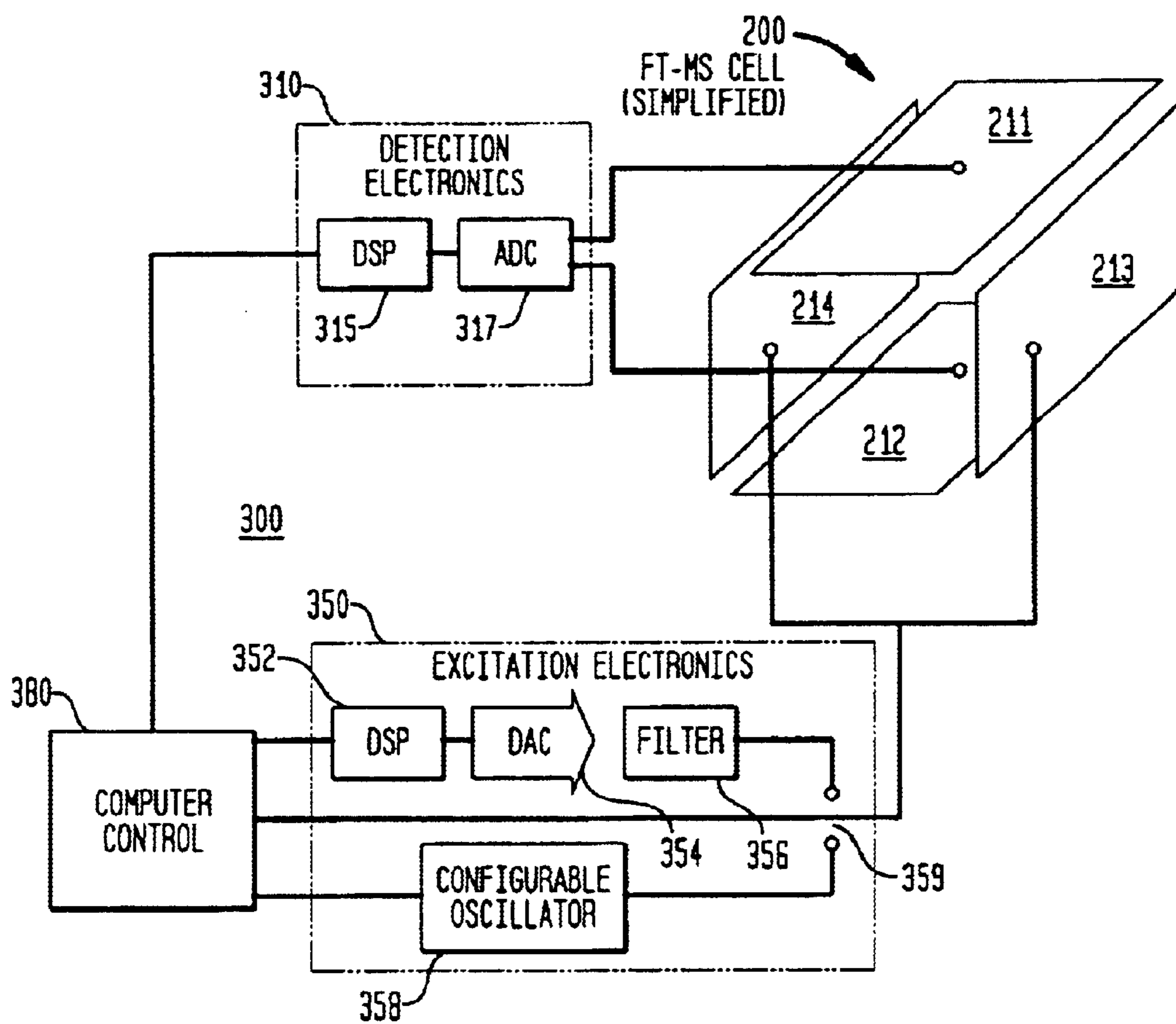
FIG. 3 (PRIOR ART)
