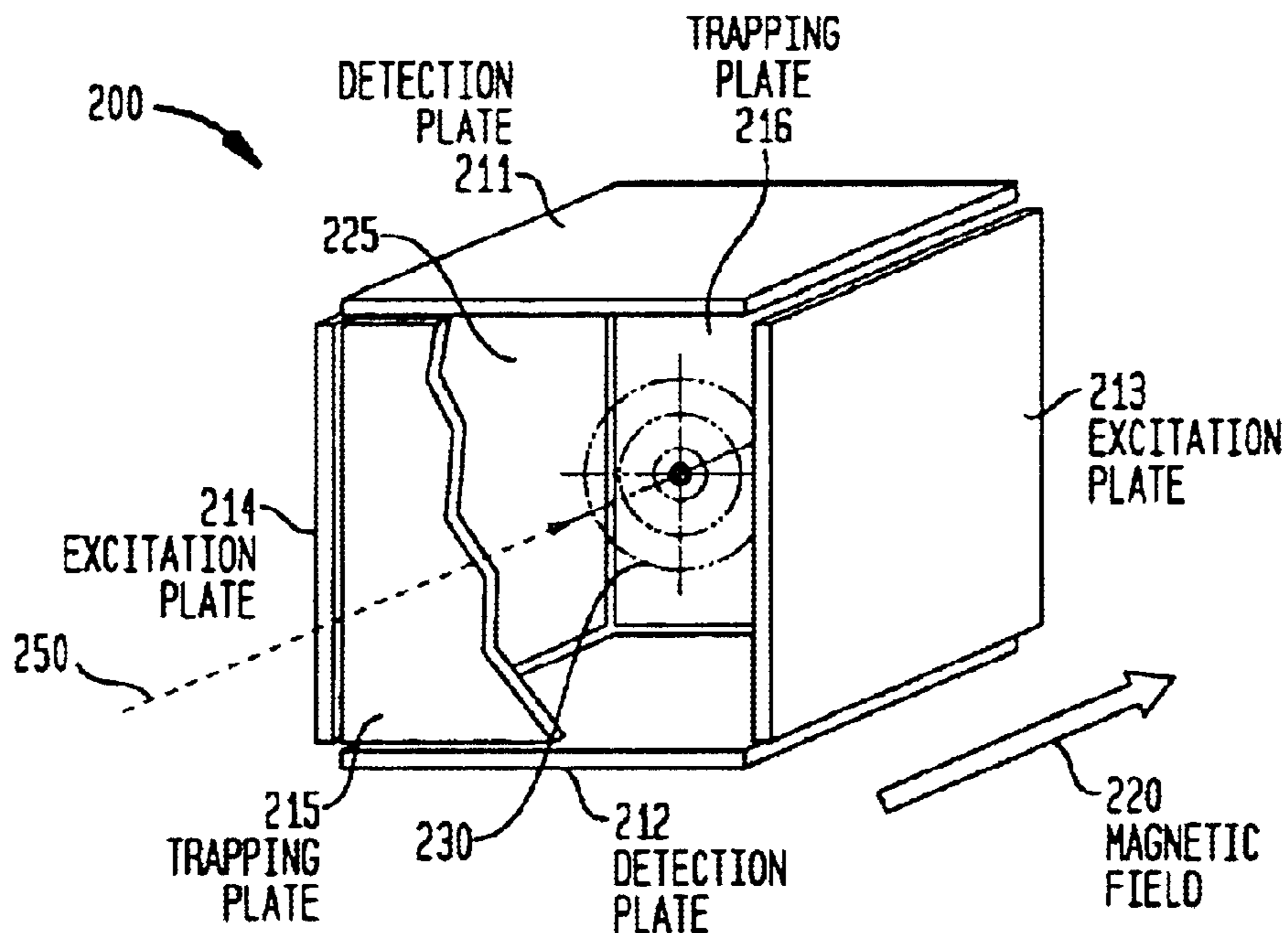
FIG. 2 (PRIOR ART)
