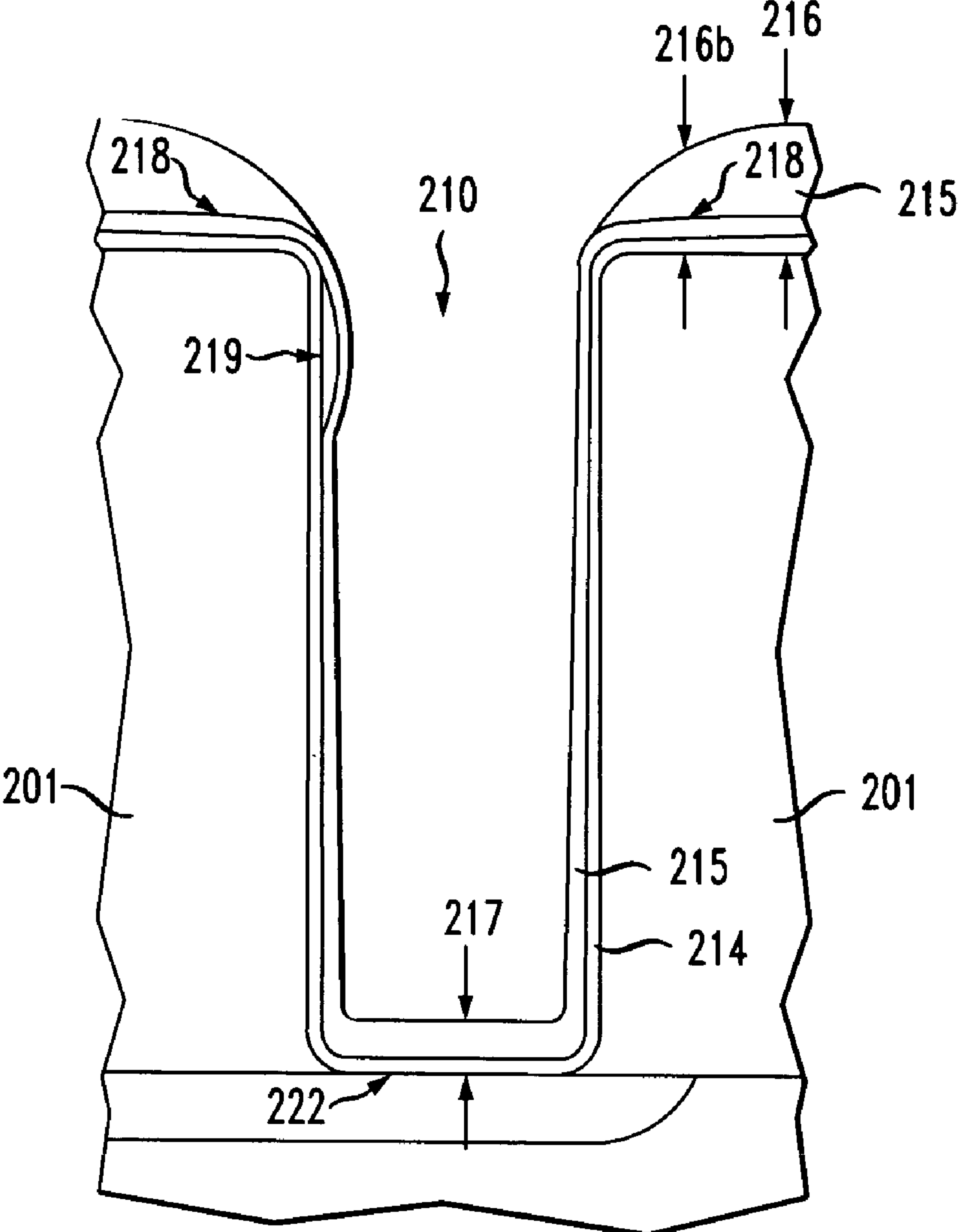
FIG. 2 (PRIOR ART)
