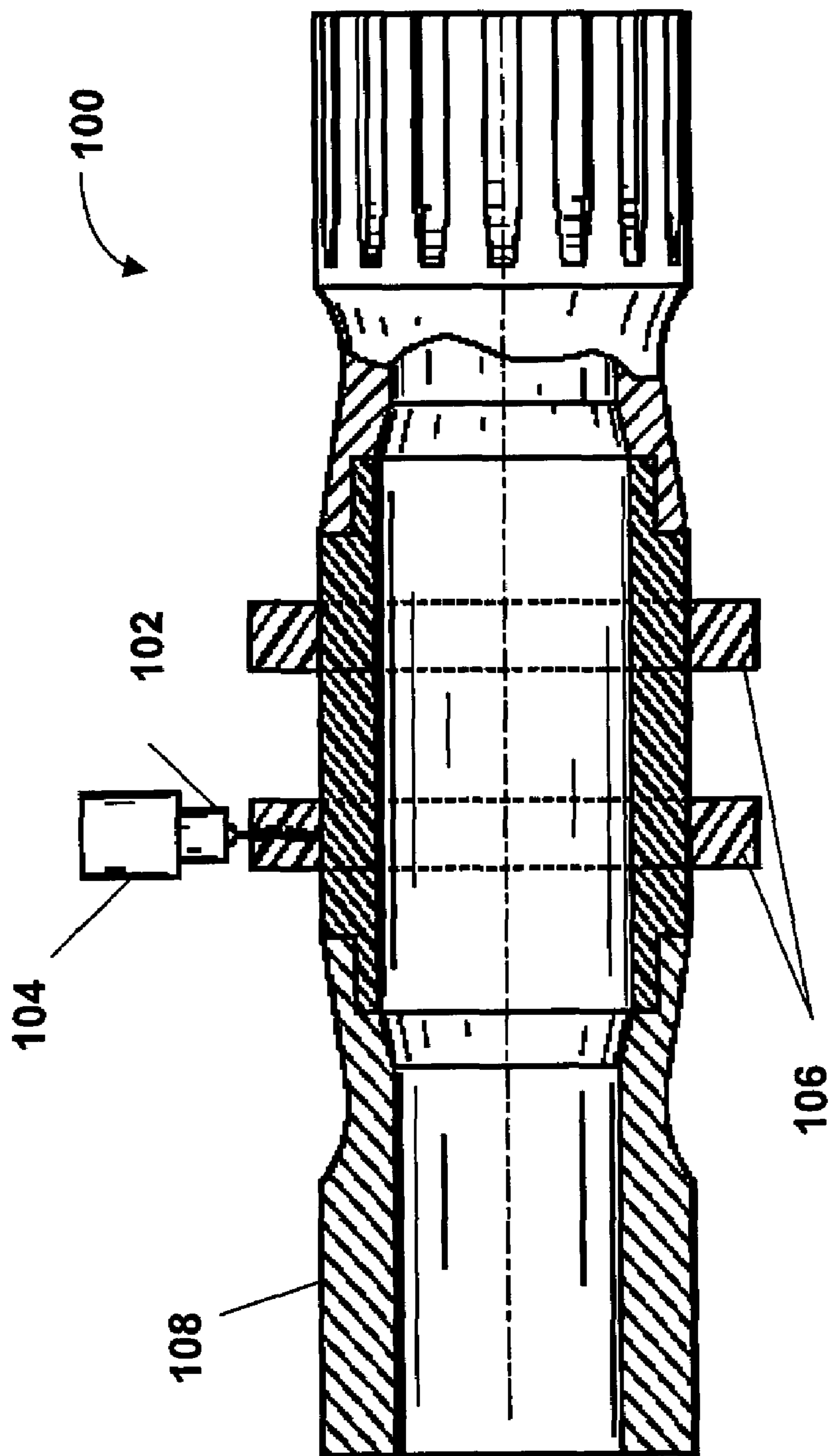
FIG. 1 (PRIOR ART)
