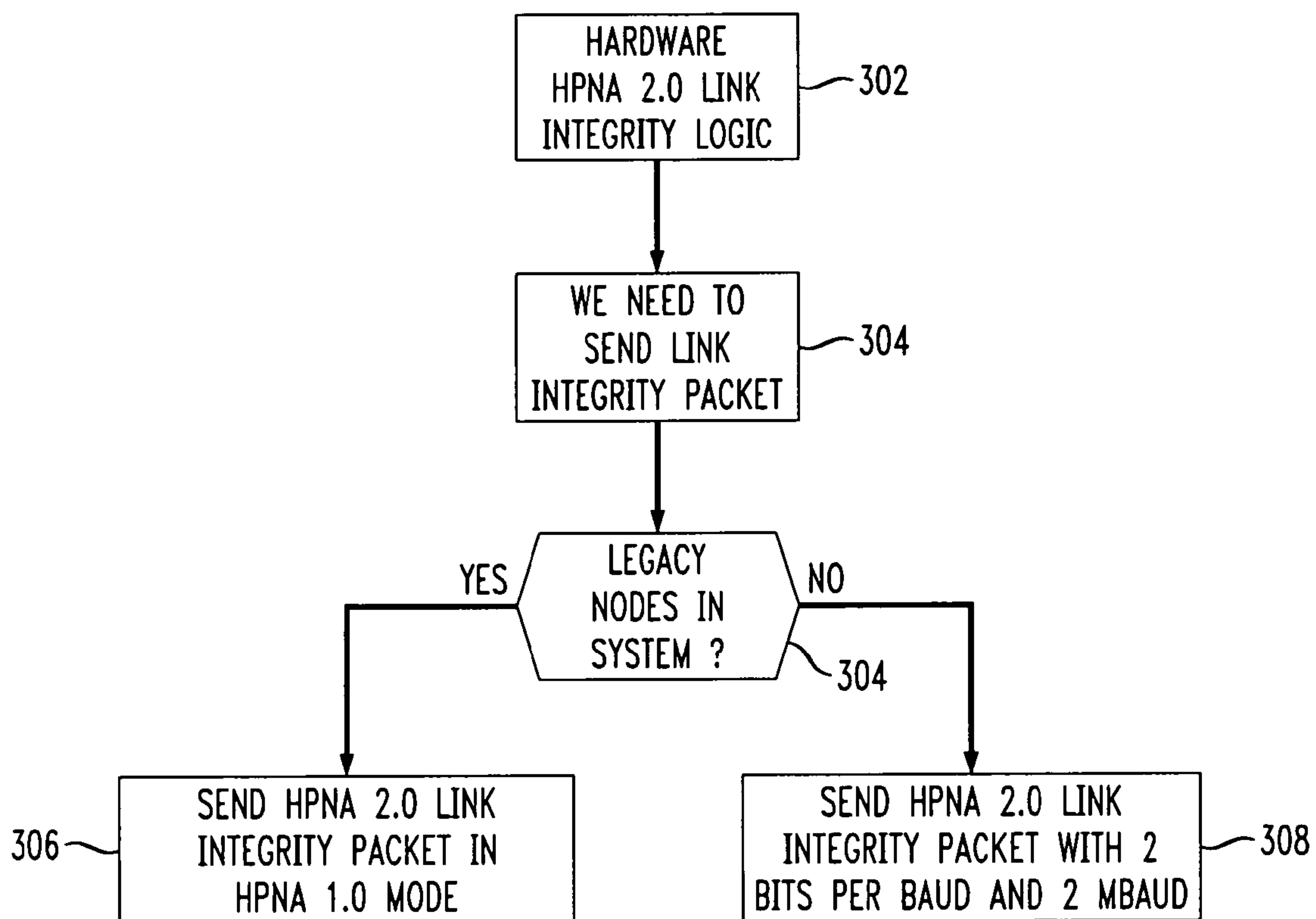
TRANSMITTER BEHAVIOR STATE FLOW DIAGRAM
