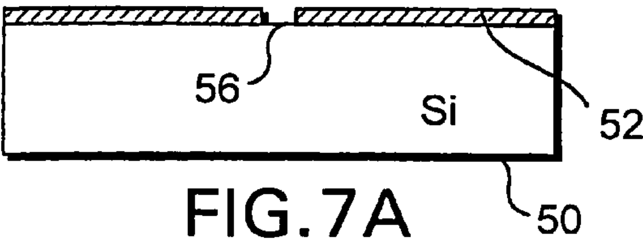
STEP 3. REMOVE DOT PATTERN MASK
