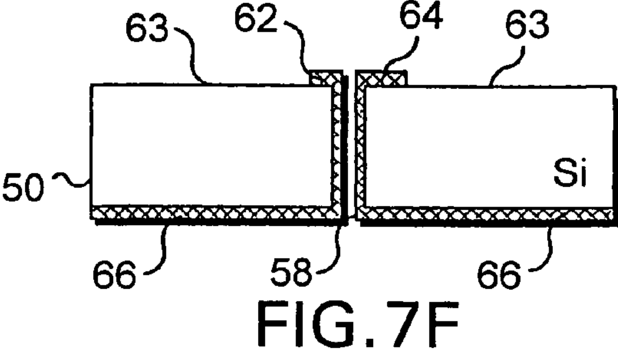
STEP 6. REMOVE NITRIDE PATTERN MASK
