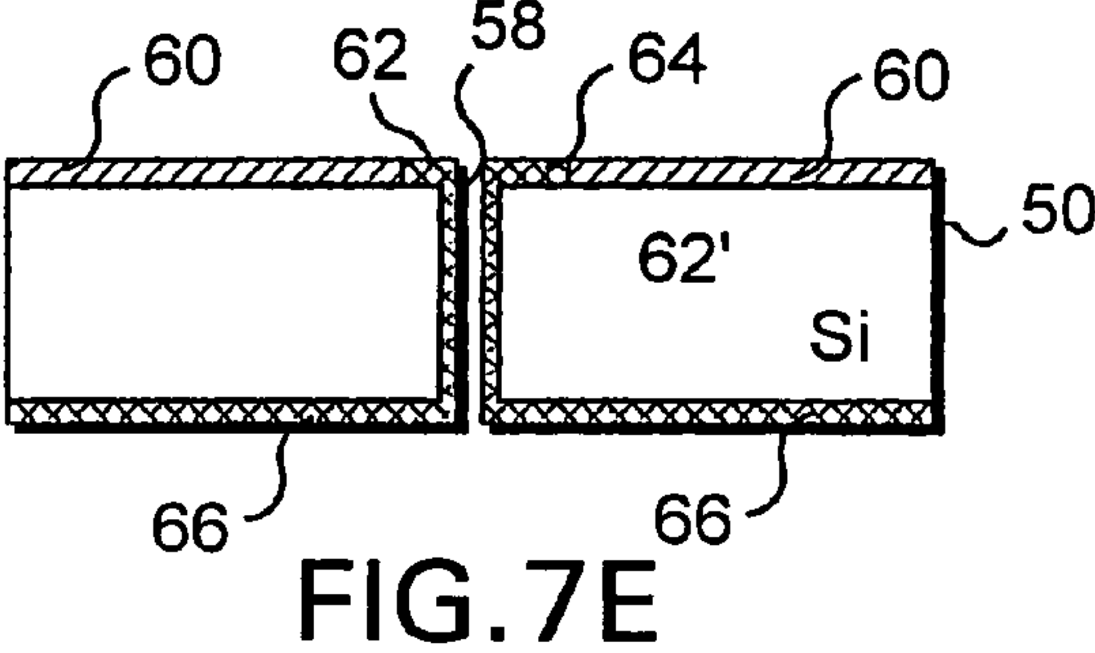
STEP 5. GROW NITRIDE LAYER
