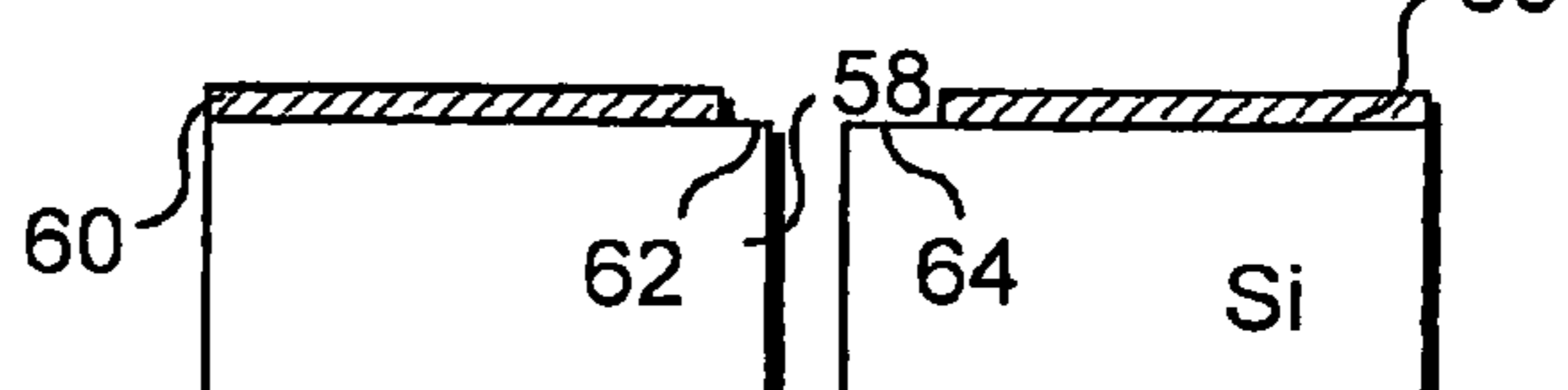
STEP 4. FORM NITRIDE PATTERN MASK
