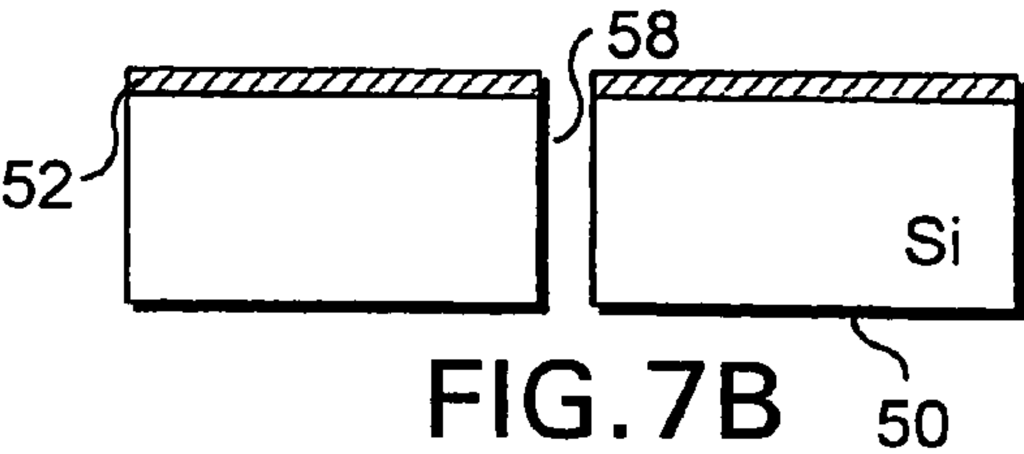
STEP 4. FORM NITRIDE PATTERN MASK
