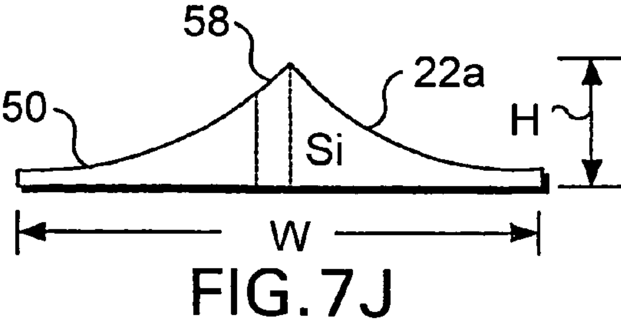
FINISHED MICRO-NEEDLE
