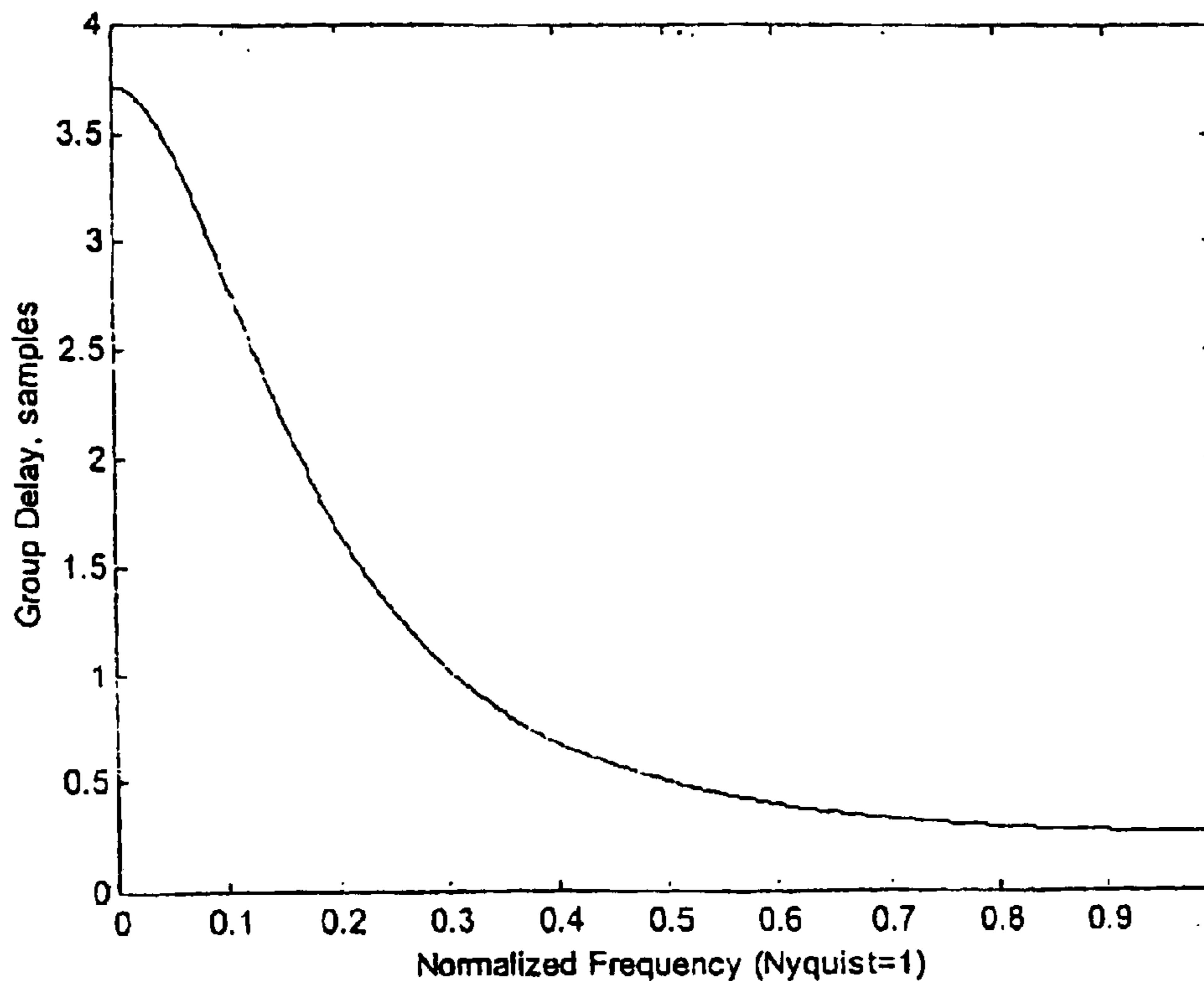
FIG. 4 (PRIOR ART)
