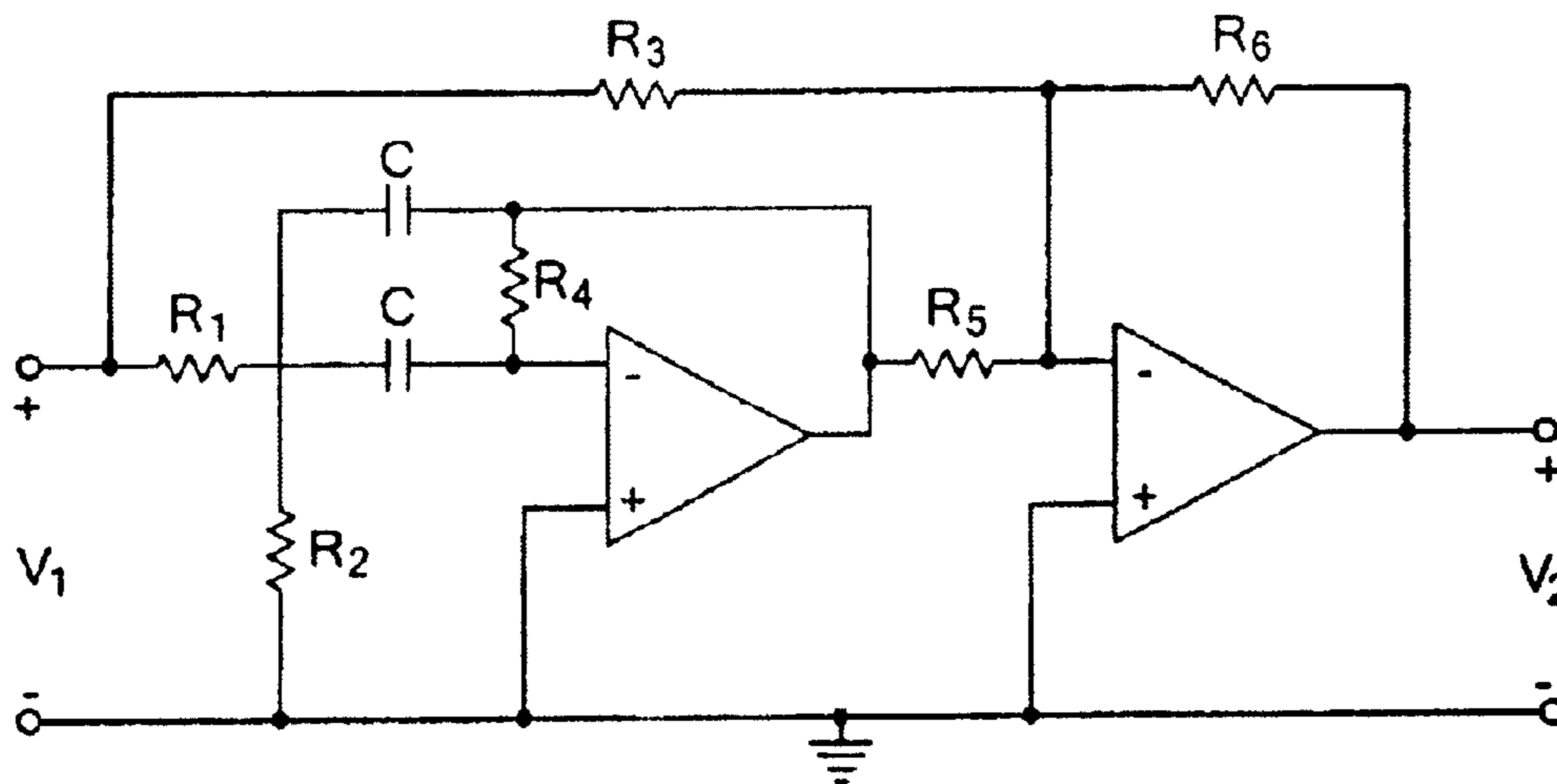
A band-reject filter
