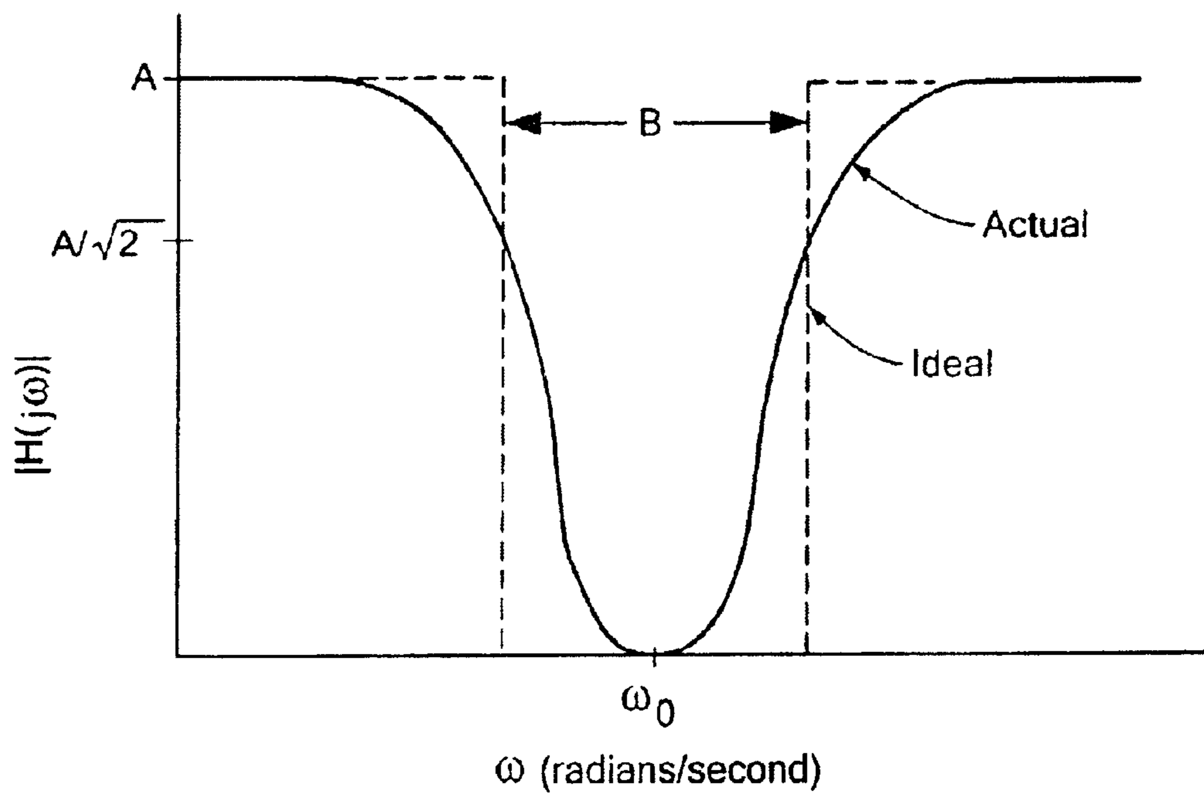
A band-reject amplitude response
