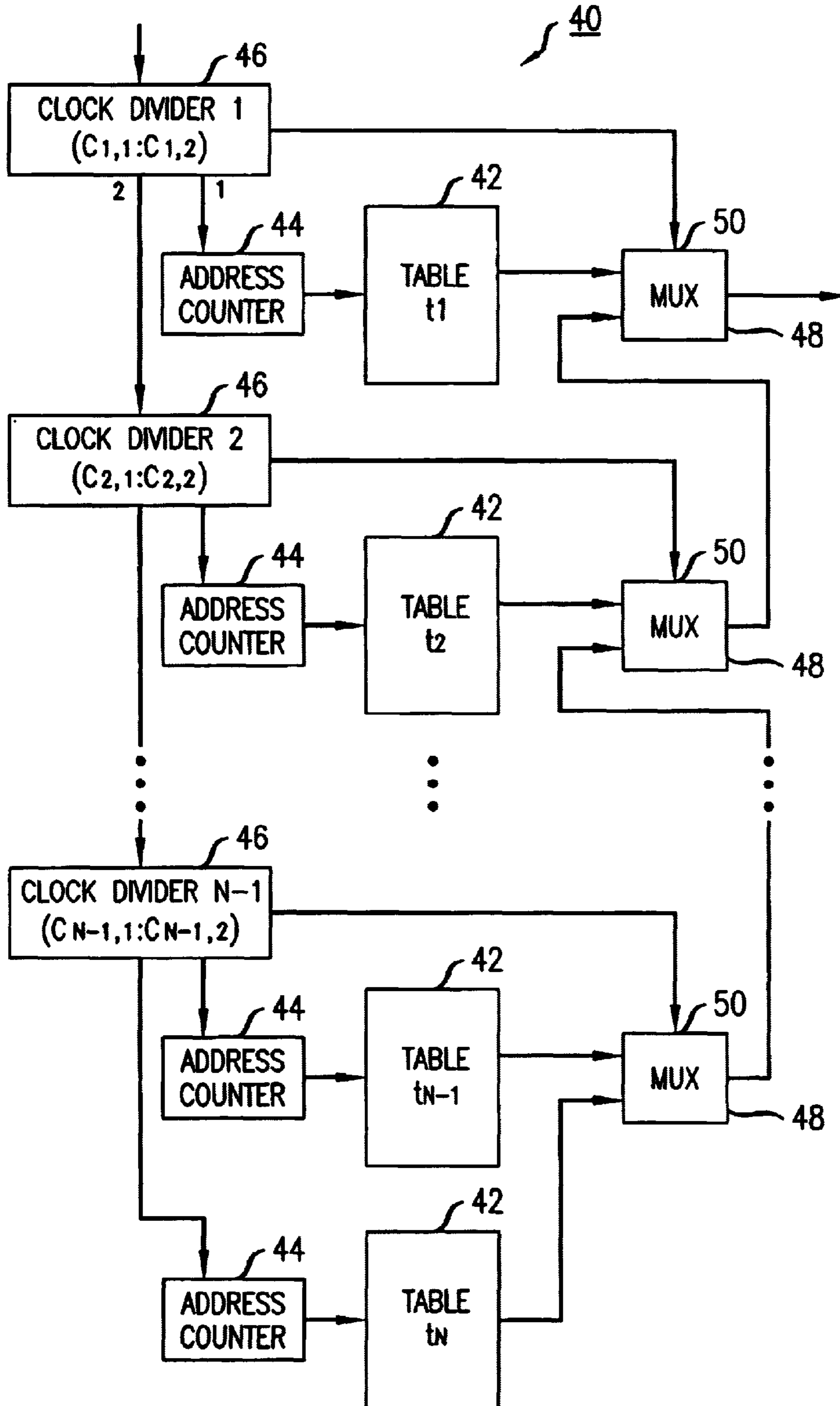
RECURSIVE IMPLEMENTATION OF GRANT GENERATOR USING MULTI-TABLES
