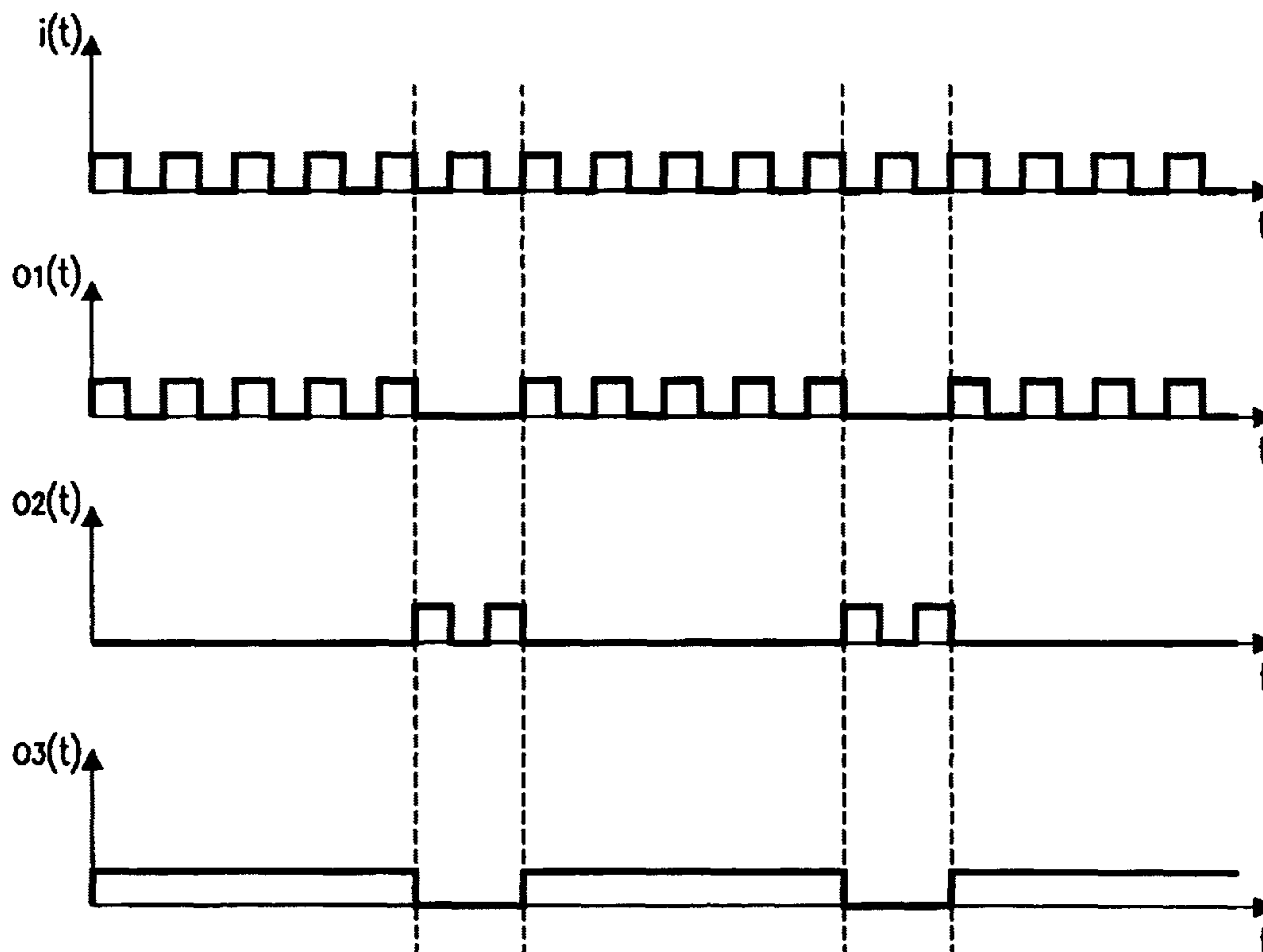
EXAMPLE TIMING DIAGRAM FOR INPUT AND OUTPUT SIGNALS OF CLOCK DIVIDER WITH DIVISION RATIO 5:2
