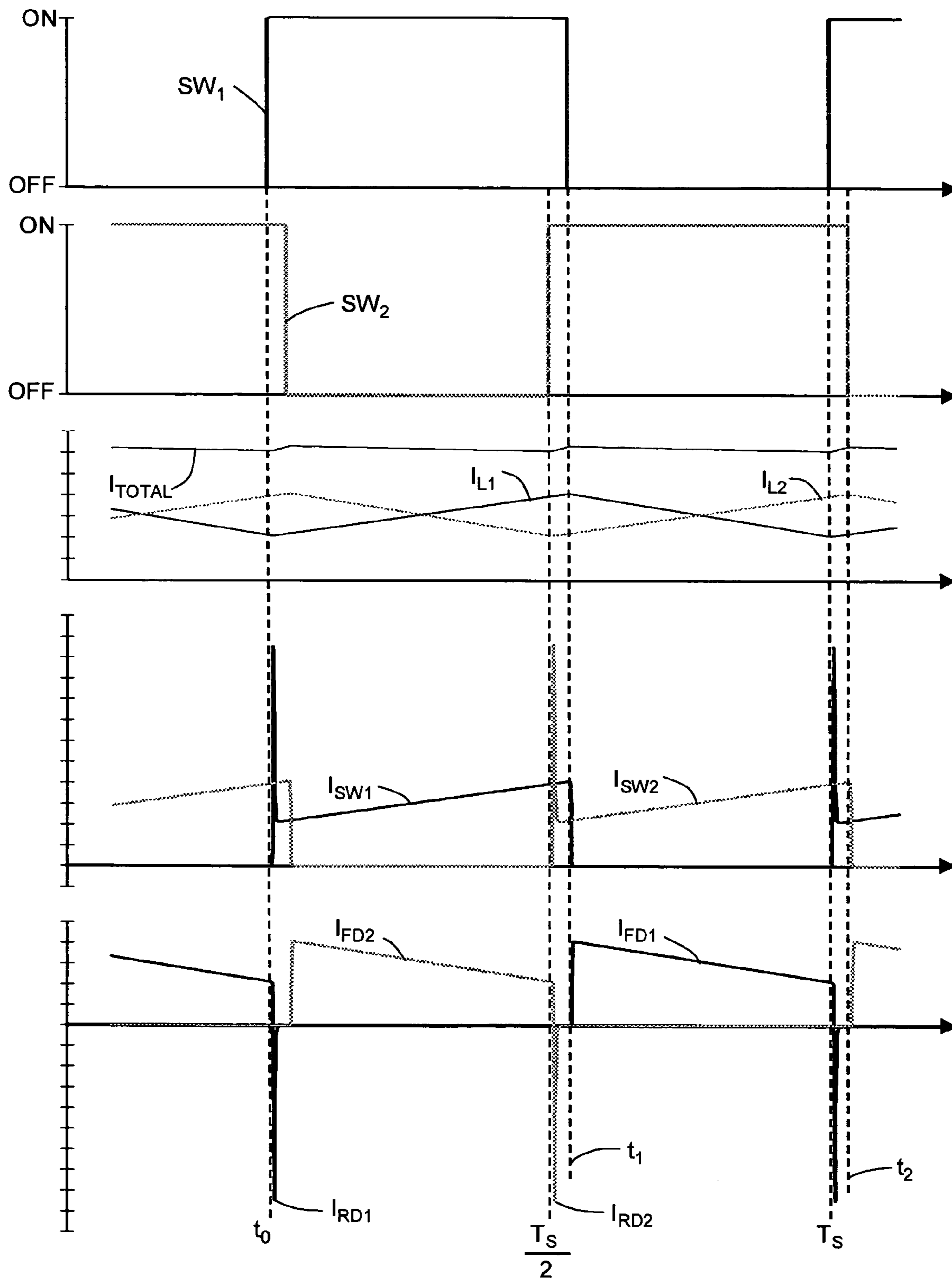
FIGURE 8 (PRIOR ART)
