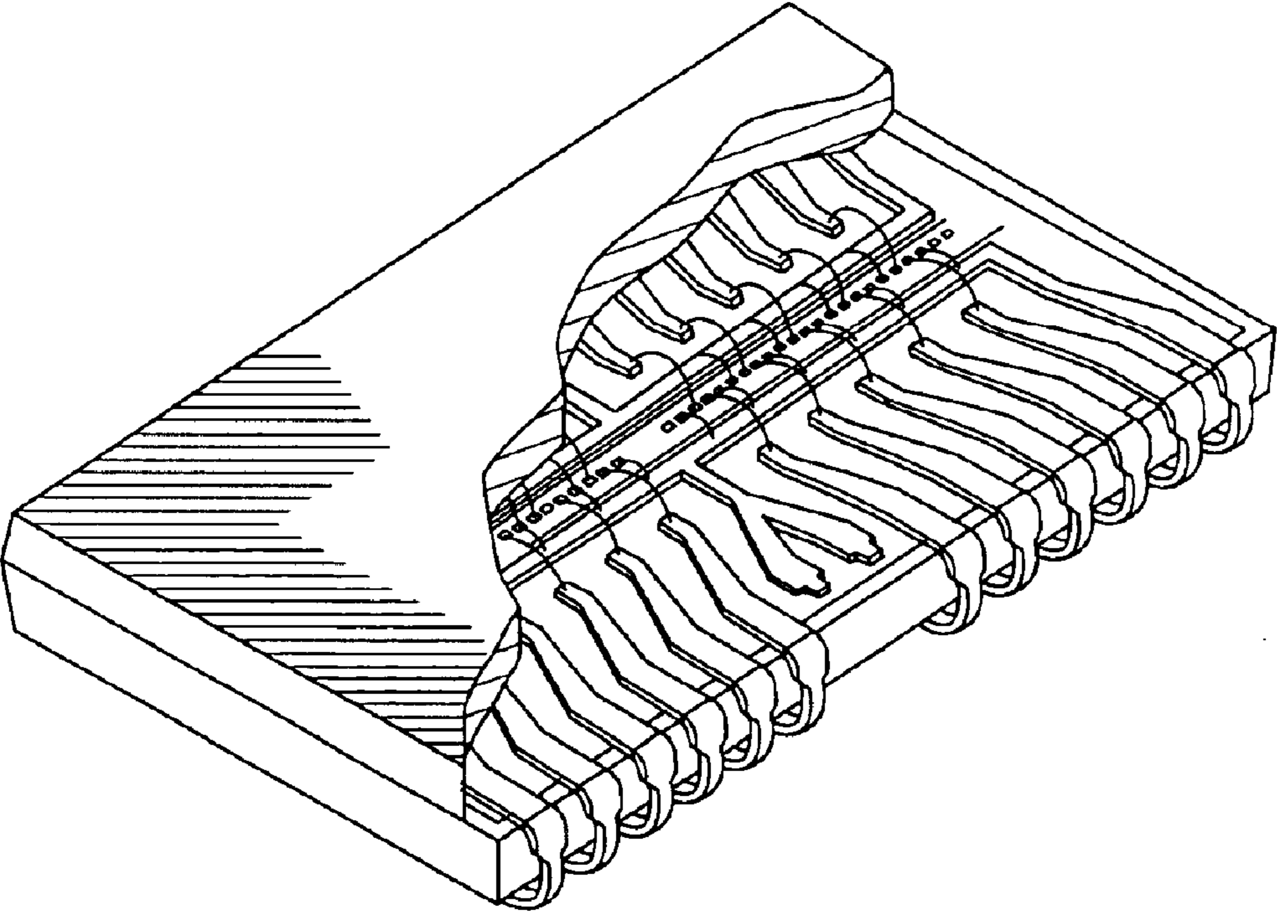
Fig. 5 (PRIOR ART)
