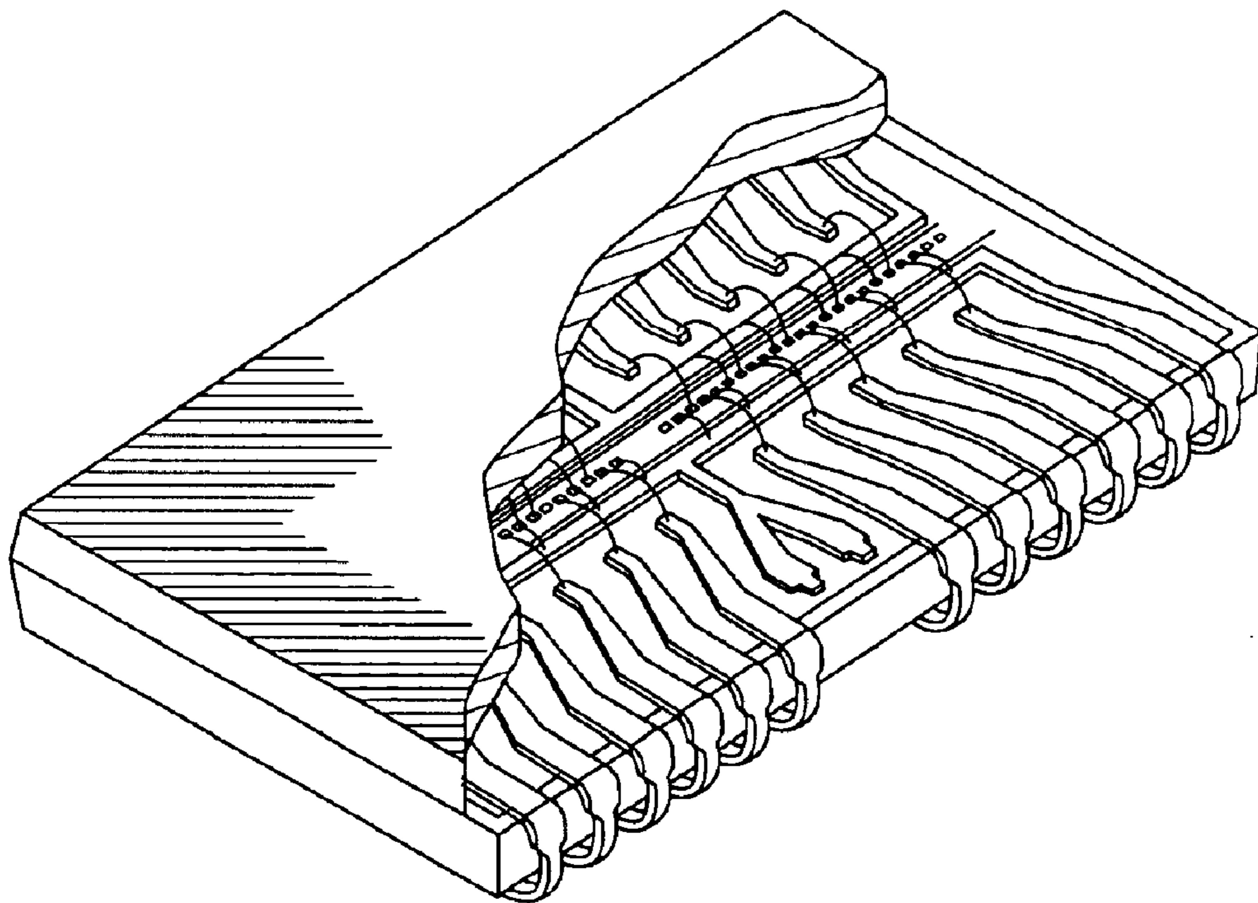
Fig. 5 (PRIOR ART)
