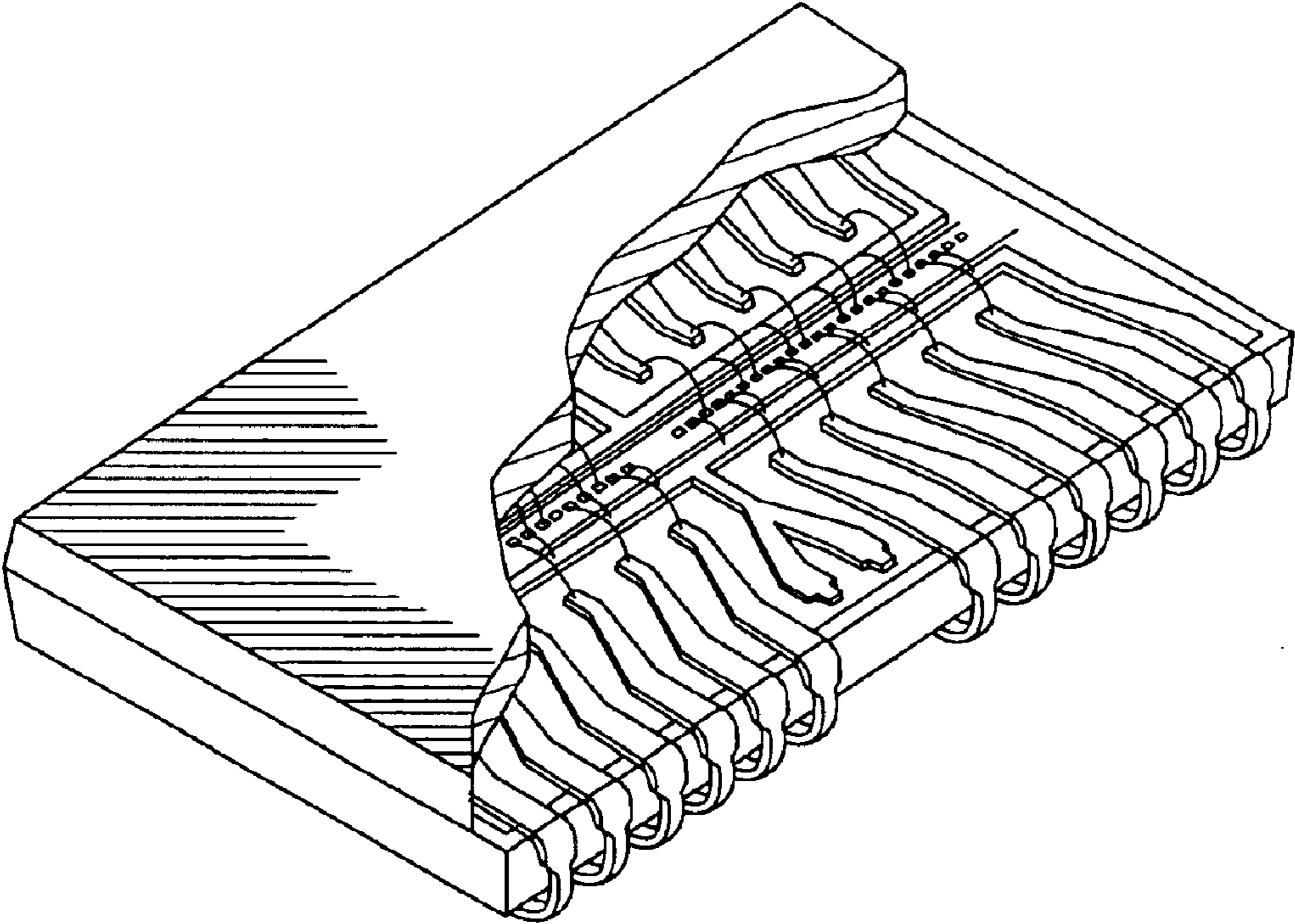
Fig. 5 (PRIOR ART)
