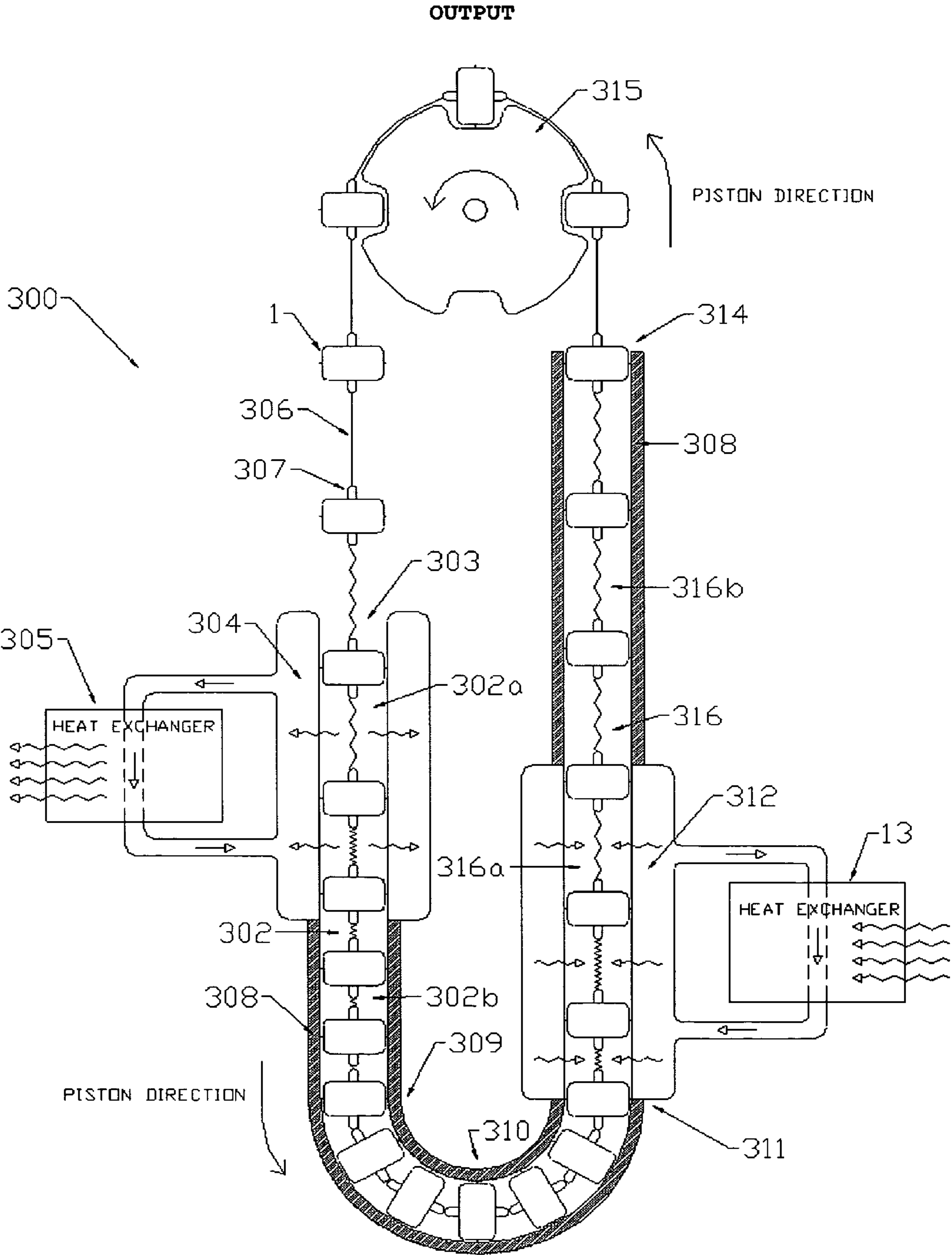
FIGURE 3 CARNOT CYCLE ENGINE WITH MECHANICAL WORK
