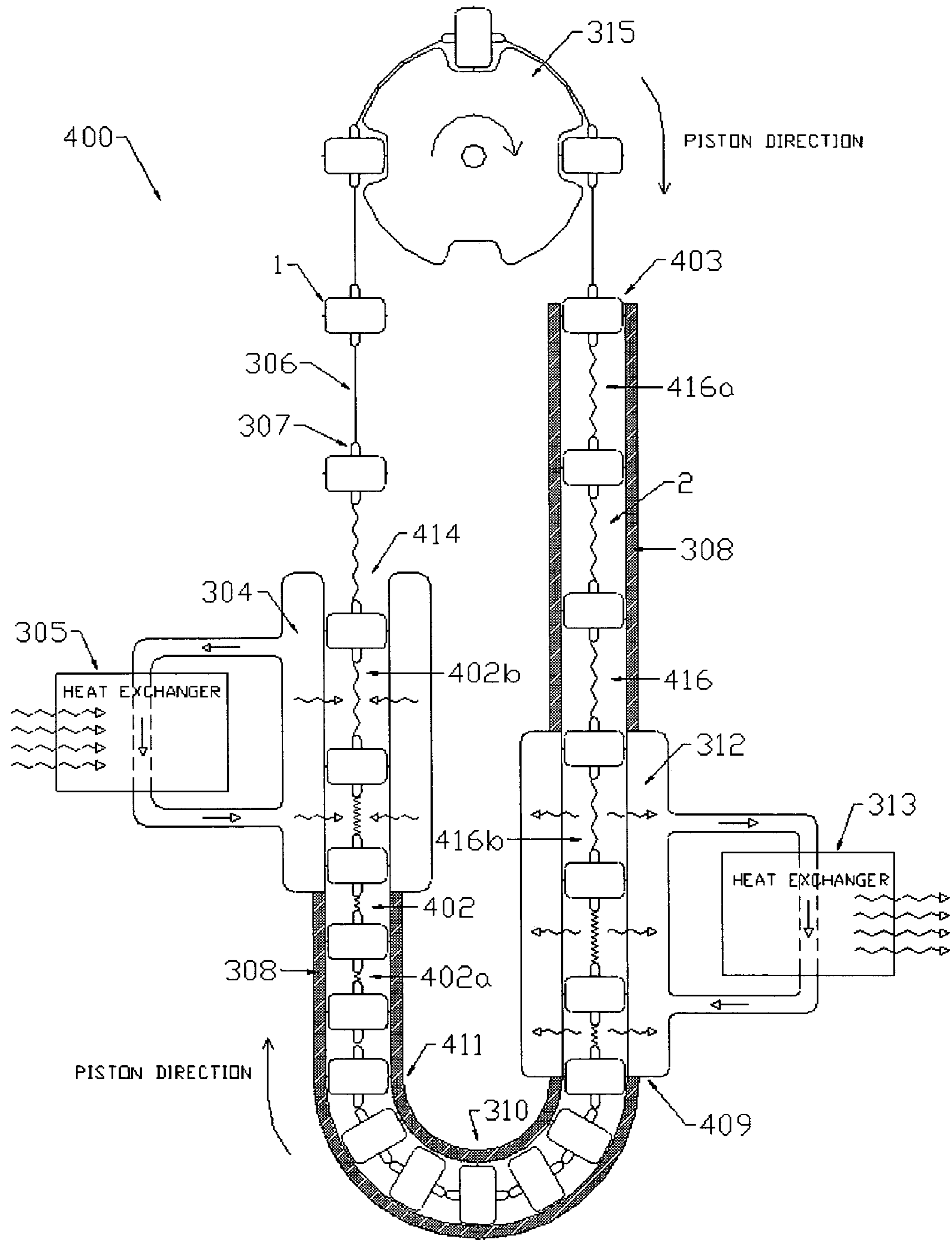
FIGURE 4 CARNOT CYCLE REFRIGERATOR WITH MECHANICAL WORK INPUT
