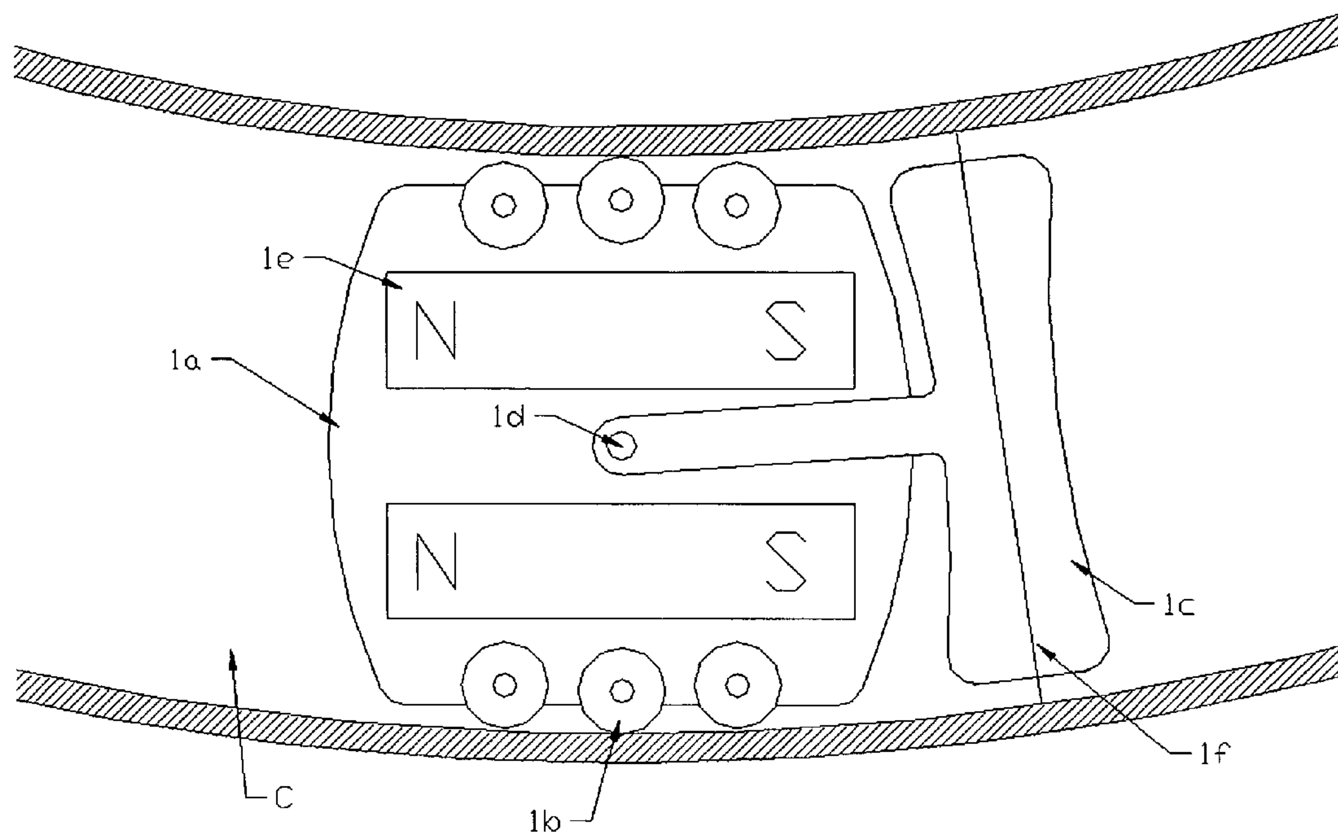
FIGURE 5 HINGED PISTON
