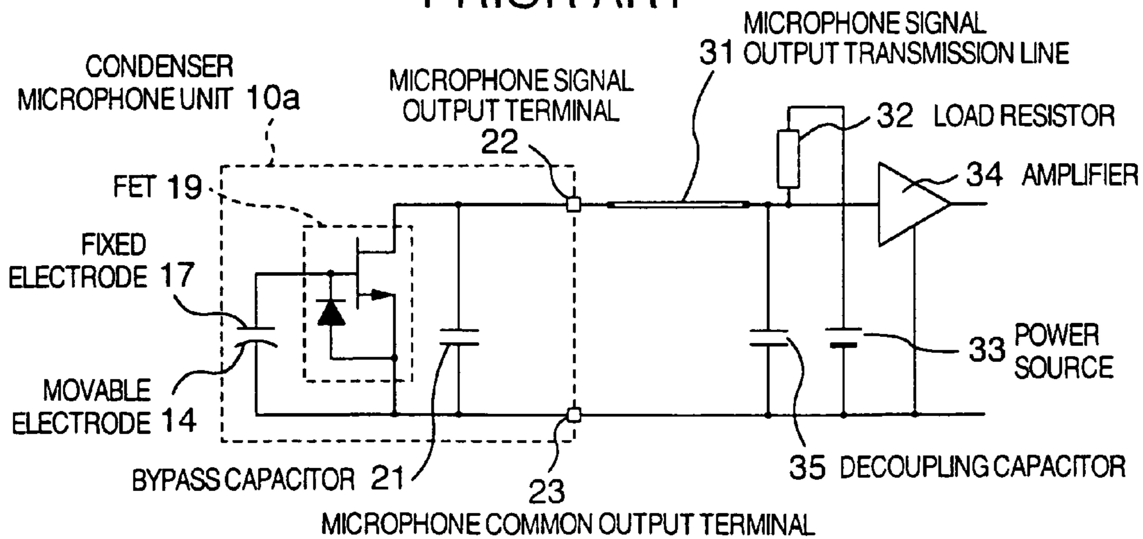
FIG.2 PRIOR ART
