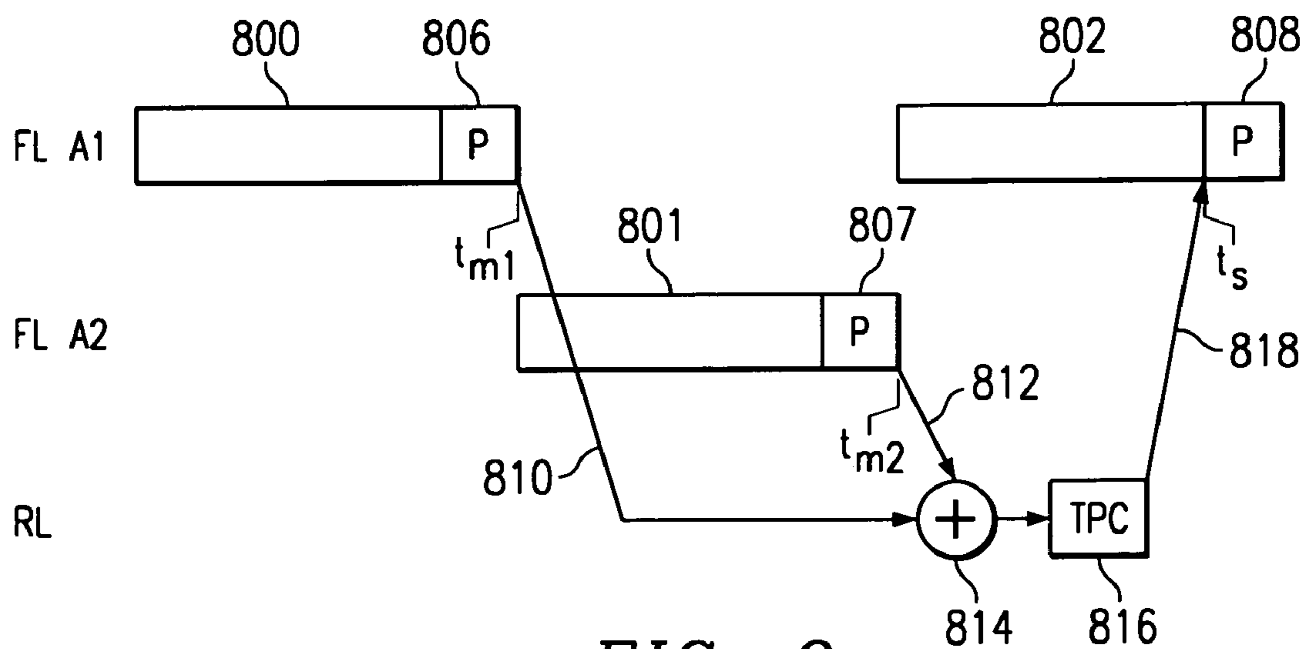
FIG. 8 (PRIOR ART)
