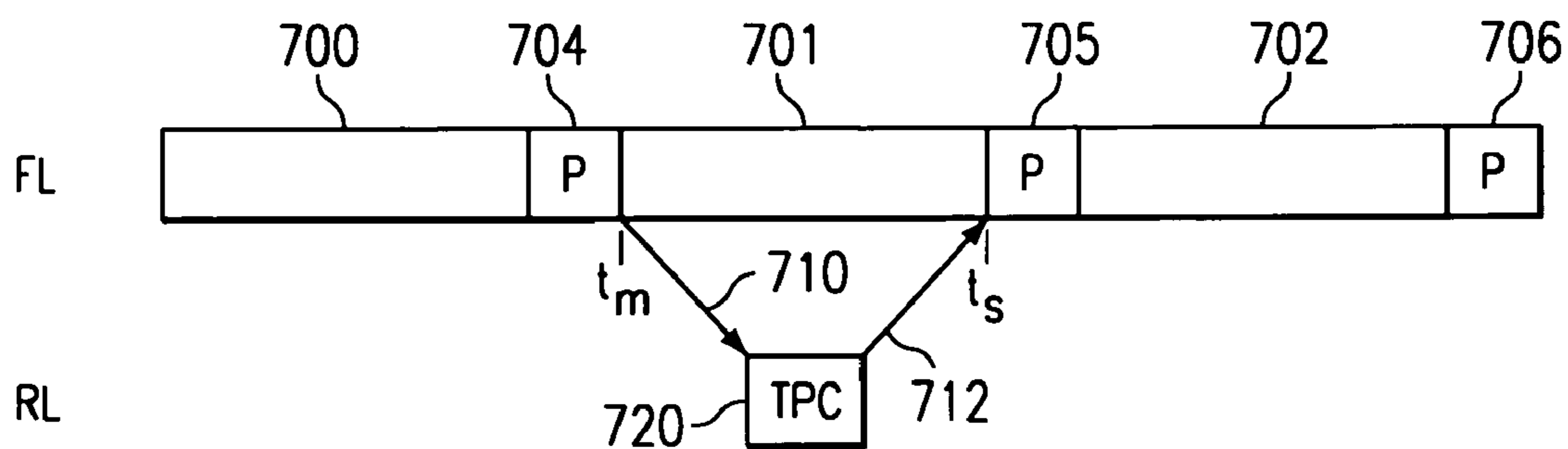
FIG. 7 (PRIOR ART)
