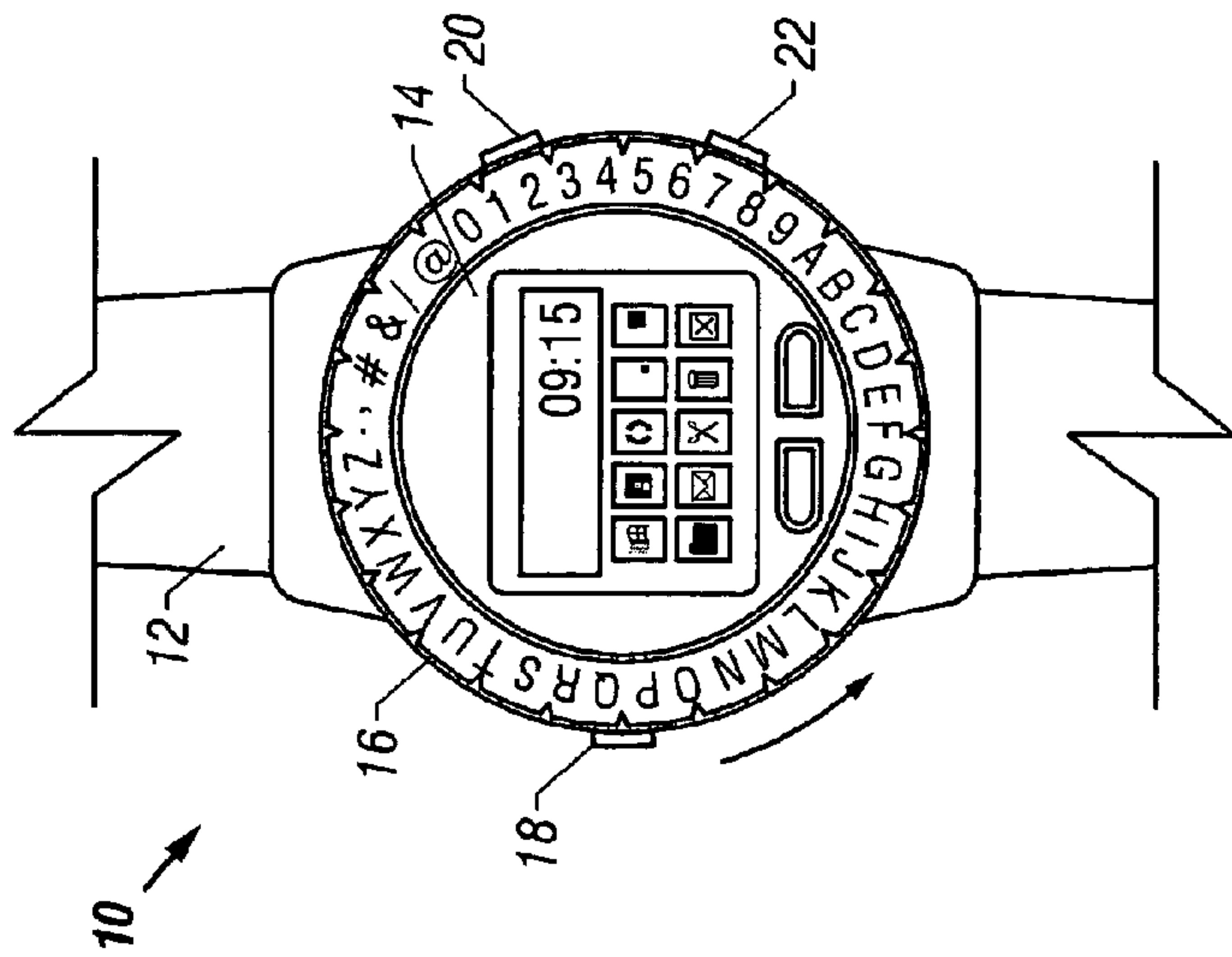
FIG. 1 (Prior Art)
