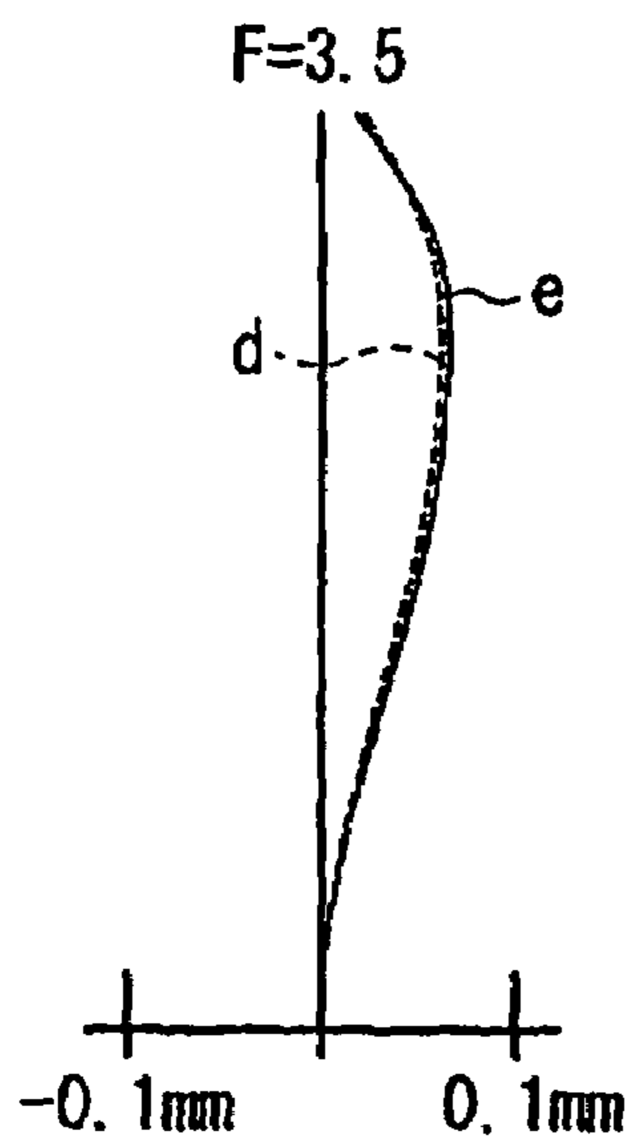
Spherical Aberration Fig. 3A
