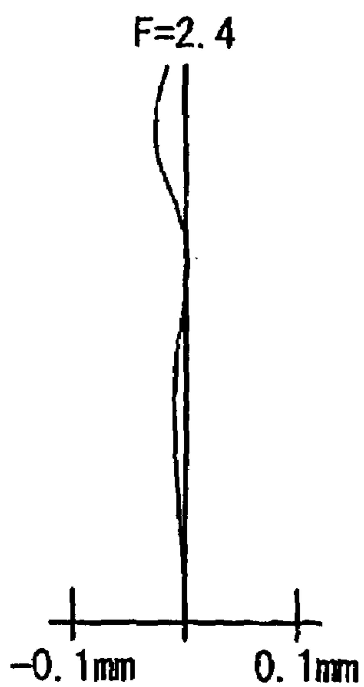
Spherical Aberration Fig. 4A
