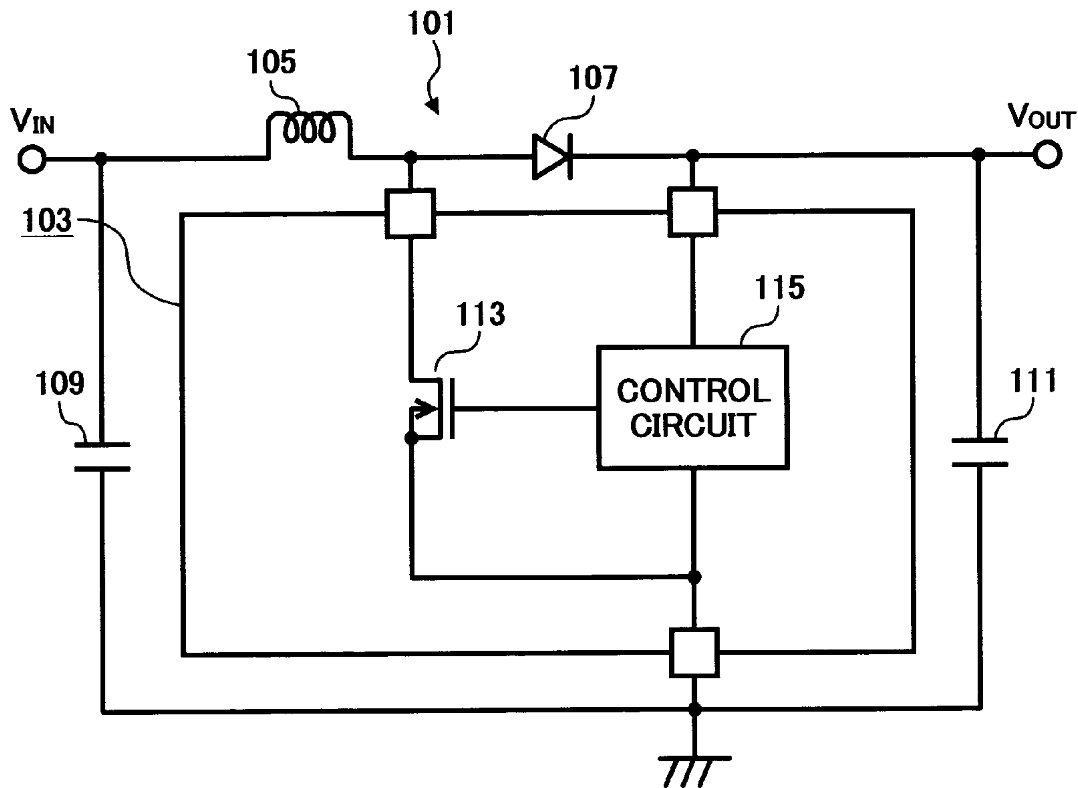
FIG. 1 PRIOR ART
