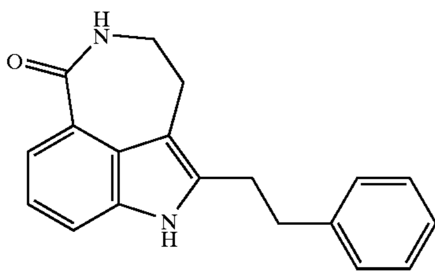
2-Phenethyl-1,3,4,5-tetrahydro-azepino[5,4,3-cd] indol-6-one (37)
