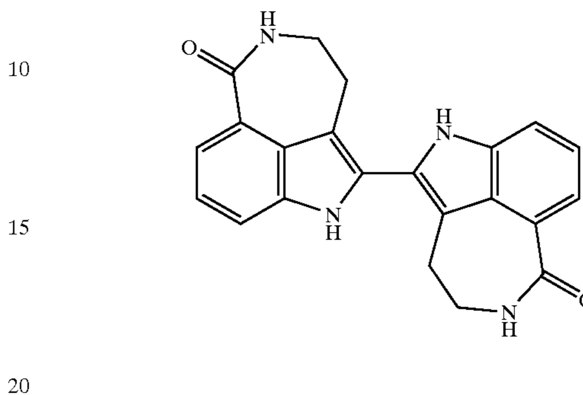
1,3,4,5,1',3',4',5'-Octahydro-[2,2']bi[azepino[5,4,3-cd]indolyl]-6,6'-dione
