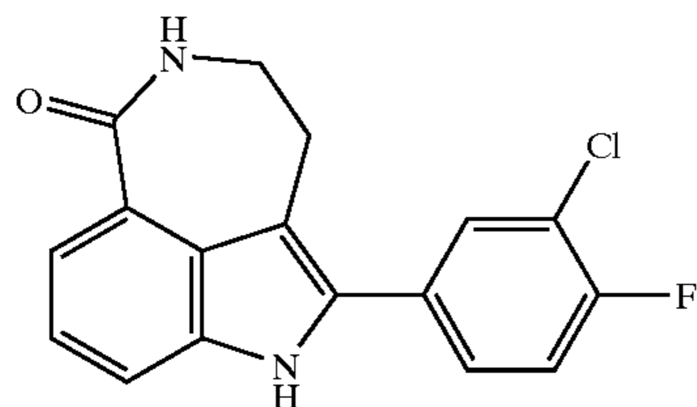
2-(3-Chloro-4-fluoro-phenyl)-1,3,4,5-tetrahydro-azepino[5,4,3-cd]indol-6-one (35)
