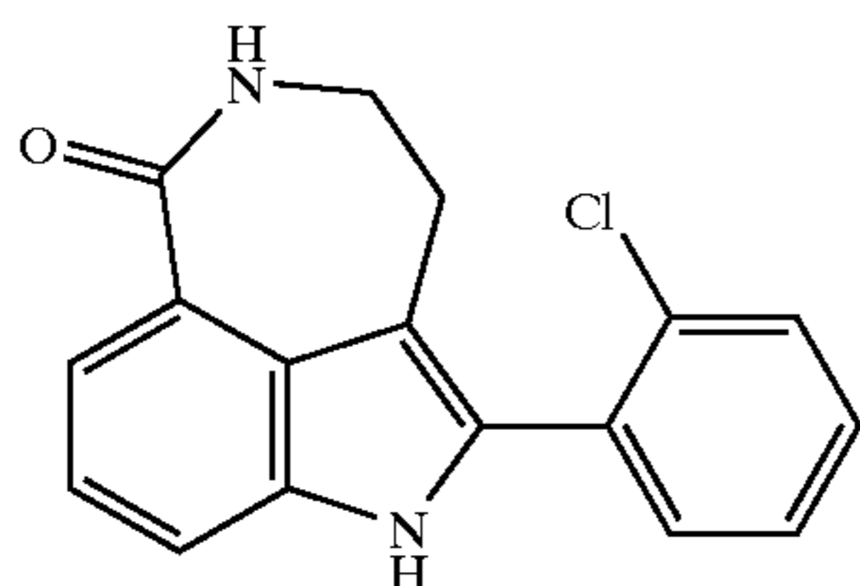
2-(2-Chlorophenyl)-1,3,4,5-tetrahydro-azepino[5,4,3-cd]indol-6-one (38)
