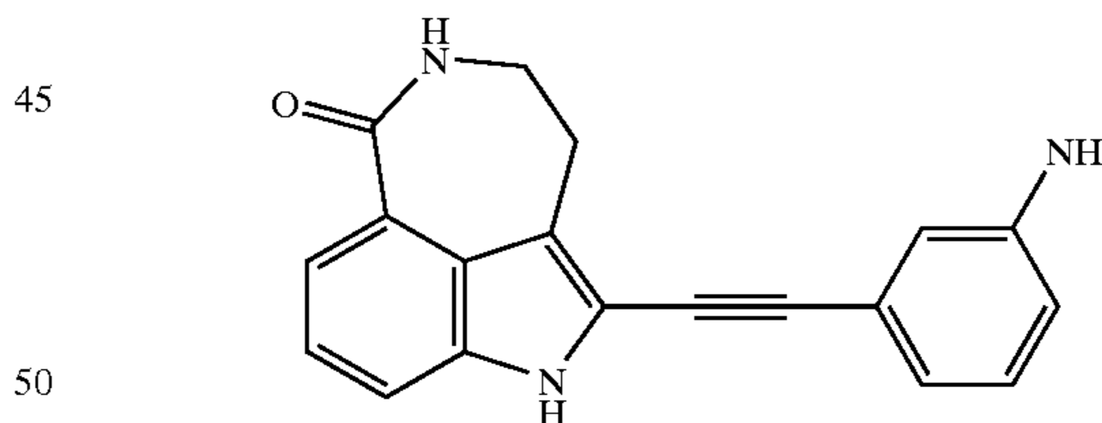
2-(3-Amino-phenylethynyl)-1,3,4,5-tetrahydro-azepino[5,4,3-cd]indol-6-one
