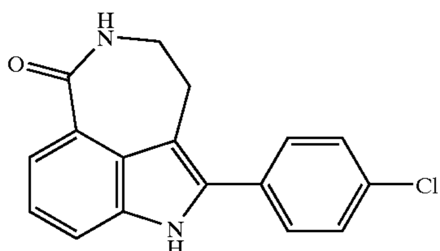
2-(4-Chloro-phenyl)-1,3,4,5-tetrahydro-azepino[5,4,3-cd]indol-6-one
