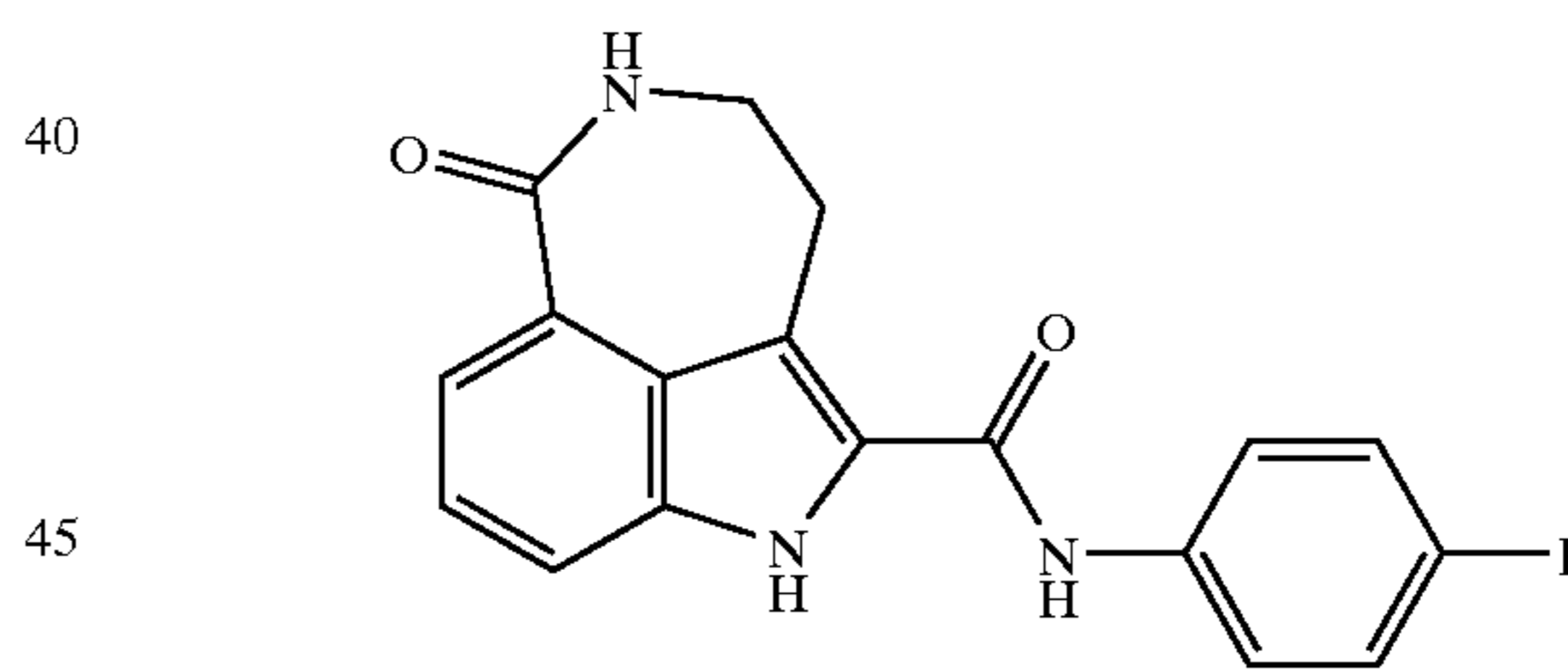
6-Oxo-3,4,5,6-tetrahydro-1H-azepino[5,4,3-cd]indole-2-carboxylic acid (4-fluoro-phenyl)-amide
