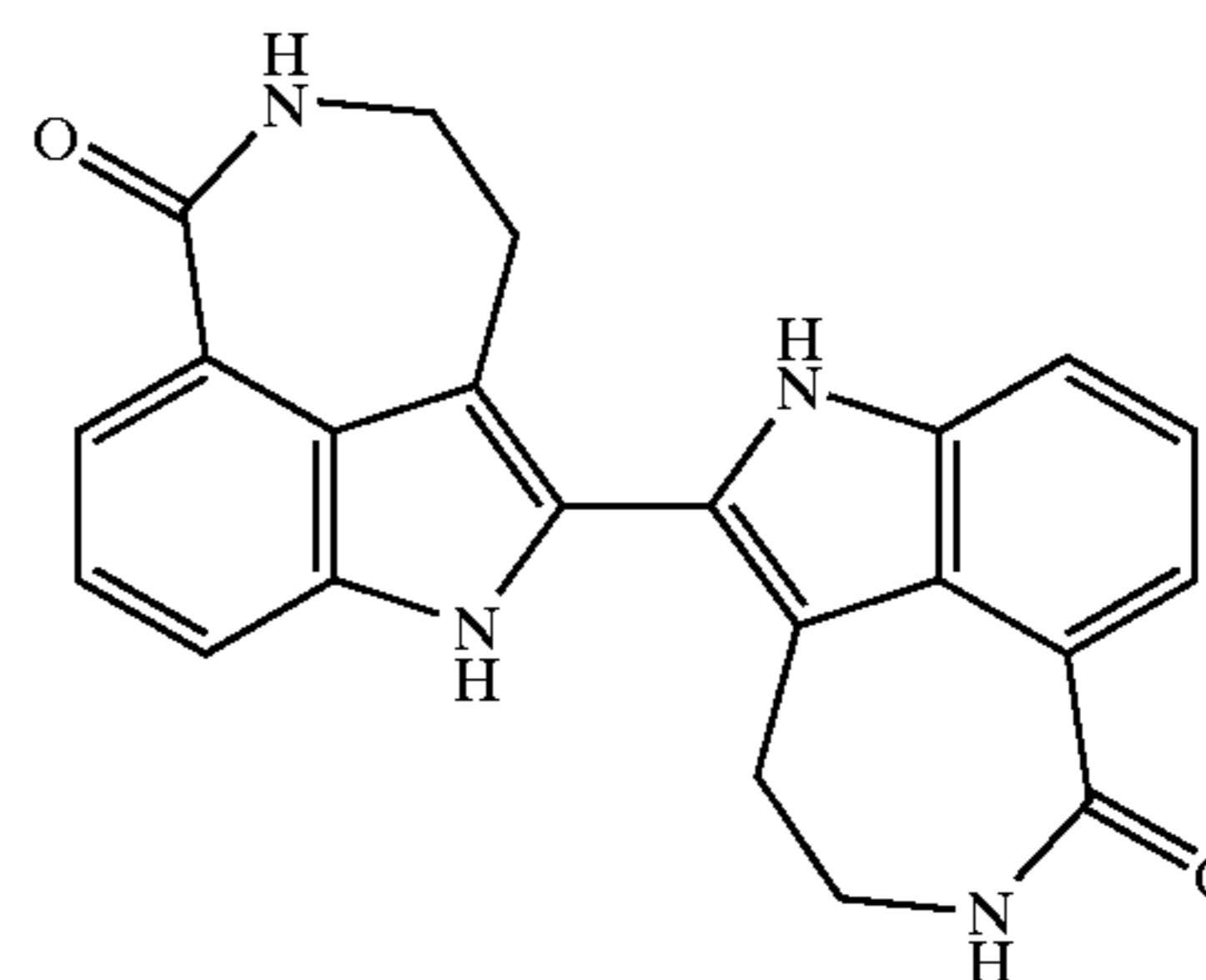
1,3,4,5,1',3',4',5'-Octahydro-[2,2']bi[azepino[5,4,3-cd]indolyl]-6,6'-dione
