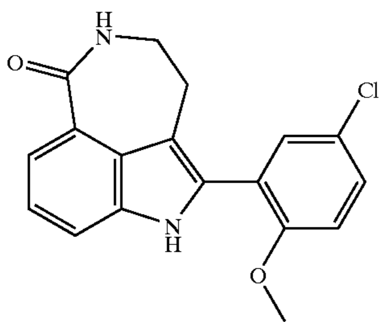
2-(5-Chloro-2-methoxy-phenyl)-3,4,5,6-tetrahydro-azepino[5,4,3-cd]indol-6-one
