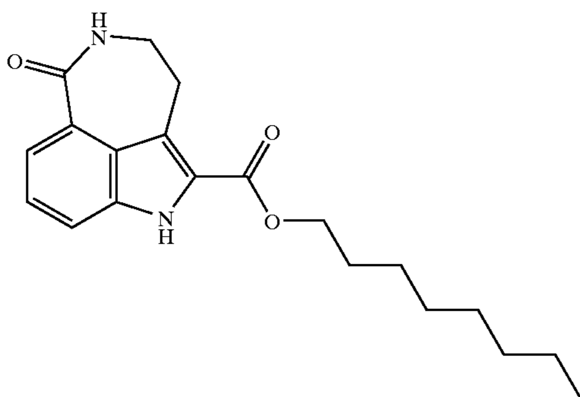
6-Oxo-3,4,5,6-tetrahydro-1H-azepino[5,4,3-cd]indole-2-carboxylic acid octyl ester
