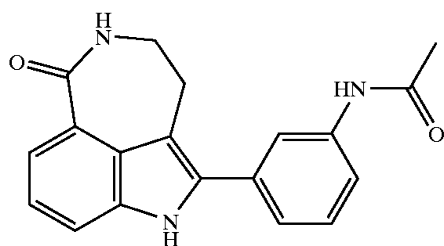
N-[3-(6-Oxo-3,4,5,6-tetrahydro-1H-azepino[5,4,3-cd]indol-2-yl)-phenyl]-acetamide
