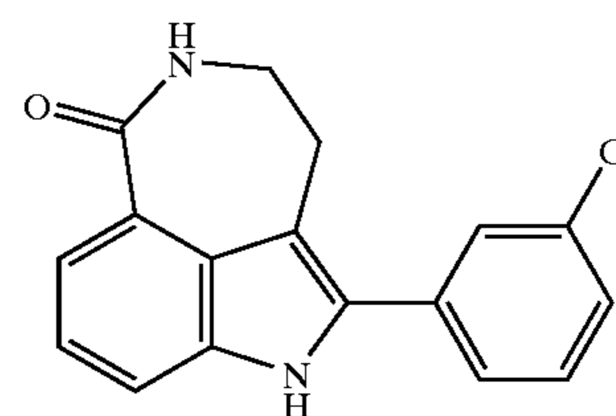
2-(3-Chlorophenyl)-1,3,4,5-tetrahydro-azepino [5,4,3-cd]indol-6-one (40)
