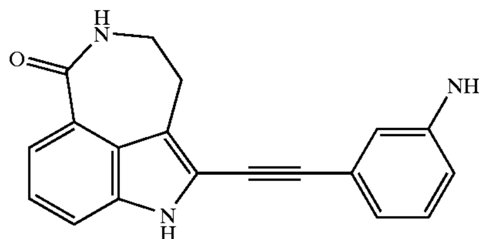
2-(3-Amino-phenylethynyl)-1,3,4,5-tetrahydro-azepino[5,4,3-cd]indol-6-one
