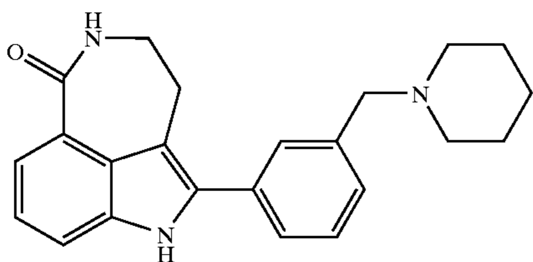
2-(3-(3-Piperidin-1-ylmethylphenyl)-3,4,5,6-tetrahydro-1H-azepino[5,4,3-cd]indol-6-one
