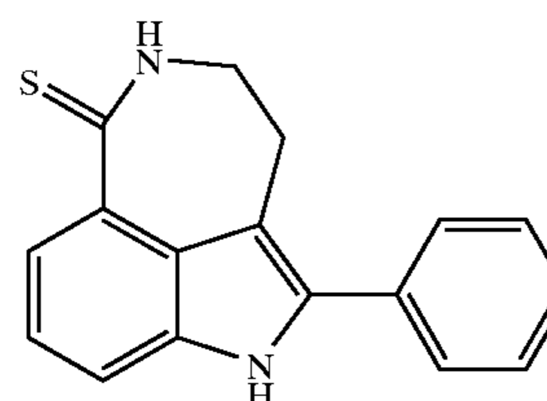
2-Phenyl-1,3,4,5-tetrahydro-azepino[5,4,3-cd]indole-6-thione (24)
