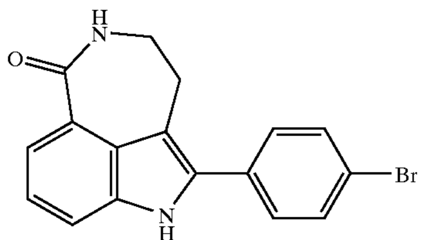
2-(4-Bromophenyl)-1,3,4,5-tetrahydro-azepino[5,4,3-cd]indol-6-one (34)
