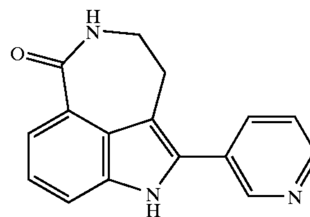
2-Pyridin-3-yl-1,3,4,5-tetrahydro-azepino[5,4,3-cd]indol-6-one
