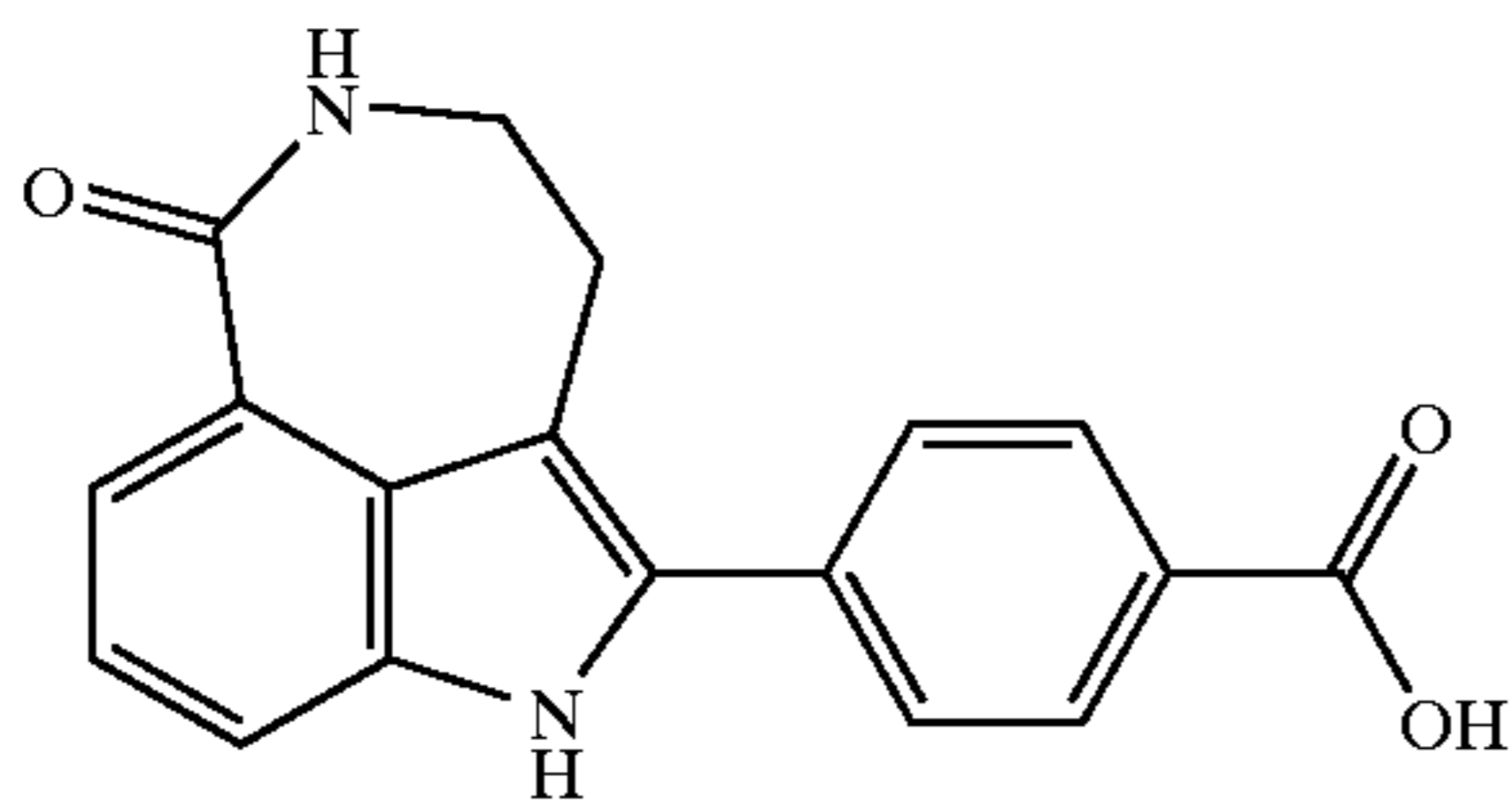
4-(6-Oxo-3,4,5,6-tetrahydro-1H-azepino[5,4,3-cd]indol-2-yl)-benzoic acid
