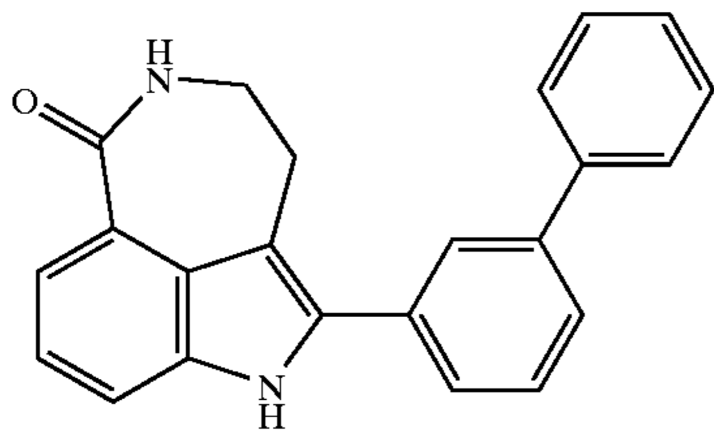
2-Biphenyl-3-yl-1,3,4,5-tetrahydro-azepino[5,4,3-cd]indol-6-one
