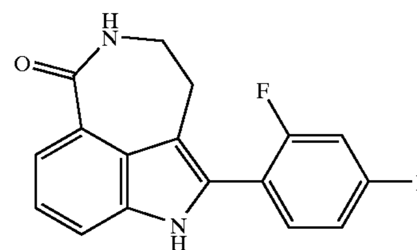
2-(2,4-Difluoro-phenyl)-1,3,4,5-tetrahydro-azepino [5,4,3-cd]indol-6-one (39)
