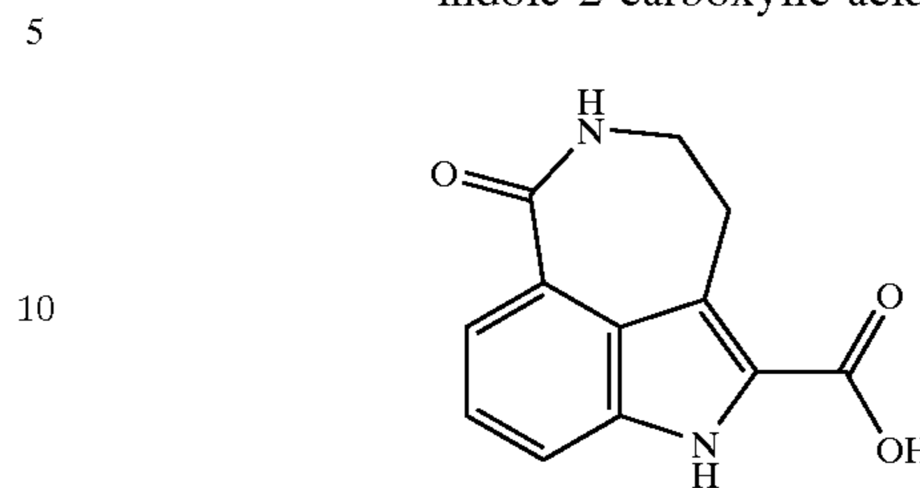
6-Oxo-3,4,5,6-tetrahydro-1H-azepino[5,4,3-cd]indole-2-carboxylic acid
