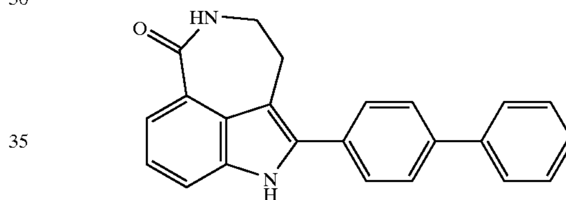
2-Biphenyl-4-yl-1,3,4,5-tetrahydro-azepino[5,4,3-cd]indol-6-one
