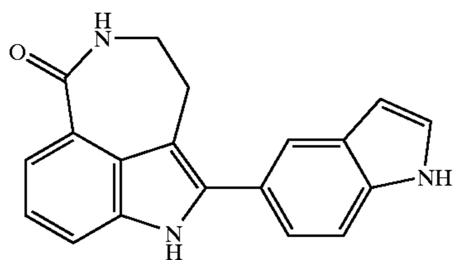
2-(1H-Indol-5-yl)-1,3,4,5-tetrahydro-azepino[5,4,3-cd]indol-6-one
