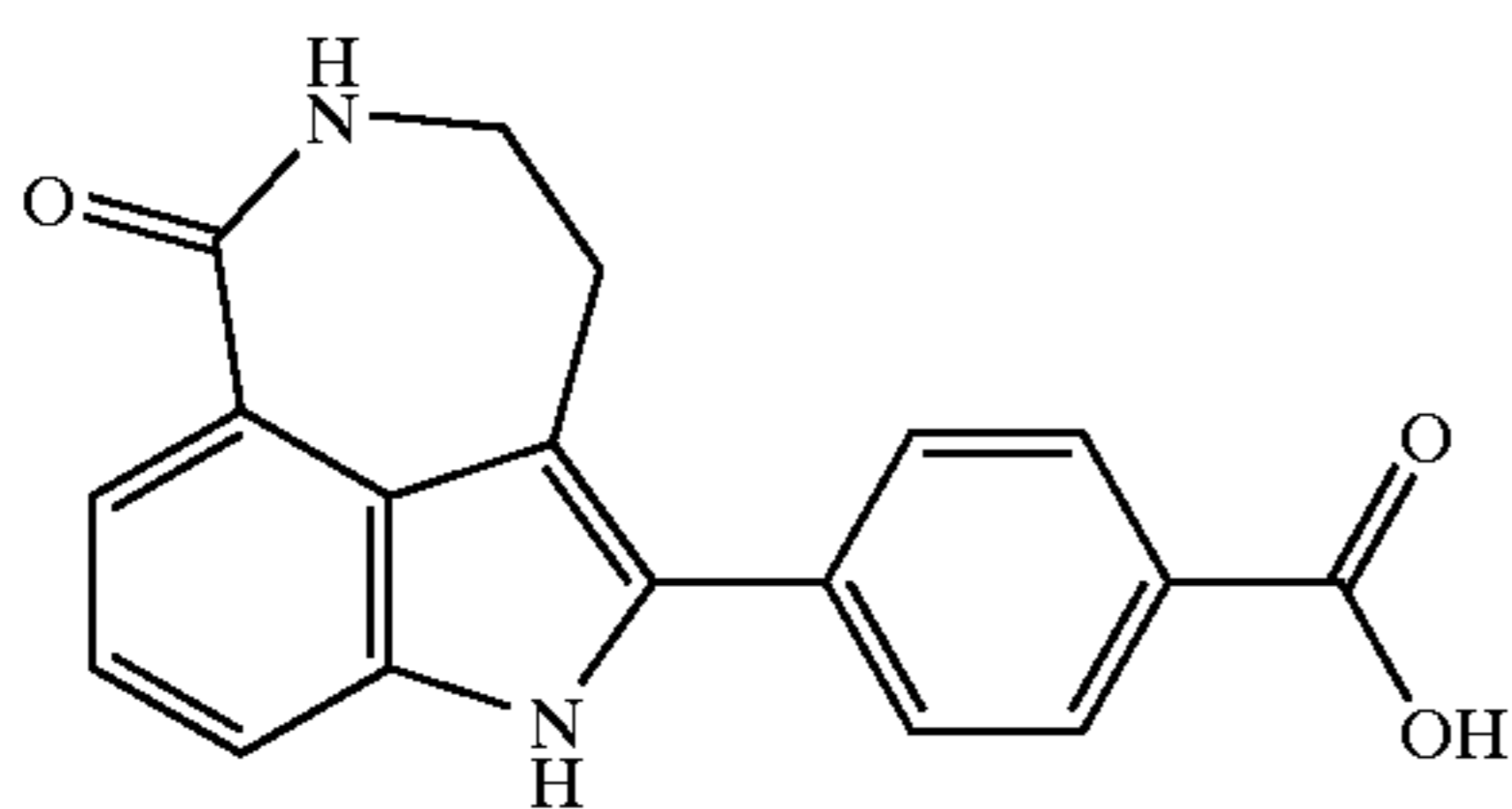
4-(6-Oxo-3,4,5,6-tetrahydro-1H-azepino[5,4,3-cd]indol-2-yl)-benzoic acid
