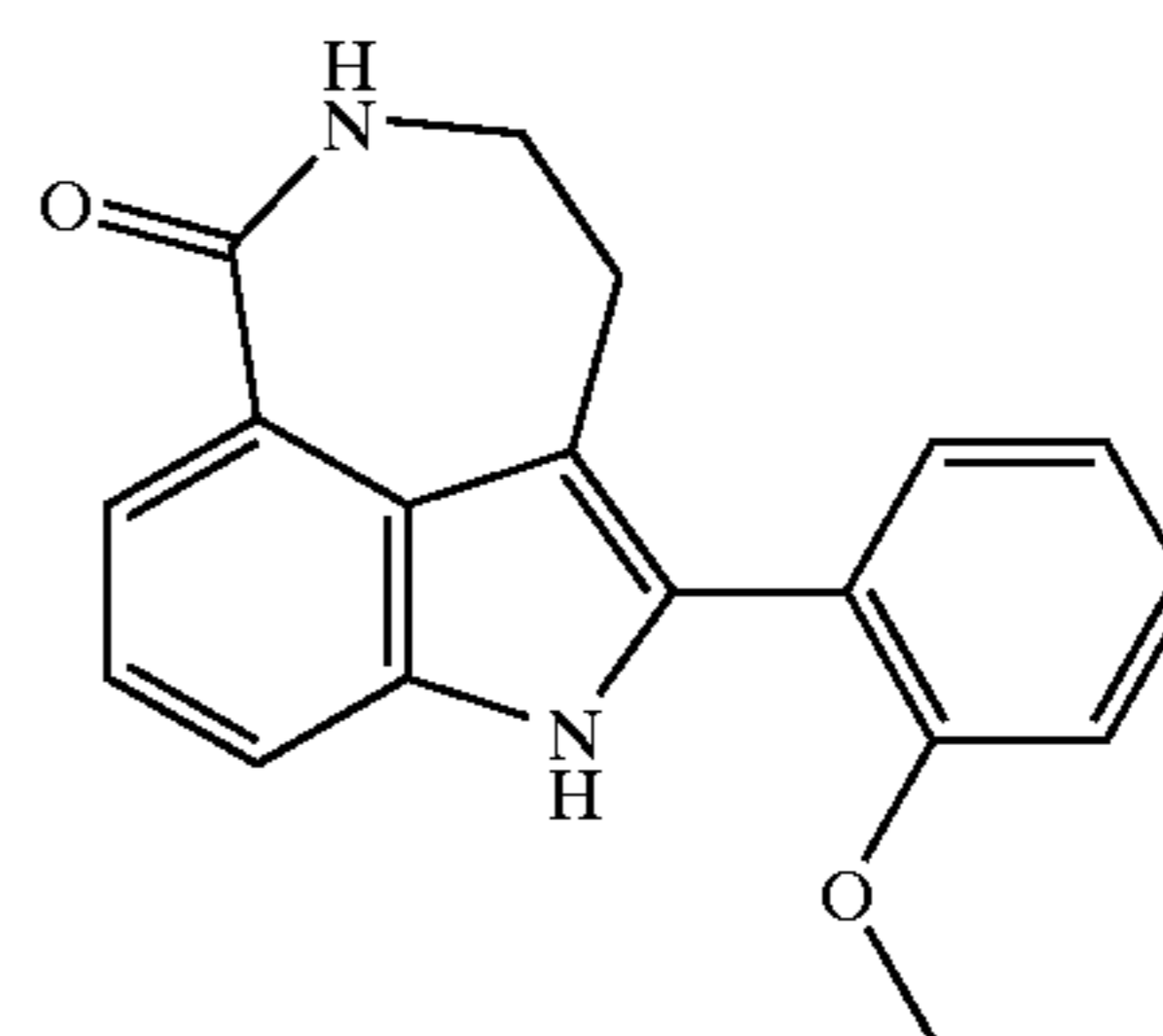
2-(2-Methoxy-phenyl)-1,3,4,5-tetrahydro-azepino[5,4,3-cd]indol-6-one
