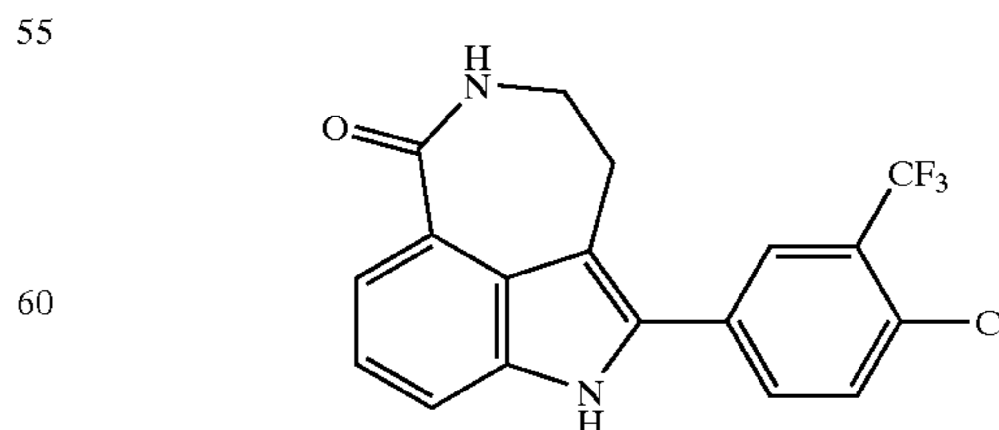
2-(4-Chloro-3-trifluoromethyl-phenyl)-1,3,4,5-tetrahydro-azepino[5,4,3-cd]indol-6-one
