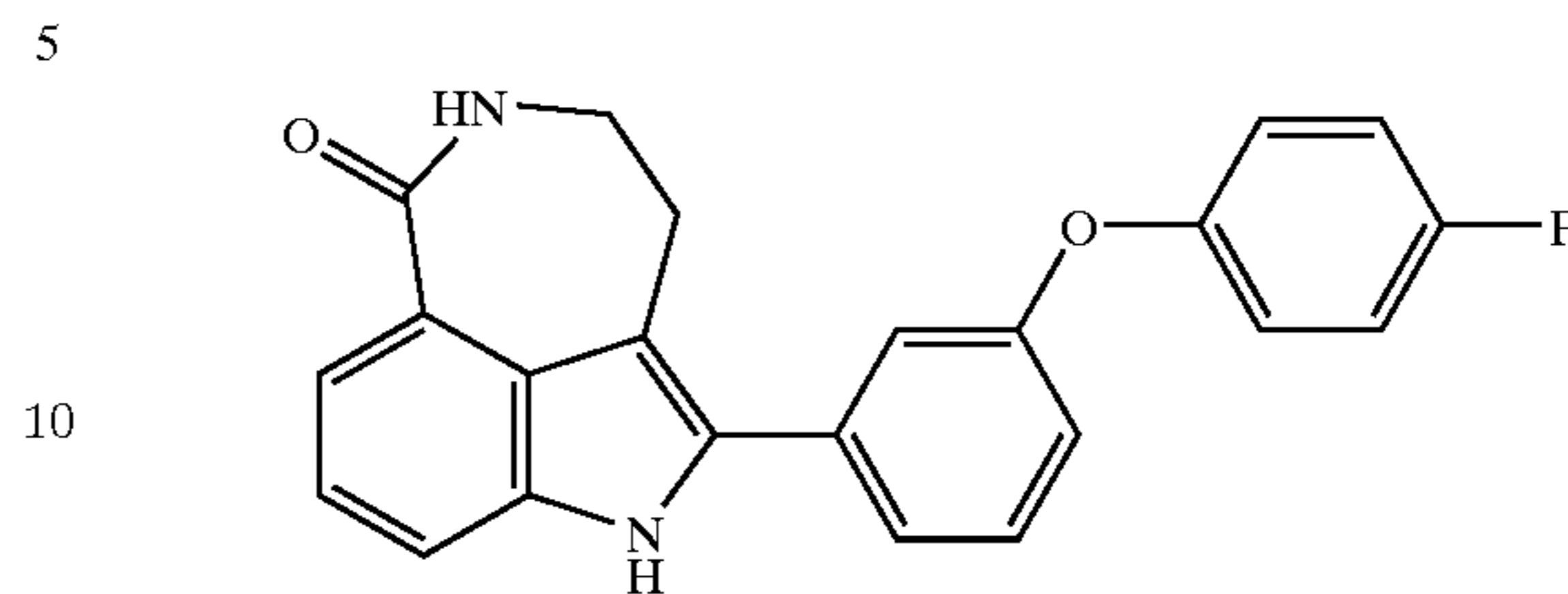
2-[3-(4-Fluoro-phenoxy)-phenyl]-1,3,4,5-tetrahydro-azepino[5,4,3-cd]indol-6-one
