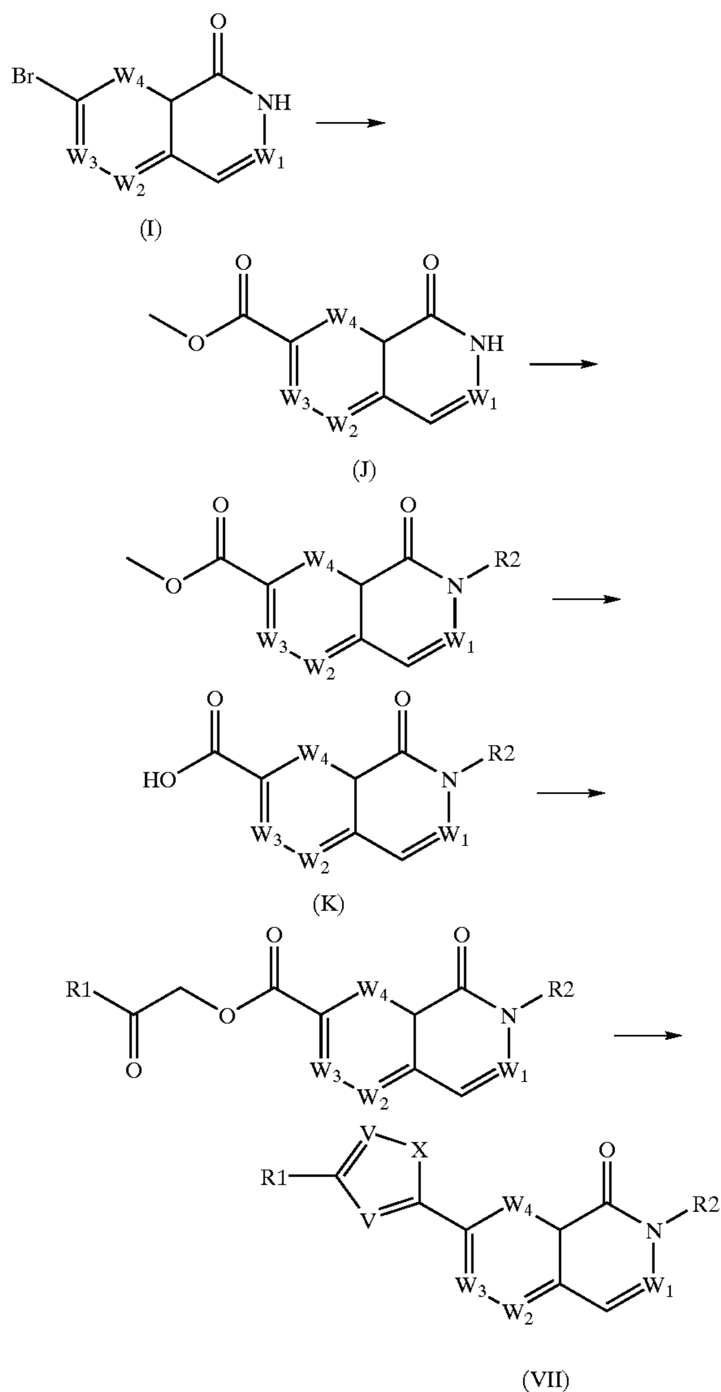
Scheme 2b.
