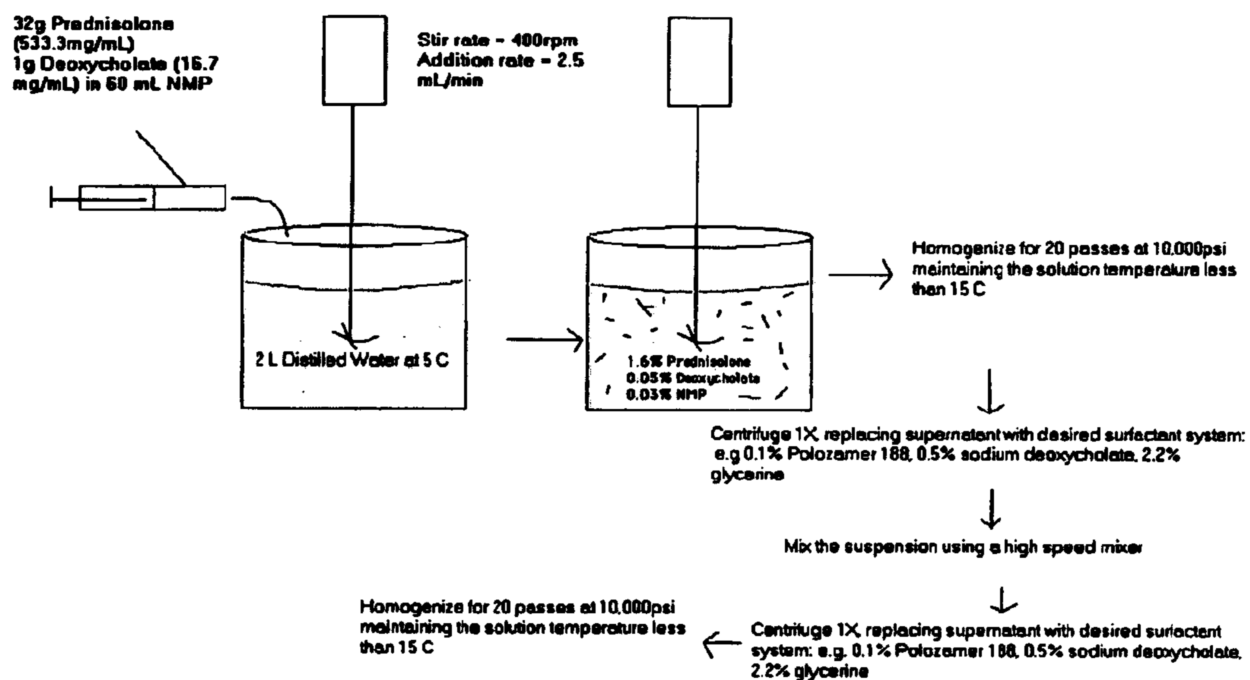
Figure 8: Diagram of Microprecipitation Process for Prednisolone (Examples 9-12)
