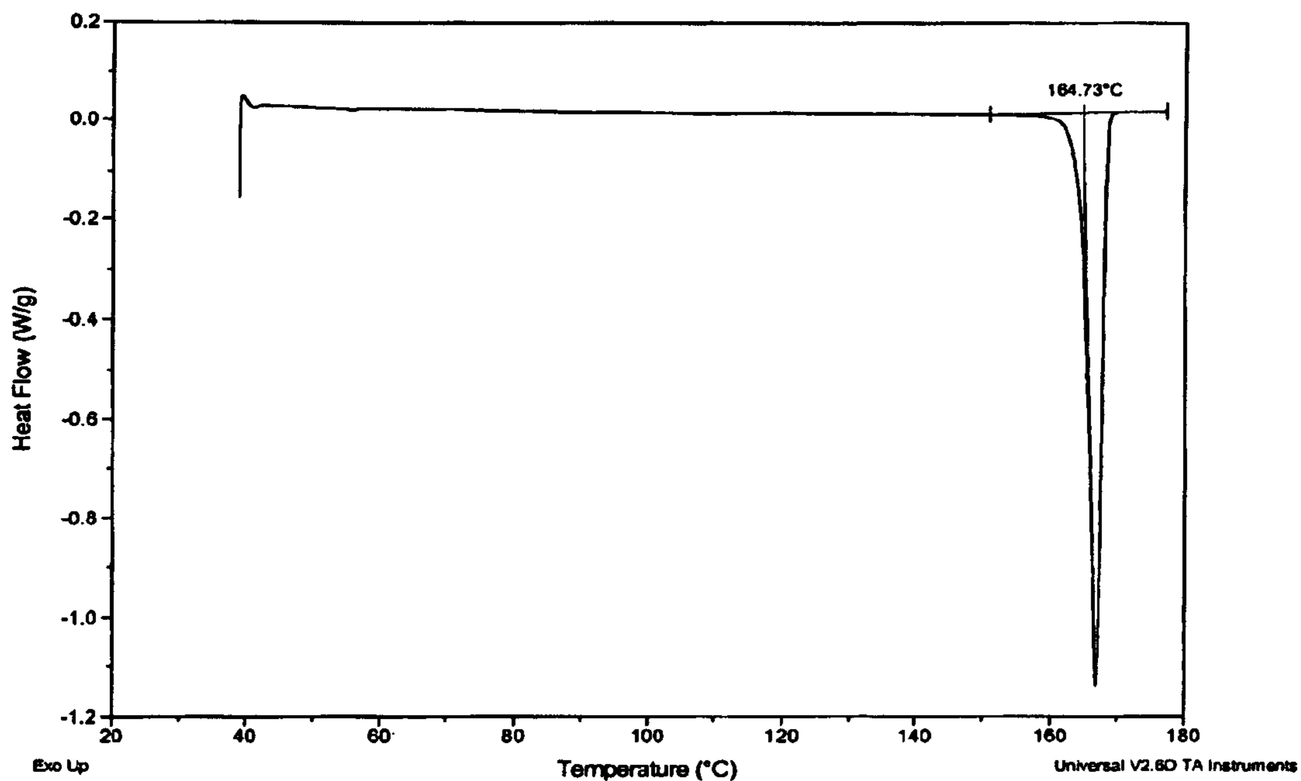
Figure 13a: DSC trace for raw material itraconazole (Example 16)
