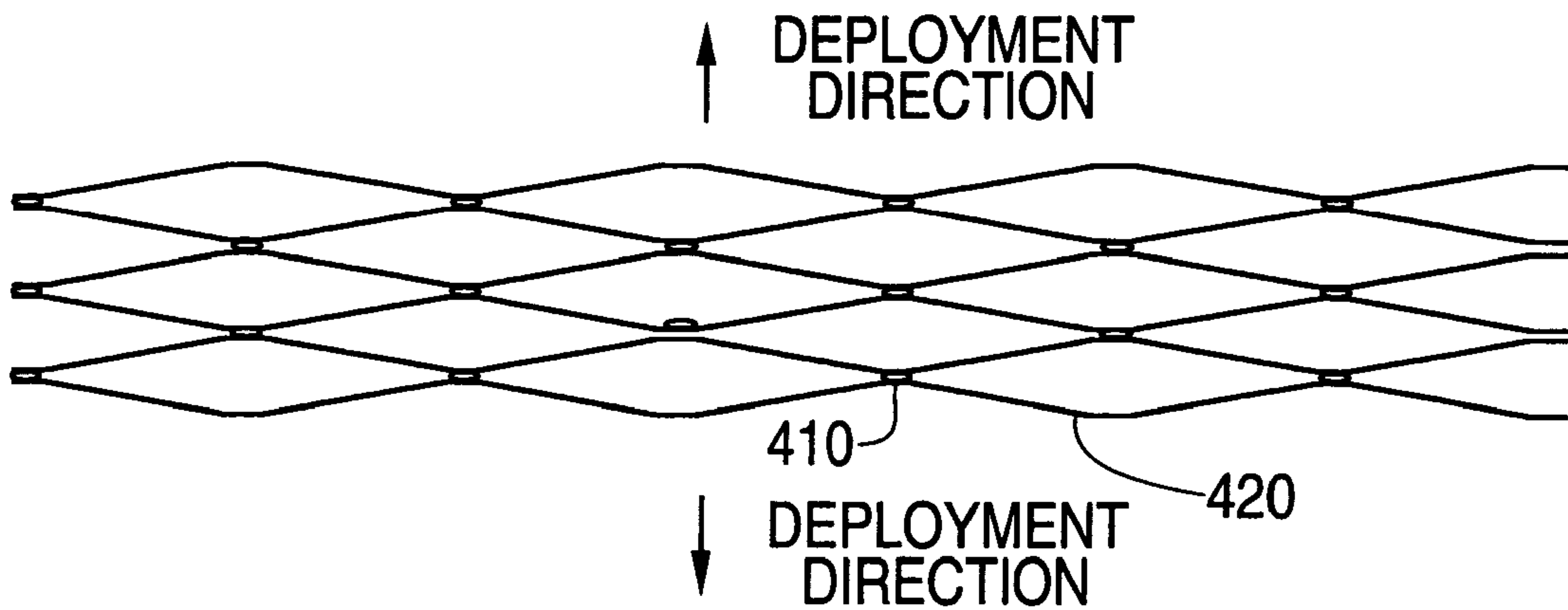
FIG. 4 (PRIOR ART)
