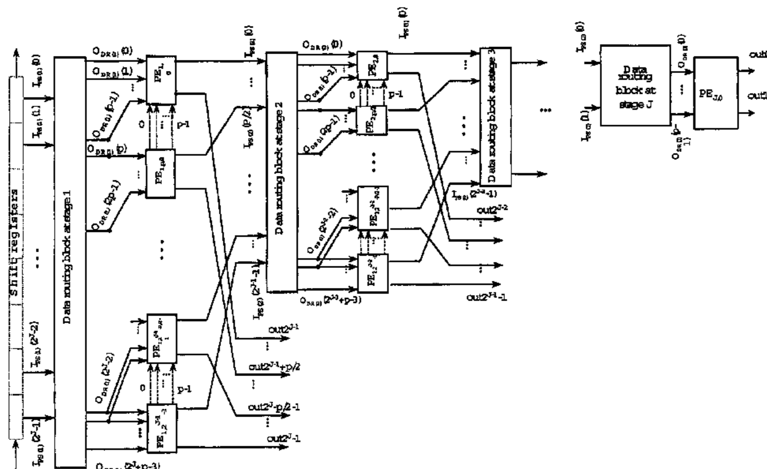
The general structure of Type 1 and Type 2 core DW T architectures
