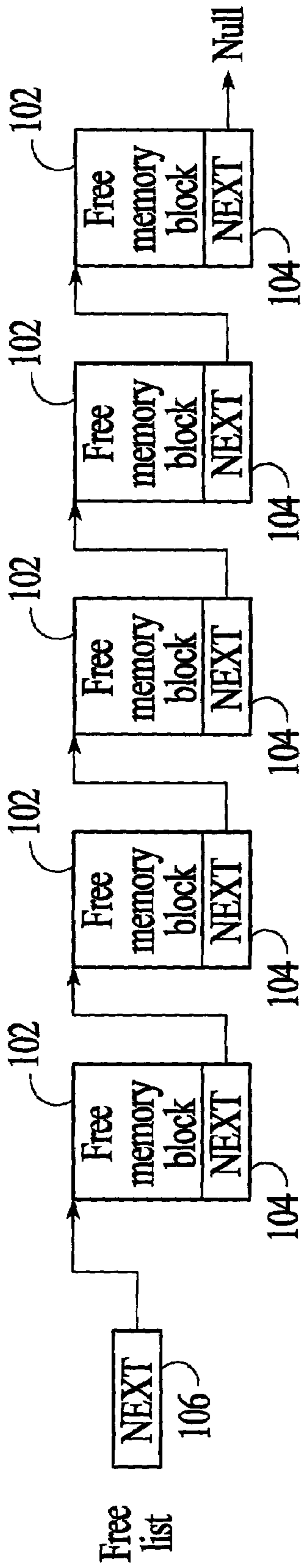
FIG. 1 (PRIOR ART)
