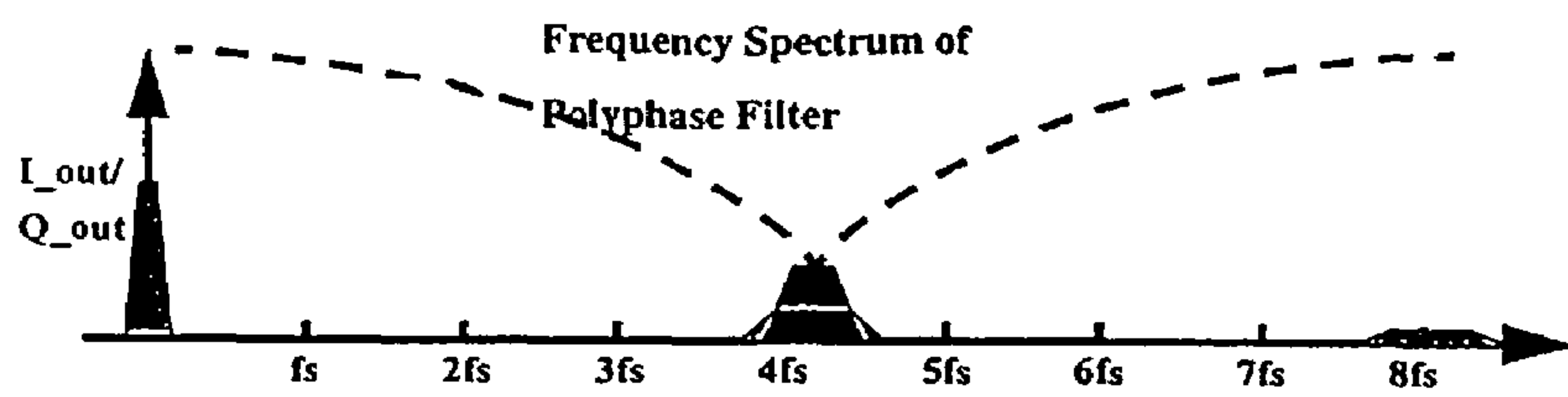
Signal Spectrum at Polyphase Input
