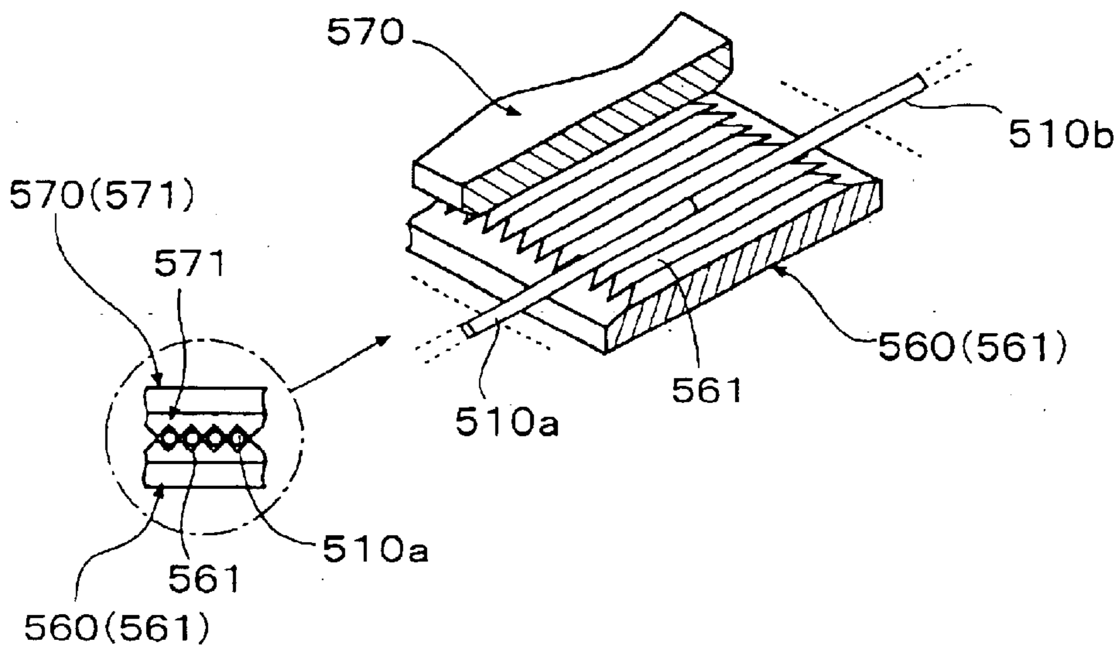
FIG. 4C PRIOR ART
