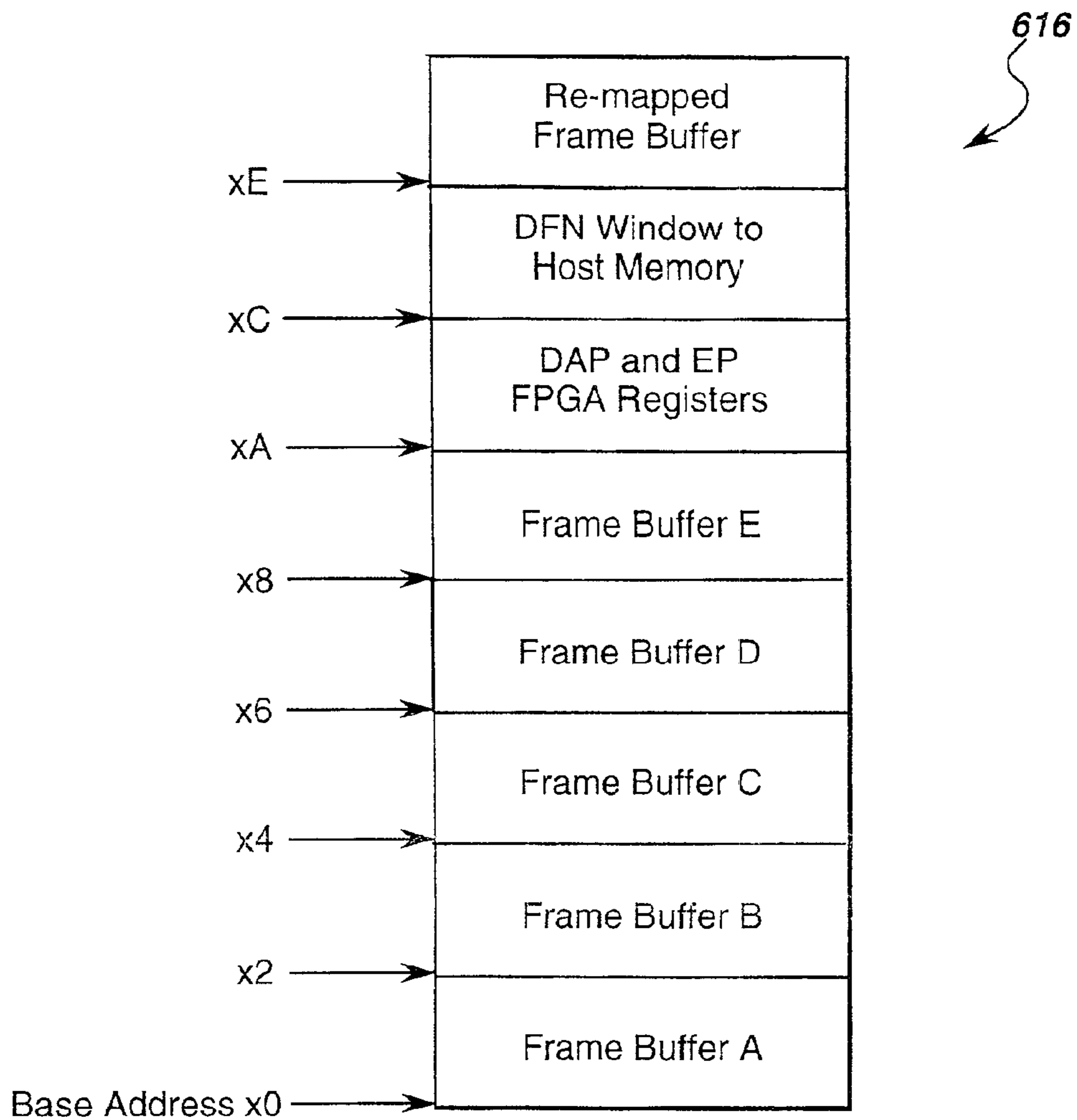
Mapping of 16 MByte PCI Address Space
