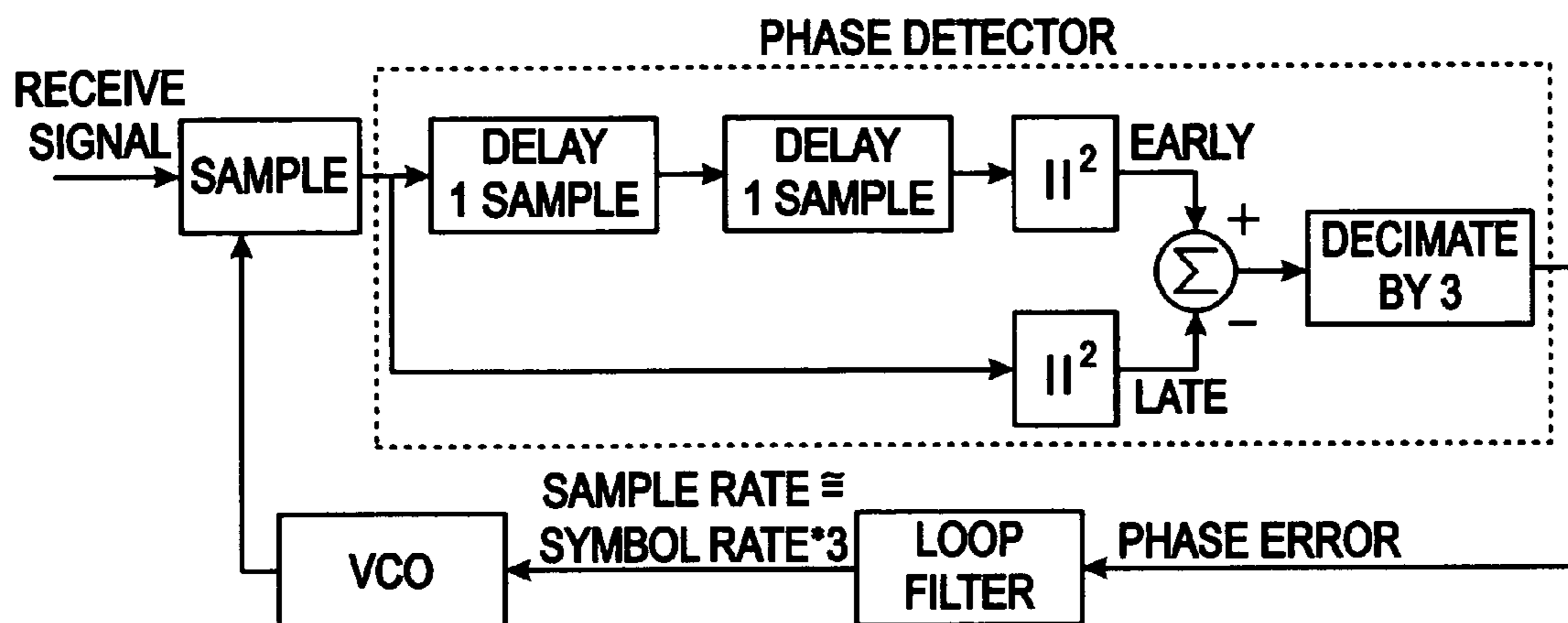
FIG. 1 (PRIOR ART)
